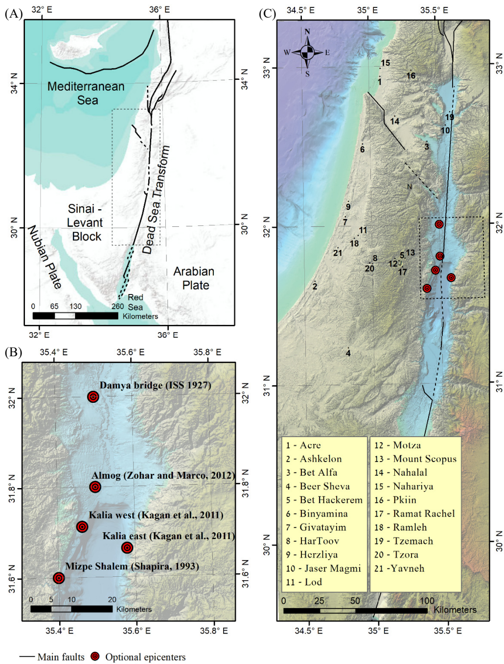
Figure 2: Research area: A) Middle East area with the main tectonic elements. B) Proposed epicenters for the 1927 earthquake event with all sites that were investigated placed over a 25m DTM image (Hall, 1996). C) Detailed location of the proposed epicenters. Also shown are sites mentioned in the text: Jerusalem (J) and Nablus (N).
