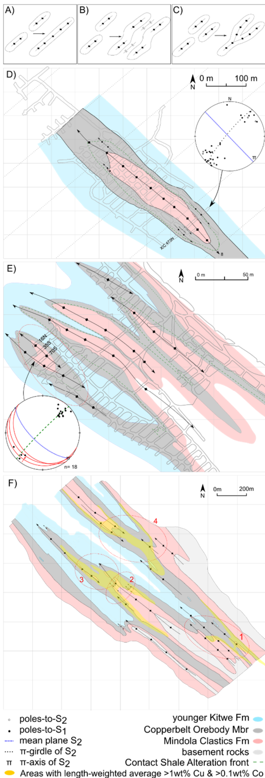
Figure 10: (a–c) Simplified illustration of concepts of fold linkage. (a) Direct fold linkage. (b) En-echelon fold linkage. (c) Bifurcation fold linkage. (d–f) Geological plans of underground levels (c. subhorizontal) and equal-area lower hemisphere stereoplots. (d) Geological map of section 7 at 3220L around 473N crosscut in Nkana South. This section intersects a doubly-plunging (periclinal) NW-SE trending 2 nd order fold geometry. Several 3 rd order parasitic folds are present along the crosscuts. Stereoplot shows measurements in 473N crosscut, with the pole-to-S 1 -cleavage plunging 8° towards the SE and axial planar S 2 cleavage. (e) Geological map of section 9 on 3140L at Nkana South. The stereoplot shows several shallow dipping reverse faults trending NW-SE (e.g. Fig. 7D). Folds are tight to isoclinally folded and the COM is often pinched out (cf. like in Fig. 9). The folds are arranged in a right stepping en-echelon system and are slightly periclinal. (f) Published geological plan by Brems et al. , (2009) of 3360L in Nkana South, at around the same position of section 8, slightly NE-wards. Areas in yellow are orebodies as defined by Brems et al. , (2009), containing >1wt% Cu and 0.1 wt% Co based on length-weighted composite assays from 186 horizontal drillholes. Interpretations of fold axial traces and patterns of geological layer boundaries show several interesting
