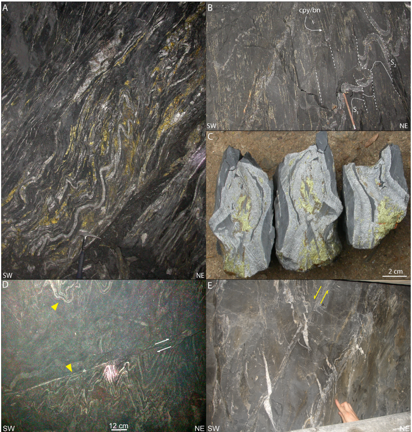
Figure 7: (a) Folded and sheared bedding-parallel veins (type I and II veins of Torremans et al., 2014). Ore mineralization consists of pyrite, chalcopyrite and bornite in the COM and in syn-folding overgrowths. Section 11, 1230S X/C. Note distinct difference in amount of sulfides between the densely veined part and the less-veined parts, suggesting that the folding of the closely spaced competent veins provides accommodation problems and transient permeability for deposition of sulfides. (b) Subvertical disjunctive S_2 cleavage affected folded fibrous bedding-parallel veins. Abundant chalcopyrite, bornite, micas and biotite are found along S_2 . Shear slickenfibres are found along some of the S_2 planes. Section 6; 910N X/C. (c) Chalcopyrite, bornite and chalcocite in fold hinges of three parallel cuts through a sample of a 4 th order folded fibrous bedding-parallel vein. The axial plane is vertical, at 89/238, with fold limbs oriented 83/238 and 84/058. Section 10; 190S X/C. (d) Low angle reverse fault in 16S crosscut (section 9) displacing folded bedding parallel veins. The fault is orientated 13/203 and mineralized by dolomite and quartz. (e) High angle normal fault with dolomite arrowhead veins in 473N crosscut at section 7 (Fig. 4). Slickenlines indicate an almost purely dip slip shear component. This fault is developed in the southern limb of a 2 nd order anticline, with the anticlinal fold hinge towards the right of the photograph.
