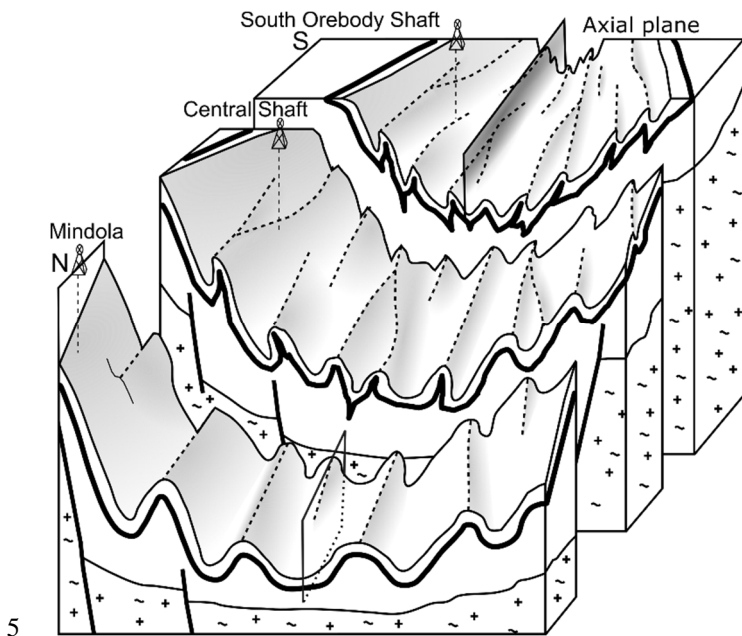
Figure 13: Interpretative schematic block diagram of the SE part of the Chambishi-Nkana Basin, showing 1 st order synclinal structure plunging 20 – 30° to the NW. Only Lower Roan Group stratigraphy is shown with the top of the Lower Roan Group exposed and the COM represented by the thick black line. Third order folds are tight to isoclinally folded in the South generally opening up towards the North. The COM at South Orebody behaves ductely and is pinched out or fault-bounded in the fold
