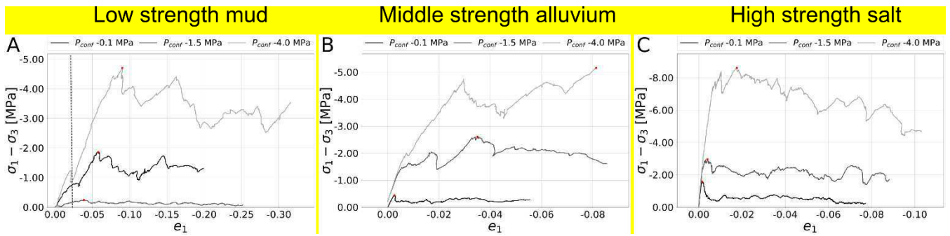
Figure 6: Differential stress versus vertical strain plots for simulated compression tests. Confining pressures of -0.1; -1.5 and -4.0 MPa are compared that highlight the depth-dependent division into elastic, yielding and post-peak behaviour in all tested materials: (A) Low strength lacustrine mud, (B) middle strength alluvial sediment and (C) high strength Holocene salt material. Black dashed line in (A) marks cut-off limit at E_{yy} = -0.02 for lacustrine mud elastic properties and peak stress estimation.
