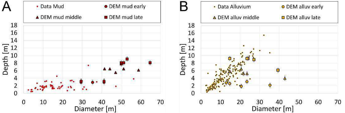
Figure 15: Sinkhole depth to diameter ratios from photogrammetry [Al-Halbouni et al., 2017] and DEM model results of this study. For field data, depth and diameter for the materials alluvium and mud were determined for 237 sinkholes. The mean values are 0.4 \pm 0.11 for sinkholes in alluvium and 0.14 \pm 0.04 for those in mud. No field data was available for salt at the time of this study. For the models, we distinguish between early collapses (circles), middle collapses (triangles) and late collapses (squares). (A) mud-flat sediments and lacustrine mud models, (B) alluvial sediments and multilayer alluvium on lacustrine mud model results.
