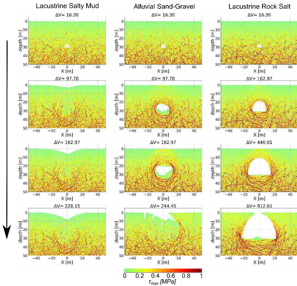
Figure 9: Evolution of maximum shear stress during cavity growth and sinkhole collapse in end-member Dead Sea materials. Shown here are selected stages in the development of cavity/sinkhole in salty-mud (left column), alluvium (middle column) and rock salt (right column). Same model setups as in Figure 8.
