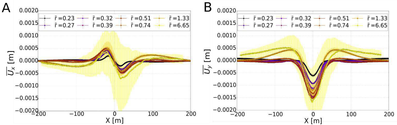
Figure 21: Results of convergence tests of for influence of particle size: Horizontal (A) and vertical displacement (B) profiles for method M1 with in a 400 x 400 m sized box. We observe a convergence of the displacement curves for mean radii around 0.32 m but for decreasing particle sizes a further diminishing of the amplitudes.
