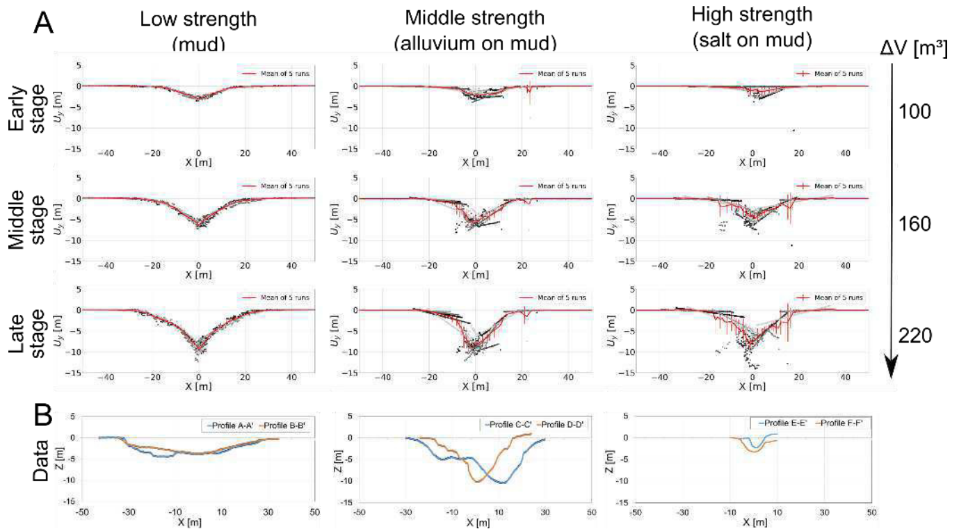
5 Figure 14: Topographic cross-sections of sinkholes in different cover materials. (A) Modelled profiles for subsrosion zones in 30 m depth and three different evolution stages. Plotted is the vertical position of the surface particles for 5 different particle assemblies of each tested model setup. Model sets are: pure lacustrine mud (left row), alluvium on mud multilayer (middle row) and salt on mud multilayer (right row). (B) Field data replotted topographic profiles of the three different sinkhole morphologies from Figure 3. The distance and altitude are normalized for better comparison with the models.
