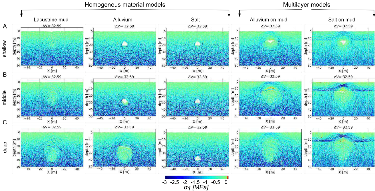
Figure 16: Maximum compressive stress for representative models after the same amount of material removal (~ 33 m 3 ). Different depths of subsion zones are compared: (A) shallow (20 m), (B) middle (30 m) and (C) deep (40m). The deeper the zone, the higher the maximum compressive stress above the created void space. The stronger the material, the more pronounced is the compression arch. Tensile stresses are observed directly above the removal zone.
