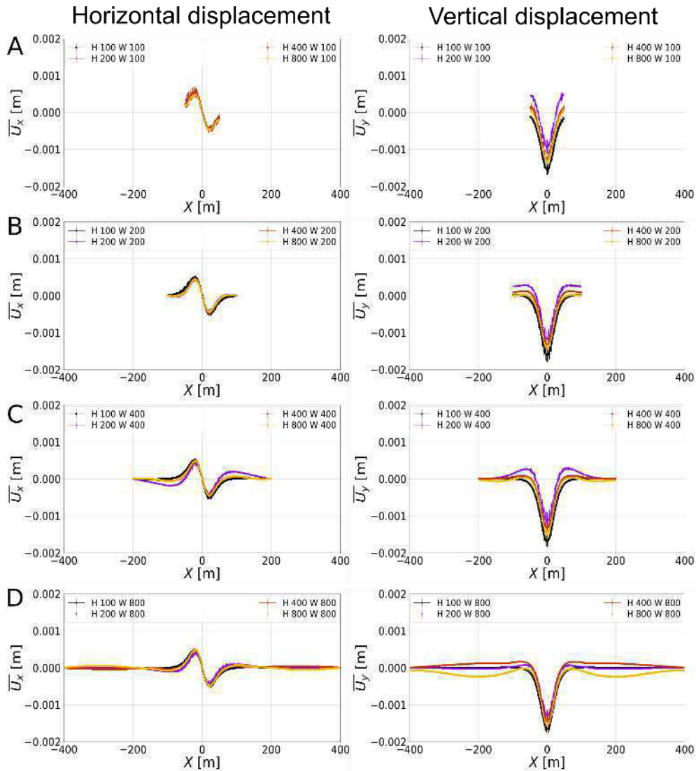
10 Figure 20: Convergence test results for model assembly dimensions: Cavity of radius = 5 m and depth = 35 m created in each case by method M1. Mean particle radius is 0.74 m. Left and right columns show horizontal and vertical displacement profiles, respectively. Each plot shows results for varying model height ( H ) from 100-800 m for a given width ( W ). In parts (A) W = 100 m;
