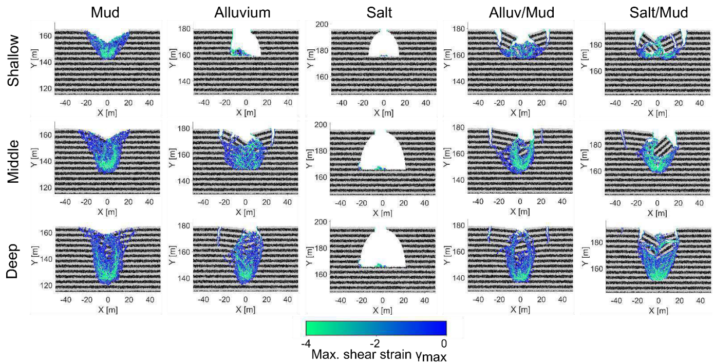
Figure 12: Sinkhole endmembers in dependency of the depth of the subrosion zone for all material combinations investigated in this study. The maximum shear strain is used to visualize the collapse zone.
