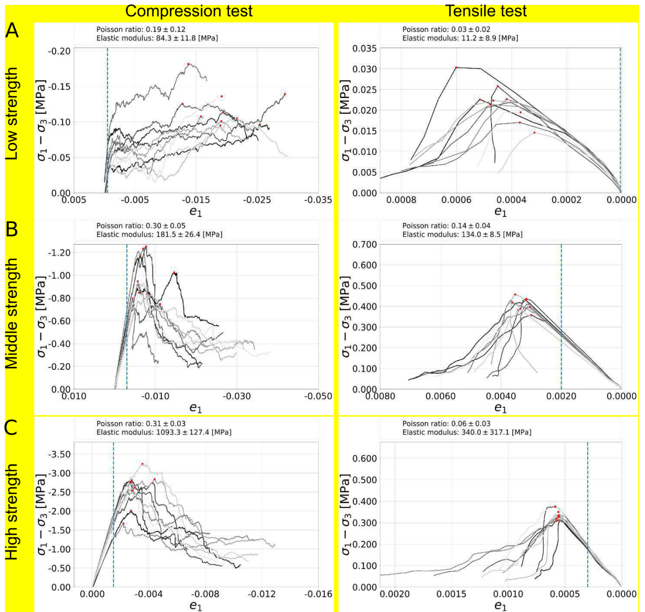
Figure 23: Differential stress vs. vertical strain for CC and DT tests for a confining pressure of 0.1 MPa. (A) Lacustrine mud; (B) Alluvium sediments; (C) Holocene salt rock. Dashed line indicates elastic limit which was used to determine elastic parameters displayed above the graphs. Red dots mark the peak stresses.
