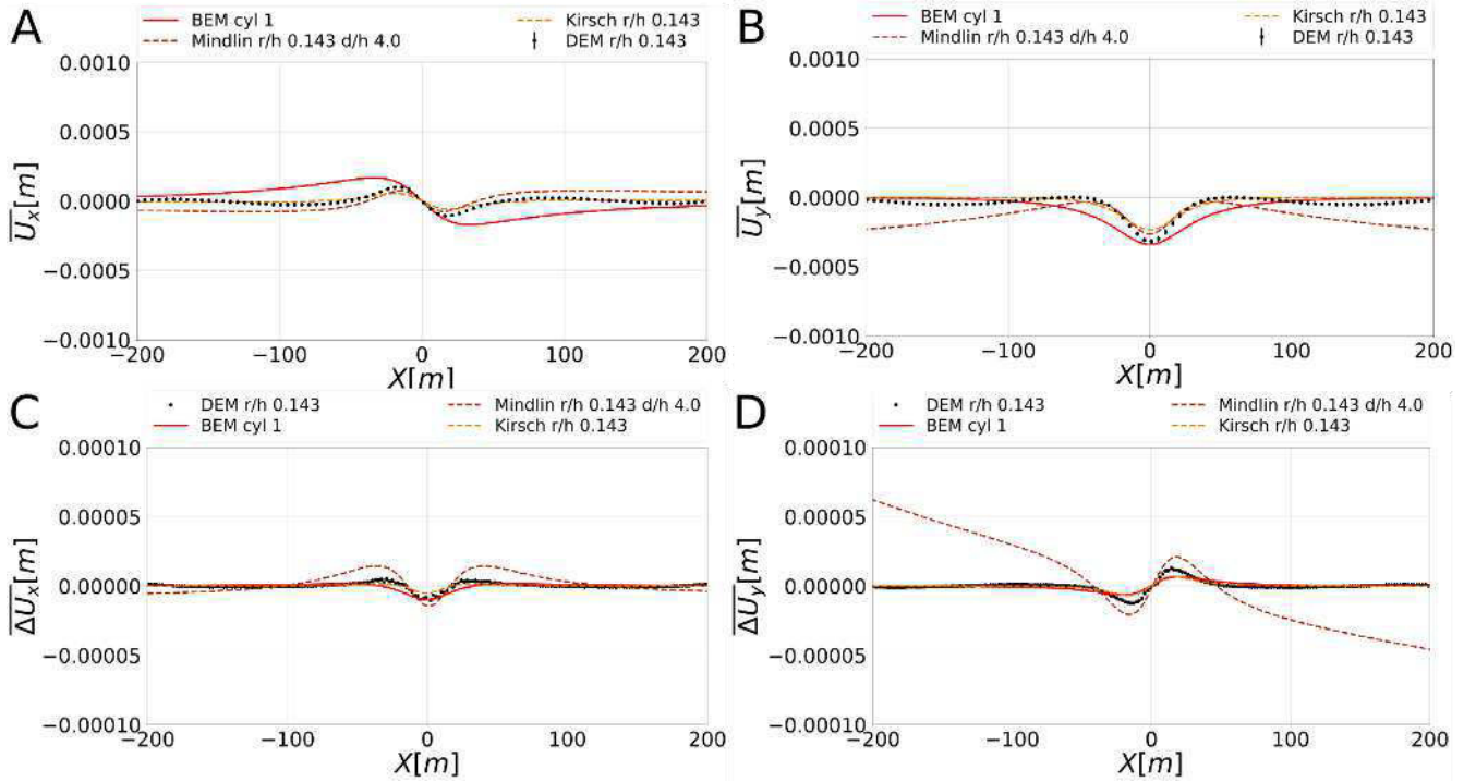
Figure 5: Results of benchmarking of the DEM cavity model against continuum-based cavity models: Analytical solutions and modelled displacement curves for model dimensions of 400 \times 400 m with particle radius 0.32 m. Reference is a cavity with r/h = 0.143 , at 35 m depth and with a 5 m radius. (A) Horizontal displacement, (B) vertical displacement, (C) horizontal displacement difference and (D) vertical displacement difference.
