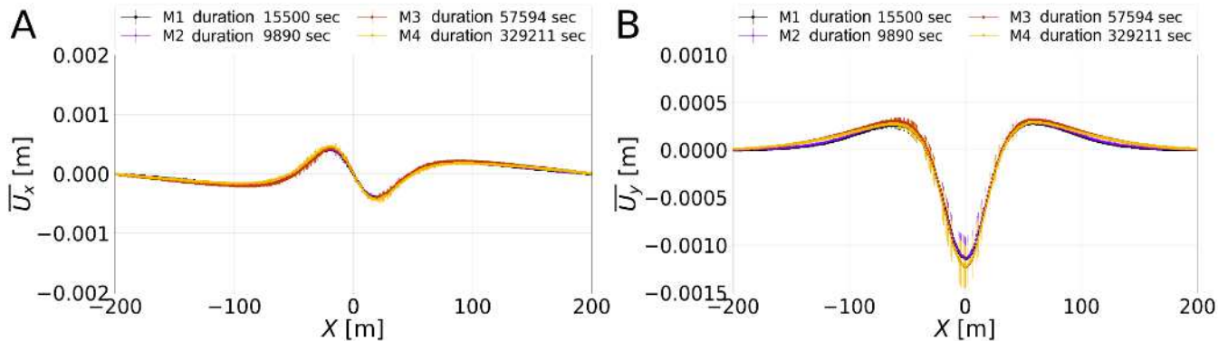
Figure 19: Displacement plots for different void installation methods. (A) Horizontal and (B) vertical model setup with size 400 x 400 m using a coarse particle distribution (mean radius 0.74 m). Indication of needed simulation time is given in the legend. M1-M4 refers to the installation method described in the text.
