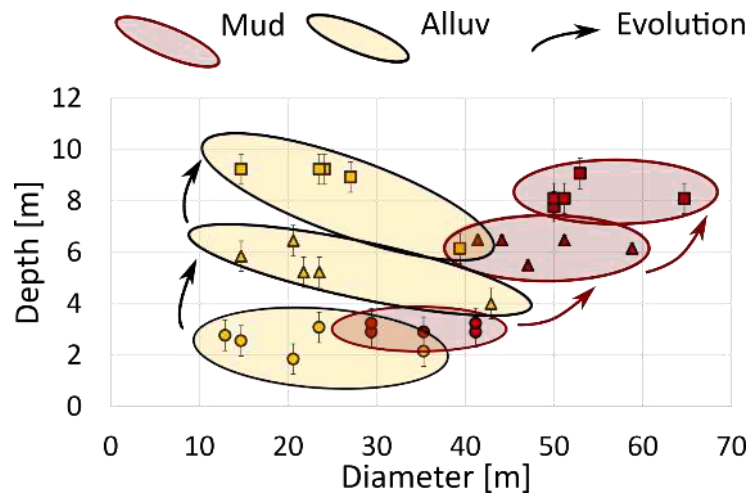
Figure 17: Simulated sinkhole depth/diameter interpretation. The simulations reveal a tendency towards deeper sinkholes in alluvium and both deeper and wider sinkholes in mud. A trend that is able to explain the observations for sinkholes at Ghor Al-Haditha.
