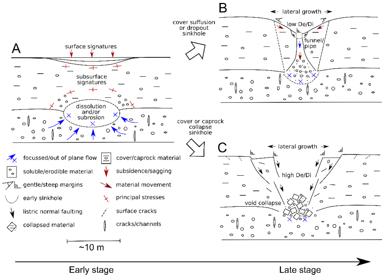
10 Figure 1: Conceptual models of sinkhole formation. (A) Sub-surface dissolution or/and subrosion caused by focussed flow in soluble/weak material. (B) Cover suffusion or dropout sinkhole that forms by material transport through a pipe or along a funnel. A weak cover material slumps into the voids and creates a sinkhole with low depth/diameter ratio and flat to steep margins depending on the material cohesion. (C) Cover or caprock collapse sinkhole. Large voids may stay initially stable in a strong material, but their growth leads to a sudden overburden collapse. The formed sinkholes have usually a high depth/diameter ratio and contain steep margins with large ground cracks. Both sinkhole types represent late stage endmembers and mixtures of both are very common in nature (Figure 2).
