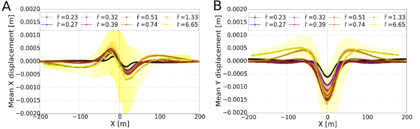
10 Figure 21: Results of convergence tests of for influence of particle size: Horizontal (A) and vertical displacement (B) profiles for method M1 with in a 400 x 400 m sized box. We observe a convergence of the displacement curves for mean radii around 0.32 m but for decreasing particle sizes a further diminishing of the amplitudes.
