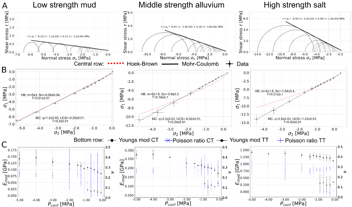
Figure 7: Bulk failure envelopes and elasticity parameters of the simulated Dead Sea materials derived from simulated laboratory tests. (A) Mohr-Coulomb failure envelopes, (B) Mohr-Coulomb and Hoek-Brown principal stress, (C) variation of elastic parameters with confining pressure. Left column: Low strength cohesive lacustrine mud, Central column: Middle strength alluvial sandy-gravel material, Right column: Higher strength Holocene salt. CT = Compression test data; TT = Tension test data.
