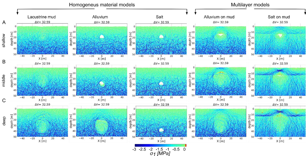
Figure 16: Maximum compressive stress for representative models after the same amount of material removal ( \sim 33 \text{ m}^3 ). Different depths of subrosion zones are compared: (A) shallow (20 m), (B) middle (30 m) and (C) deep (40m). The deeper the zone, the higher the maximum compressive stress above the created void space. The stronger the material, the more pronounced is the compression arch. Tensile stresses are observed directly above the removal zone.
