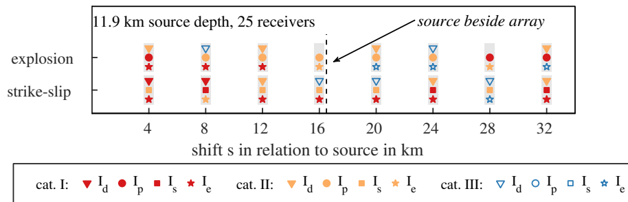
Figure 8. The quality of localizations location accuracy achieved by using 25 instead of 9 stations placed 8\text{ km} apart while shifting the array . It is marked at which shifts the array is no longer above the array. A source in 11.9\text{ km} depth was tested with two source types. The localization achieved obtained with the individual imaging conditions were ranked according to the categories from Fig. 2. Grey bars indicate setups that were tested. No symbol in the grey bar means the localization was not successful. Symbol type and colour in the grey bar represent successful localizations locations with the imaging condition sorted into the respective category.
