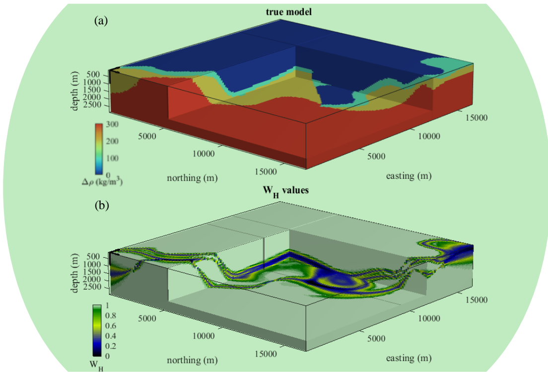
Figure 1. True density contrast model and W_H values used for local regularization conditioning. (a) Unperturbed reference model populated with density contrast values, (b) uncertainty values used for local regularization conditioning.
