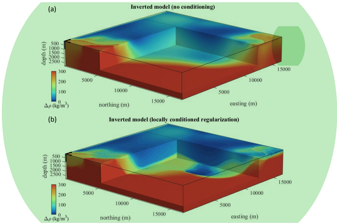
Figure 2. Comparison of inversion results. (a) Inverted models with non-conditioned regularization weights, and (b) using local conditioning.
