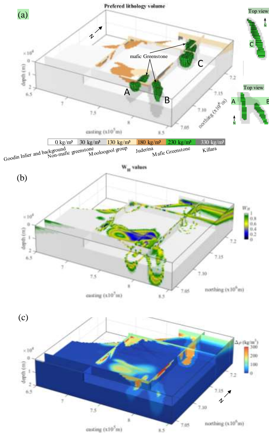
Figure 7. Geological modelling results. (a) Most probable lithology in each model cell (same colour code as in Figure 6) (b) values used for local regularization conditioning, (c) and prior model derived from PGM and prior petrophysical information). In (a), “background” refers to all the lithologies that have a density contrast equal to 0 kg.m -3 .
