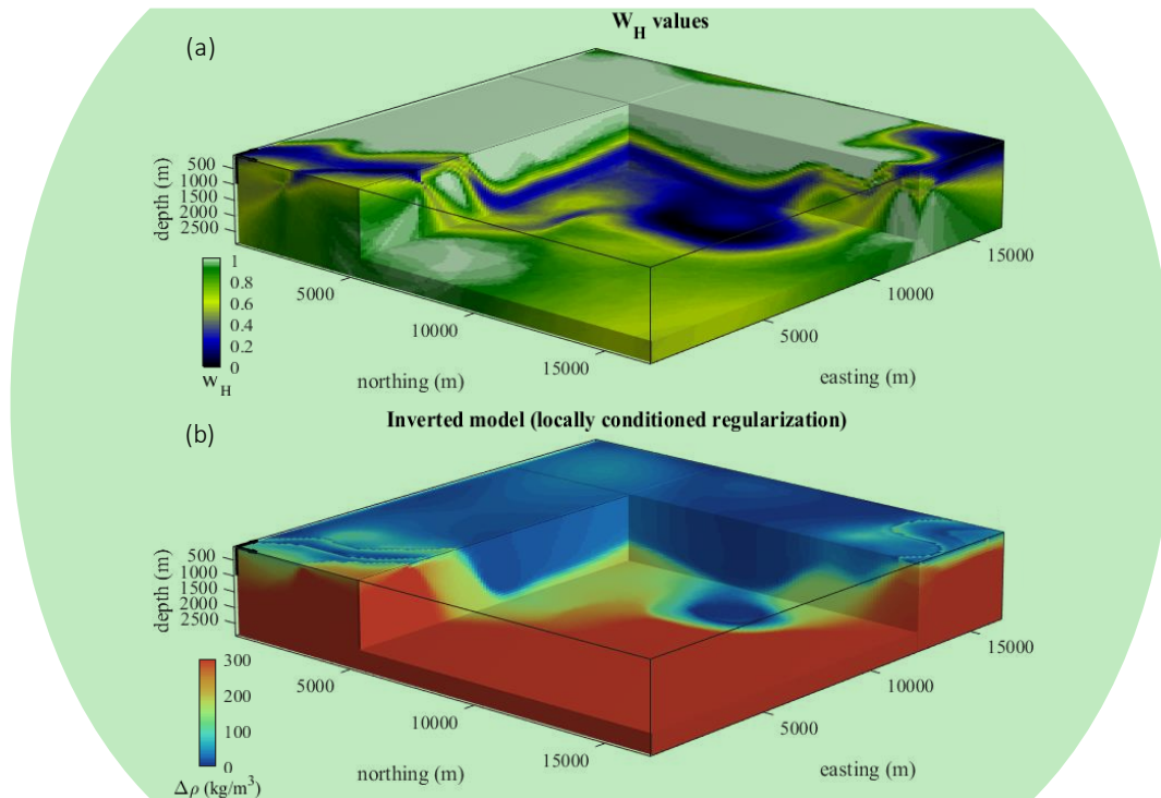
Figure 5. (a) Local weights W_H calculated from a PGM corresponding to exaggerated uncertainty in geological input measurements and (b) corresponding inverted density contrast model.
