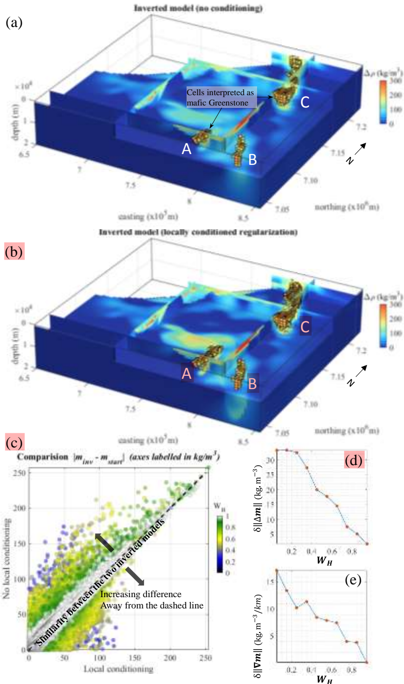
5 Figure 3. Comparison of inversion results. (a) inverted models with non-conditioned regularization weights, and (b) using local conditioning. (c) cross-plot between the corresponding absolute value of the update of the starting model, (d) difference in model updates \delta\|\Delta m\| = \|m_{cond} - m_{nocond}\|_2 as a function of values of W_H and (e) difference in model roughness \delta\|\nabla m\| = \|\nabla m_{cond}\|_2 - \|\nabla m_{nocond}\|_2 as a function of values of W_H . The model cells labelled A, B and C are interpreted as mafic greenstone belts. All voxels are coloured as a function of density contrast.
