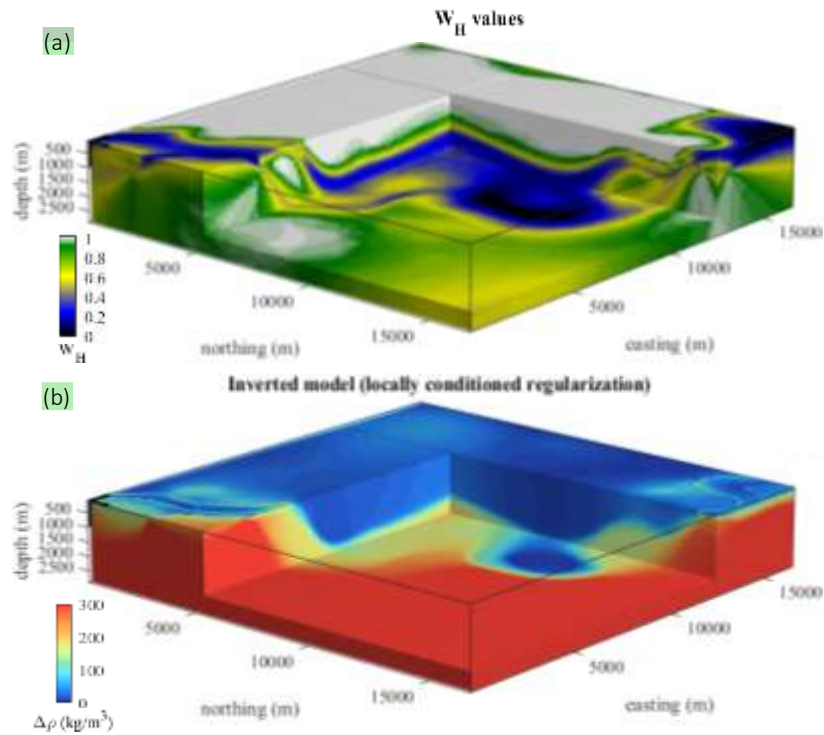
Figure 5. (a) Local weights W_H calculated from a PGM corresponding to exaggerated uncertainty in geological input measurements and (b) corresponding inverted density contrast model.
