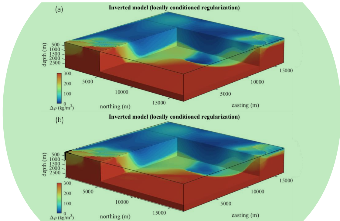
Figure 4. Comparison of inverted model using W_H derived from a PGM considering the ghost unit (b) and without it (a); (a) is the inverse model obtained without bias in the PGM as per Figure 2 and is shown here for comparison with (b).
