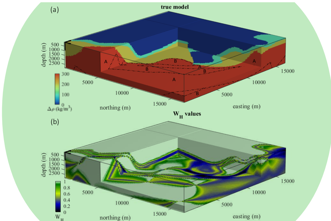
Figure 3. (a) true density contrast model with outline of the ‘ghost’ unit B (black dashed line), embedded in ultramafic unit A, and (b) local weights calculated from the PGM calculated using MCUE for model (a).
