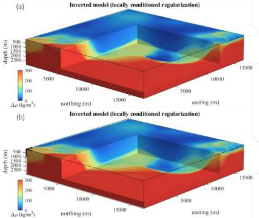
Figure 4. Comparison of inverted model using W_H derived from a PGM considering the ghost unit (b) and without it (a); (a) is the inverse model obtained without bias in the PGM as per Figure 2 and is shown here for comparison with (b).
