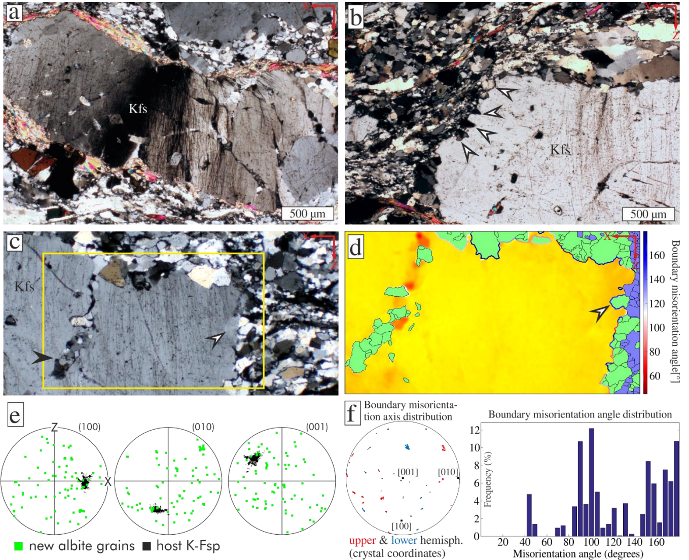
Figure 5: K-feldspar deformation microstructures (sample CT599). (a, b) Polarized light micrographs (crossed polarizers) of bent K-feldspar porphyroblast with healed microcracks parallel to the shortening direction and cusped grain boundaries (white arrows in (b)). (c) Polarized light micrograph (crossed polarizers) showing K-feldspar with fractures filled with albite (black arrow) and cusped phase boundaries. Healed microcracks are cut-off by newly formed albite (white arrow). Yellow rectangle shows area of EBSD map in (d). (d) EBSD map, where boundaries between replacing albite grains (green) and the K-feldspar-host (yellow) are colored after their misorientation angle. Quartz in the matrix is blue in color. (e) Polefigures of poles to (100), (010) and (001)
