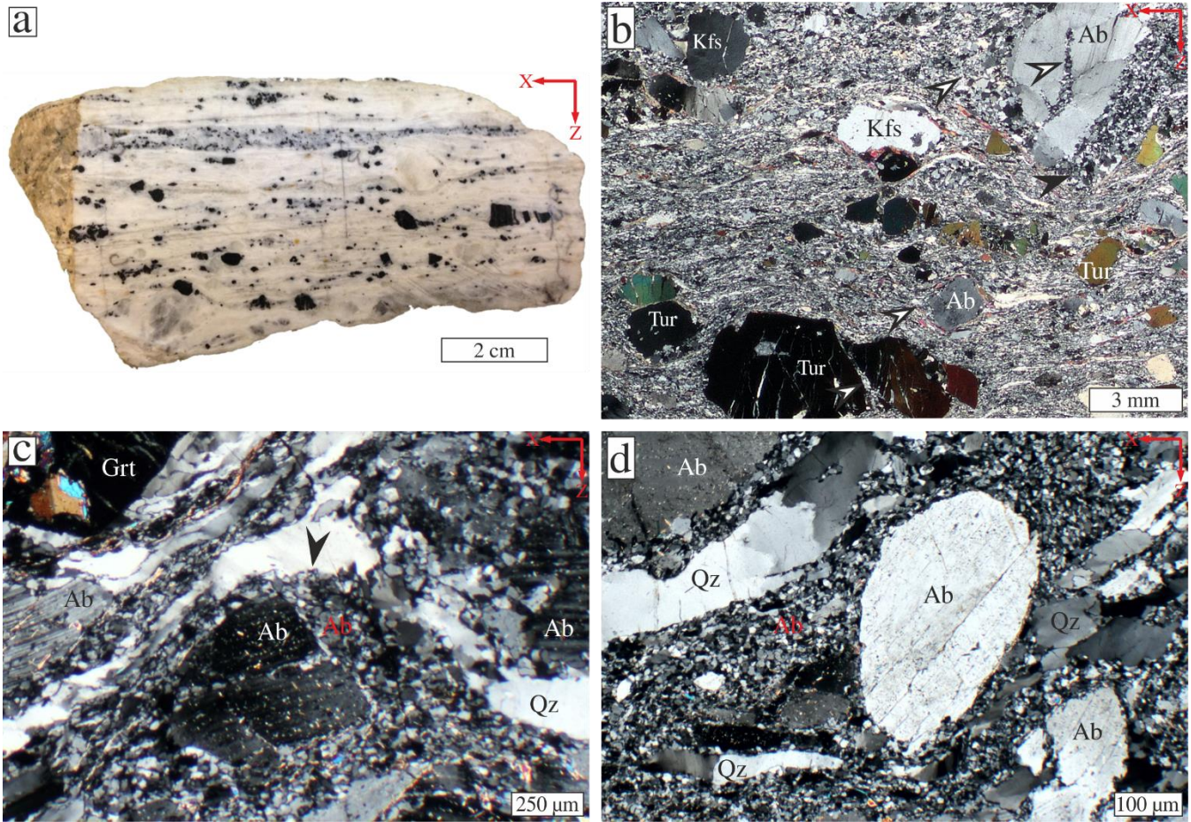
5 Figure 2: Photograph of polished surface (a) and thin section micrograph taken with crossed polarizers (b) of sample CT599. K-feldspar (Kfs), albite (Pl) and tourmaline (Tur) porphyroclasts are embedded in a fine-grained matrix. Elongate fractured tourmaline crystals are oriented with their long axes parallel to the stretching lineation (x). Fractures are commonly oriented at low angle to the shortening direction (z). Arrows point to strain shadows surrounding porphyroclast and prismatic strain shadows between fragments of tourmaline and feldspar. Black arrow points to mylonitic foliation flowing around strain shadow. (c, d) Polarized light micrographs (crossed polarizers, sample FH5b) showing mylonitic foliation defined by quartz layers (Qz) flowing around garnet (Grt) and albite porphyroclasts (Pl), which are partly disintegrated into a fine-grained albite matrix.
