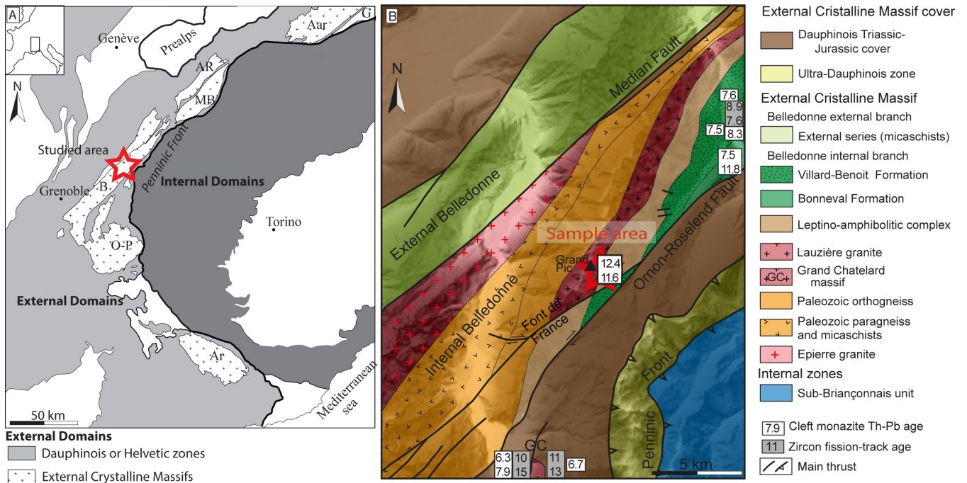
Figure 1: Simplified geological maps showing the location of the investigated area (red star). (A) Western Alps with the location of the External Crystalline Massifs: Aar; G: Gotthard; AR: Aiguilles Rouges; MB: Mont Blanc; B: Belledonne; P: Pelvoux; O: Oisans; Ar: Argentera. (B) Main geological units of the Lauzière massif. Grey rectangles are zircon fission-track central ages (Fügenschuh and Schmid, 2003), white rectangles are cleft monazite Th-Pb ages (Gasquet et al., 2010; Grand'Homme et al., 2016).
