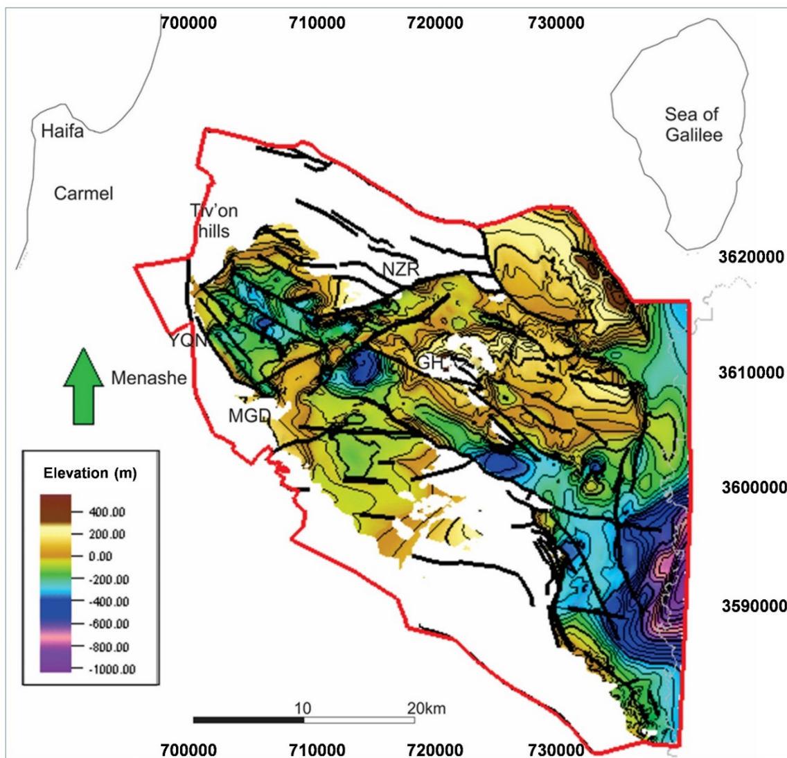
Figure 7. Structural map of the top of the Lower Basalt Formation surface. Note that the lowest areas strike NW. GH- Givat Hamore, 10 MGD- Megiddo, YQN- Yoqneam, NZR- Nazareth.
