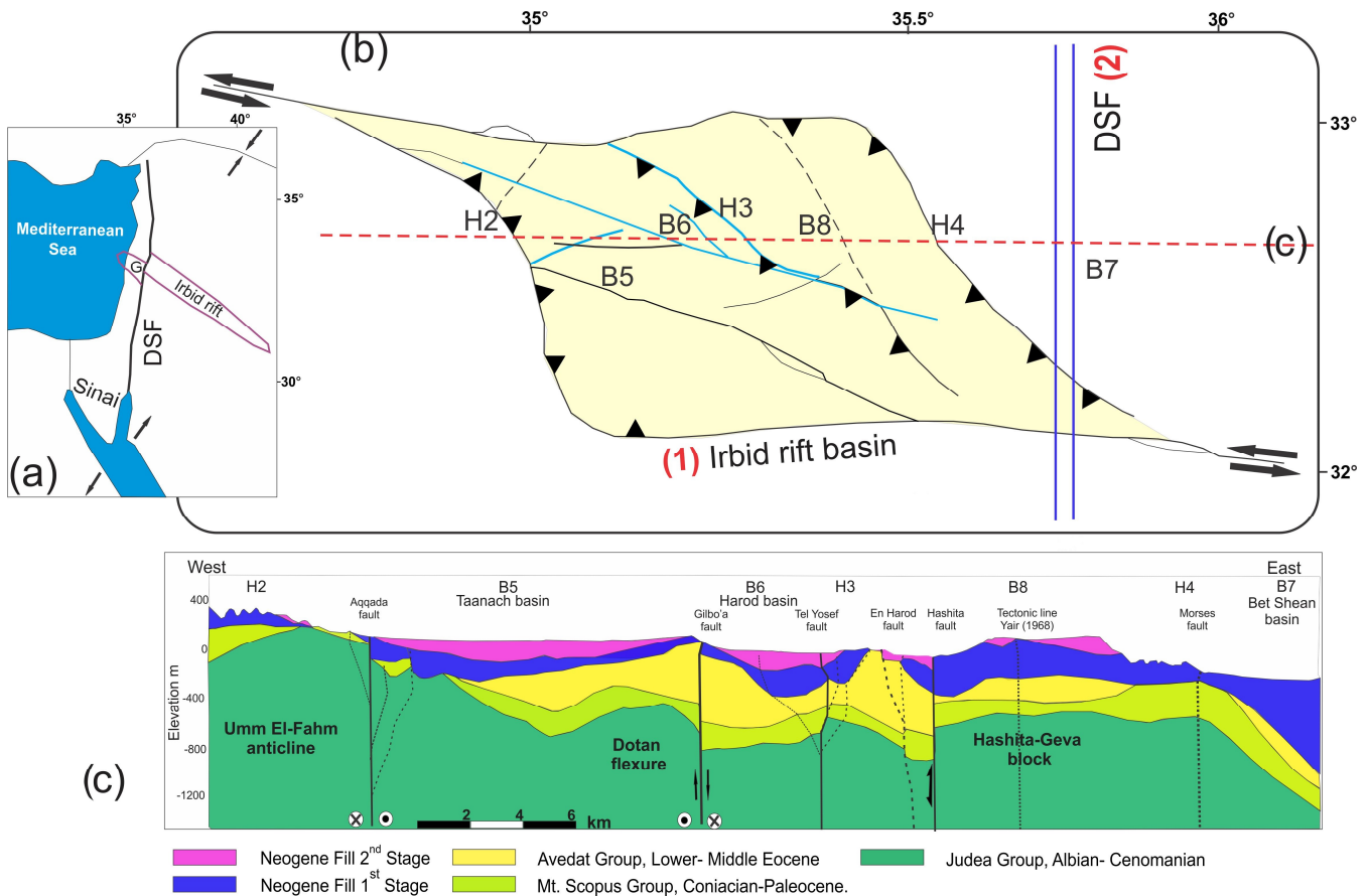
Figure 13. (a) Plan view of the northwest trending Irbit rift dissected by the Dead Sea fault plate boundary. (b) Presumed releasing jog that subsided across the Galilee above a left-lateral strike-slip Primary Deformation Zone (PDZ) during the Irbit rifting (marked as 1st stage; modified after McClay and Bonora, 2001). NNE elongation provoked extension across the interpreted normal faults (marked by celeste lines). The 2nd stage reflects the Dead Sea Fault (DSF) stress regime. (c) East-west geological cross section through basins B5, B6, B8, B7 (location in Figs. 3 and 13B). The profile is extracted from a structural model constructed for the entire study area based on seismic data, wells, and outcrops. Blue and pink shading represent the 1st and 2nd subsidence stages respectively. An inverted relief of tilted blocks is a result of a Pliocene-Pleistocene ESE compressional stress component of the Dead Sea Fault stress regime.
