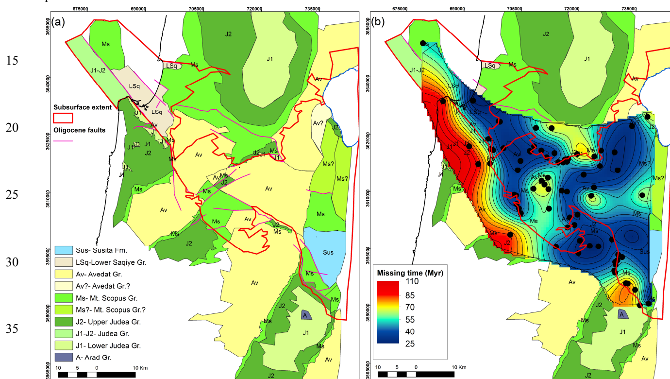
Figure 4. (a) Subcrop map of the Oligocene regional truncation surface (RTS) in UTM GWS1984 Zone 36N projection. The map shows the youngest units truncated by the RTS, based on the integrated interpretation of geological and geophysical data, from the surface and subsurface. Colors correspond to the seismic profiles. Red polygon marks the extent of data gathered in the current study. (b) Spatial variation in truncation across the Galilee represented by contours of equal time gap in million years. Black dots mark locations where the youngest unit below RTS and older unit from above are available for quantifying the time gap (see also SM6). Some of the data points are today exposed above the datum of the map. Note that some of the points may include pre-Oligocene truncations.
