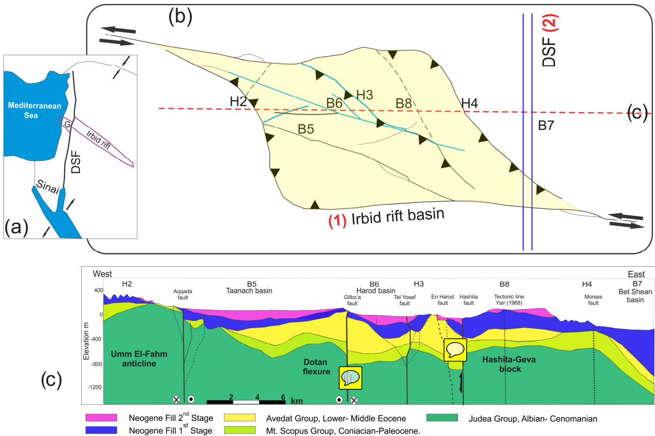
Figure 13. (a) Plan view of the northwest trending Irbit rift dissected by the Dead Sea fault plate boundary. (b) assumed releasing jog that subsided across the Galilee above a left-lateral strike-slip Primary Deformation Zone (PDZ) during the Irbit rifting (marked as 1st stage; modified after McClay and Bonora, 2001). NNE elongation provoked extension across the interpreted normal faults (marked by celeste lines). The 2nd stage reflects the Dead Sea Fault (DSF) stress regime. (c) East-west geological cross section through basins B5, B6, B8, B7 (location in Figs. 3 and 13B). The profile is extracted from a structural model constructed for the entire study area based on seismic data, wells, and outcrops. Blue and pink shading represent the 1st and 2nd subsidence stages respectively. An inverted relief of tilted blocks is a result of a Pliocene-Pleistocene ESE compressional stress component of the Dead Sea Fault stress regime.
