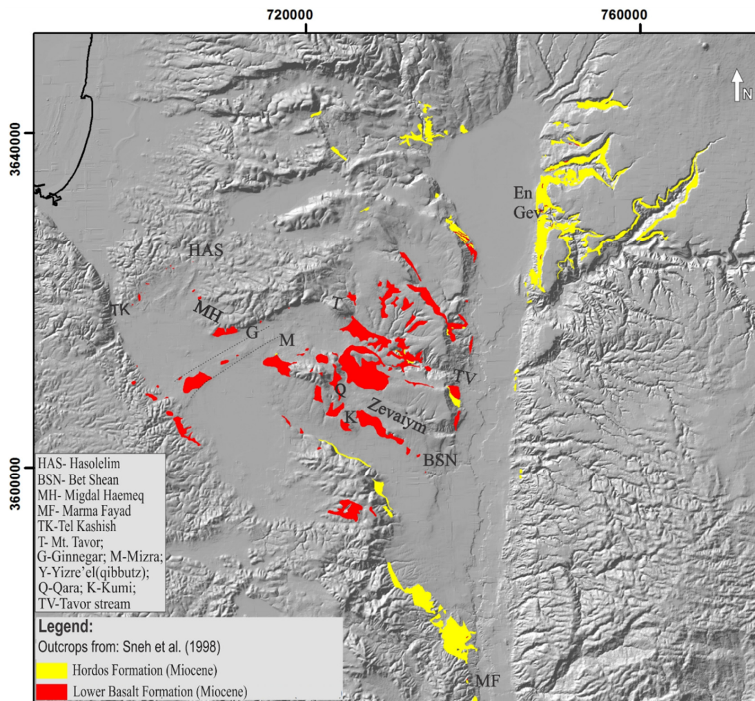
Figure 6. Location of Lower basalt Formation and Hordos Formation outcrops. The westernmost outcrop is along the eastern margins of H1 (location: Fig. 3; DEM- Sneh et al., 2000b).
