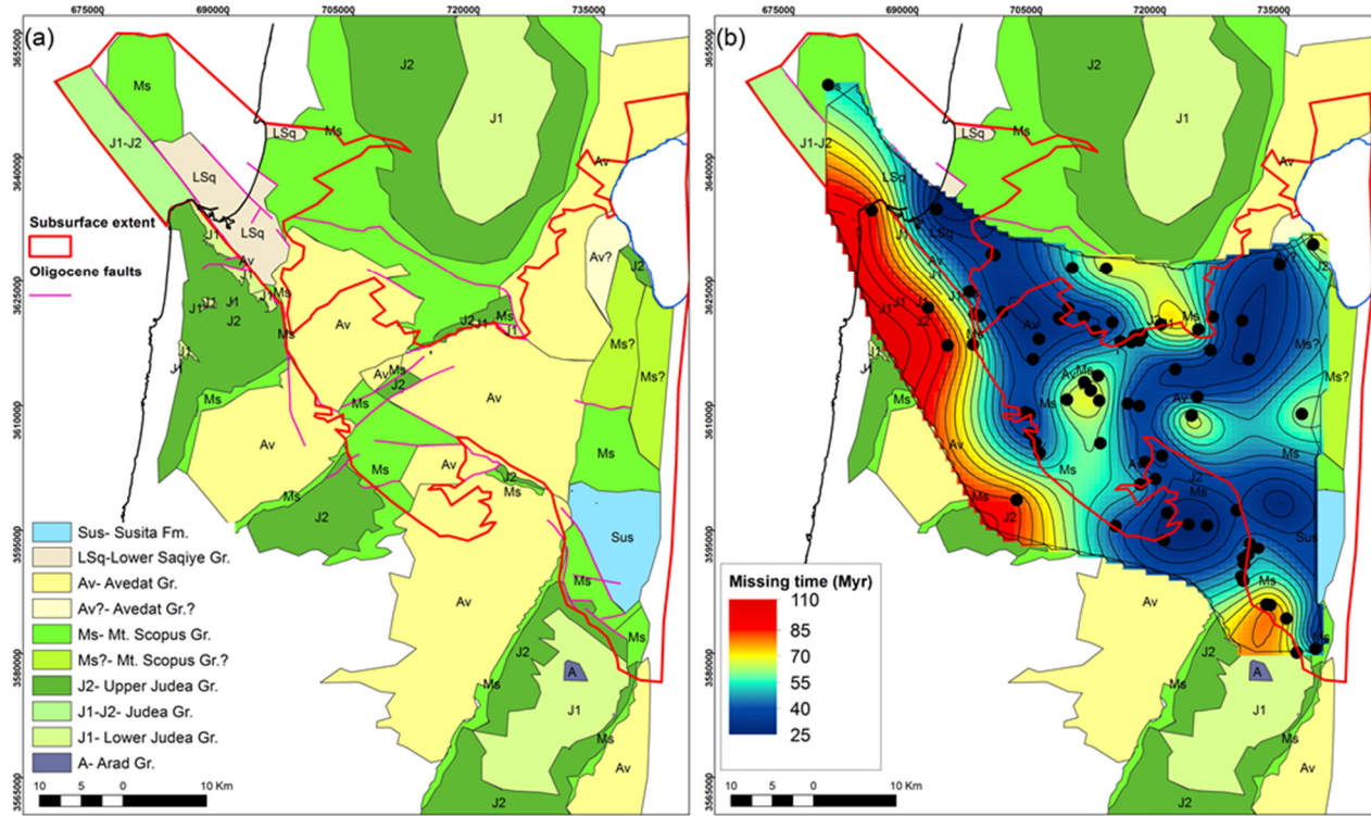
Figure 4. (a) Subcrop map of the Oligocene regional truncation surface (RTS) in UTM GWS1984 Zone 36N projection. The map shows the youngest units truncated by the RTS, based on the integrated interpretation of geological and geophysical data, from the surface and subsurface. Colors correspond to the seismic profiles. Red polygon marks the extent of data gathered in the current study. (b) Spatial variation in truncation across the Galilee is a product of kriging interpolation, further represented by contours of equal time gap in million years. Black dots mark locations where the youngest unit below RTS and older unit from above are available for quantifying the time gap (the time gap is discussed in Wald et al., under review). Some of the data points are today exposed above the datum of the map. Note that some of the points may include pre-Oligocene truncations.
