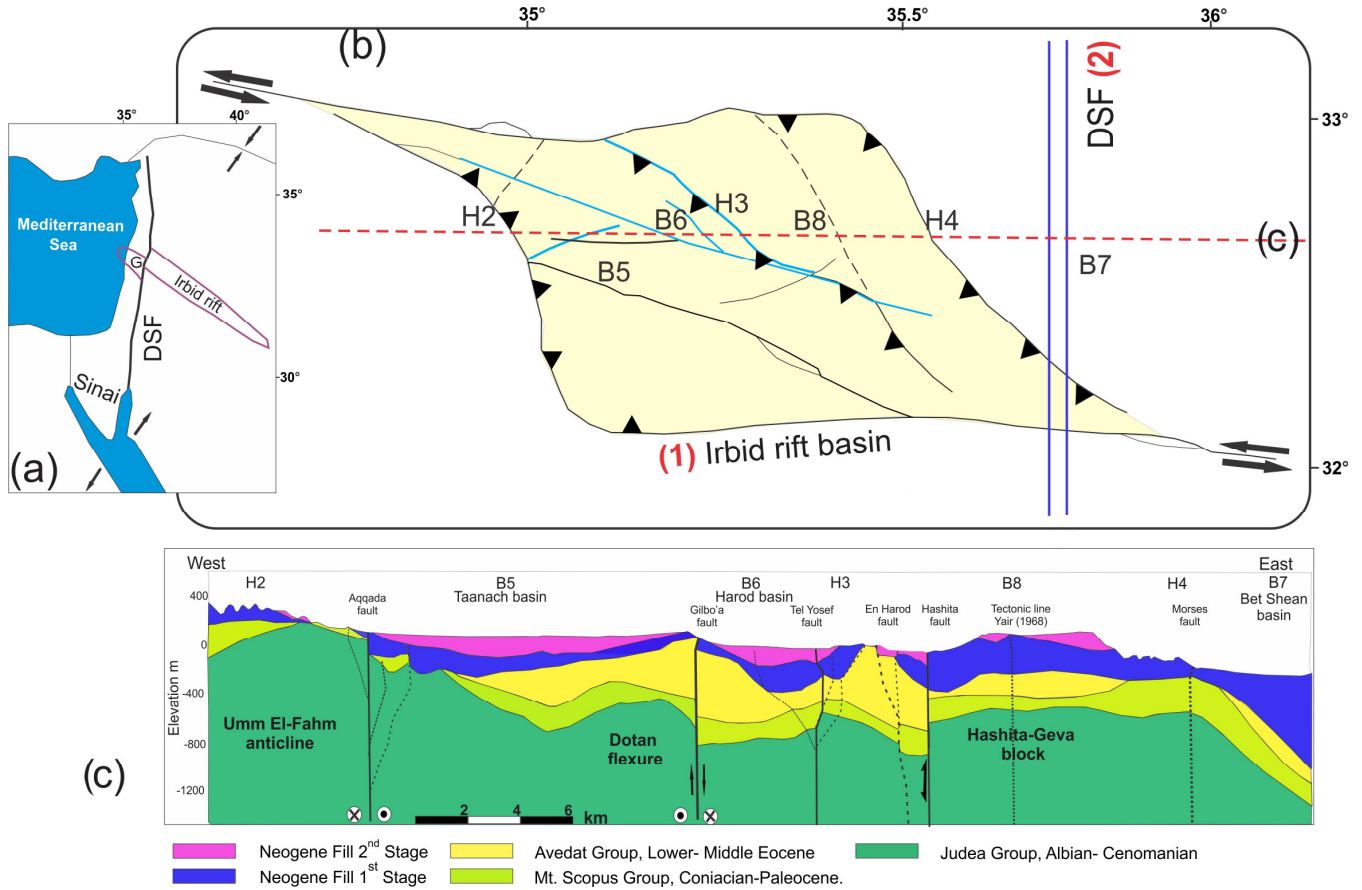
5 Figure 13. (a) Current plan view of the northwest trending Irbit rift dissected by the Dead Sea fault plate boundary. (b) Neogene basin subsidence across the Galilee during the Irbit rifting (marked as 1st stage). NNE elongation provoked extension across the interpreted normal faults (marked by celeste lines). The 2nd stage reflects the Dead Sea Fault (DSF) stress regime, during which subsidence, normal faulting and grabenization decrease while complex strike-slip faulting characterizes the strain style. An establishment of a left-lateral strike-slip Primary Deformation Zone-PDZ, modified after McClay and Bonora, 2001. (c) East-west geological cross section through basins B5, B6, B8, B7 (location: Figs. 3 and 13B). The profile is extracted from a structural model constructed for the entire study area based on seismic data, wells, and outcrops. Blue and pink shading represent the 1st and 2nd subsidence stages respectively. An inverted relief of tilted blocks is a result of a Pliocene-Pleistocene ESE compressional stress component of the Dead Sea Fault stress regime.
