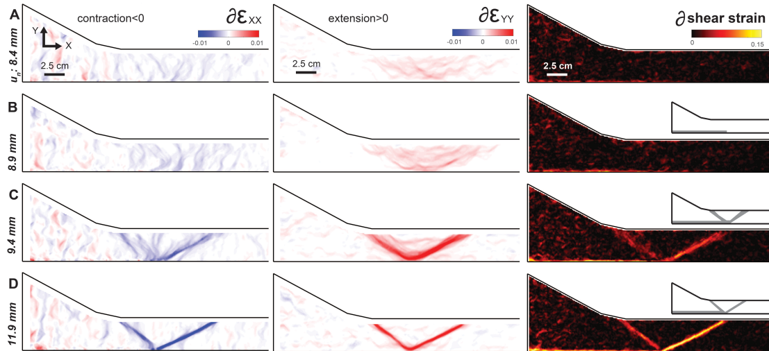
80 Figure 7: Evolution of strain as the thrust faults develop in experiment E375. Gray regions in sketches in right column indicate portion of strain field that contributes to \delta W_{\text{fric}} , and the remaining white area contributes to \delta W_{\text{int}} . A) Preceding thrust faulting, the wedge had distributed high horizontal and vertical normal strains. B) With continued backwall displacement, horizontal contraction and vertical extension shifted toward the region where the thrusts ultimately develop. C) In the incipient stages of thrust development, horizontal contraction and vertical extension formed broad bands of high strain a few centimeters thick, and shear strain began to localize along both thrusts. At this stage, and in subsequent increments, the forethrust produced higher shear strain than the backthrust. D) The zones of high horizontal contraction, vertical extension and shear strain localized into discrete zones of higher incremental strains along the thrusts. The progressively localizing normal and shear strains produced the gradually increasing and decreasing \delta W_{\text{int}} coincident with fault development. Preceding fault development, the distributed strains produced maxima values of \delta W_{\text{int}} . As strain localizes onto faults, \delta W_{\text{int}} decreased to near zero, while \delta W_{\text{fric}} increased. 85
