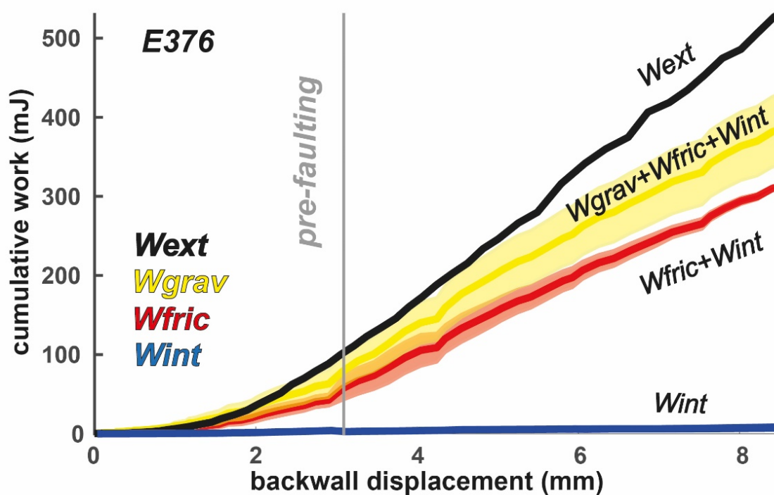
90 Figure 8: Total accumulation of work done throughout experiment E376. Upper black line shows total W_{ext} . Thicker lines show accumulation of work components calculated from average of the left and right displacement fields. Upper and lower edges of shaded regions show work accumulation calculated from left and right side views, respectively.
