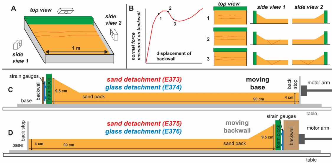
10 Figure 1: Schematics of experimental setup, force and faulting evolution. A) Position of cameras relative to sandpack. Backwall and glass sidewalls are in green and gray. B) Characteristic force curve and faulting events revealed through the top and side views. C-D) Experiment apparatus configurations of each experiment. The four experiments differ in the apparatus configuration: C) moving base (E373, E374) or D) moving backwall (E375, E376), and the inclusion of basal glass bead layer.
