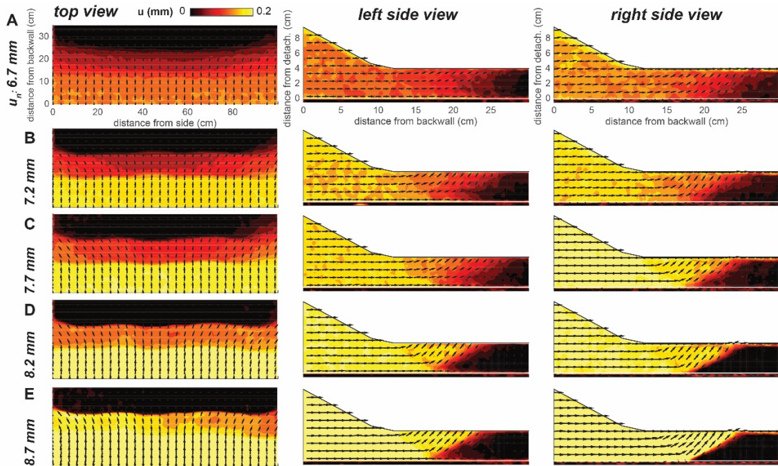
15 Figure 2: Incremental displacement fields of top and side views of experiment E374 (glass detachment and moving base) throughout the development of the first thrust pair at 0.5 mm increments of applied backwall displacement, u_n . A) Preceding thrust fault development, the net displacement gradually decreases from the backwall toward the opposite wall. B) When sharp gradients in the top view displacement field revealed the development of the first thrust pair within the center of the box, the side view displacement fields showed more diffuse zones of shear. C-E) With continued backwall displacement, the gradients in the top and side view displacement fields progressively sharpened as faults localize. The top view displacement fields reveal that the thrusts began to localize within the center of the sandpack, and then extended toward the sidewalls. The side view displacement fields indicate that fault localization began earlier on the right side than the left side in this experiment (C). The forethrust remained more diffuse on the left side view than the right side view in the last increment shown here (E). 20
