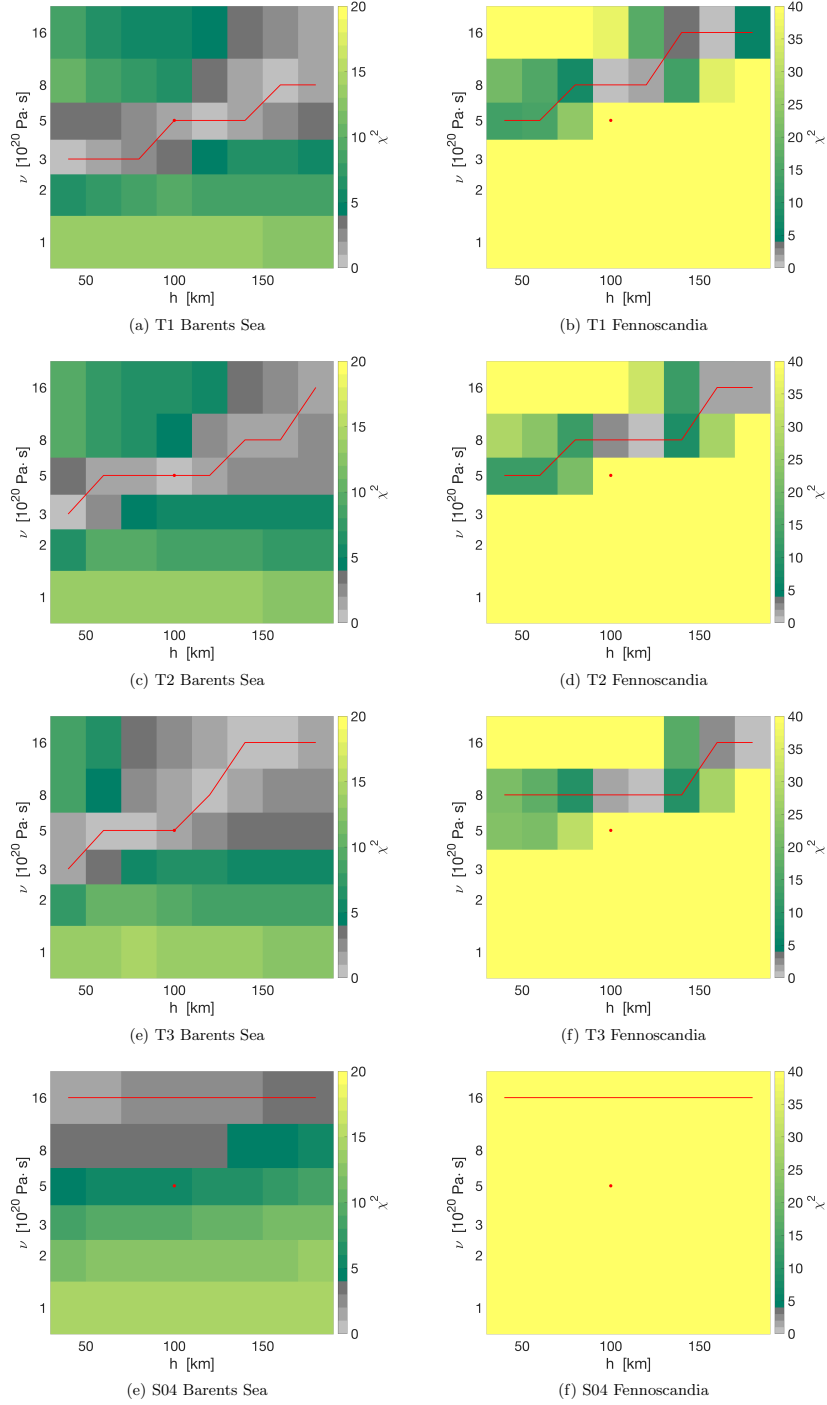
Figure 6. Misfit of the T1,T2,T3 and S04 ice deglaciation chronologies to GRACE observations for different values of upper mantle viscosity ( \nu ) and lithospheric thickness ( h ) in the Barents Sea (left column) and Fennoscandia (right column). The fit is given in terms of the \Delta\chi^2 . The circle indicates the reference model and the red line shows the best fitting model for each lithospheric thickness
