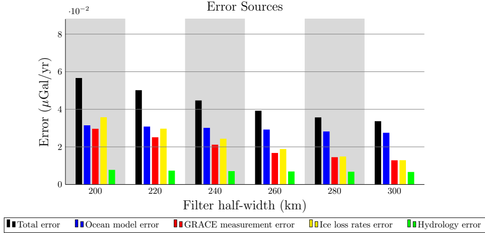
Figure 4. Error in \mu\text{Gal}/\text{yr} in the maximum gravity rate in the central Barents Sea from different sources. The magnitude of the error is given for different low-pass filter half widths and a high-pass filter half width of 600 km.
