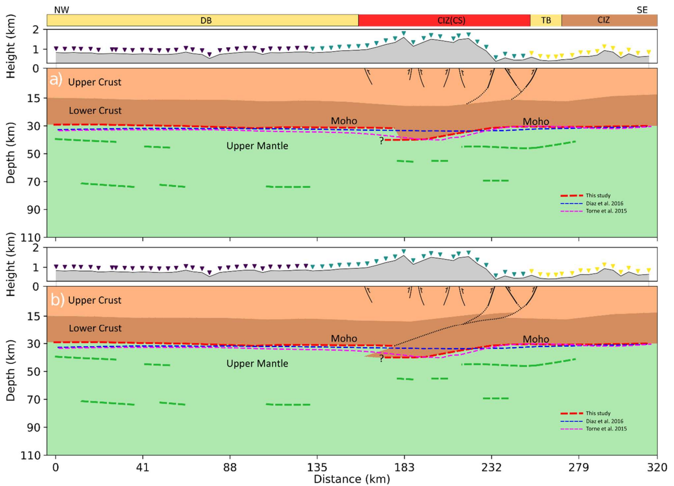
Figure. 6 Sketch of the proposed crustal geometry, overlapped with Moho results from gravity inversion and RF. a) model where the S thrust and the Tietar fault lie within the upper crust and only the lower crust imbricates; b) model where the entire crust imbricates below the CS
