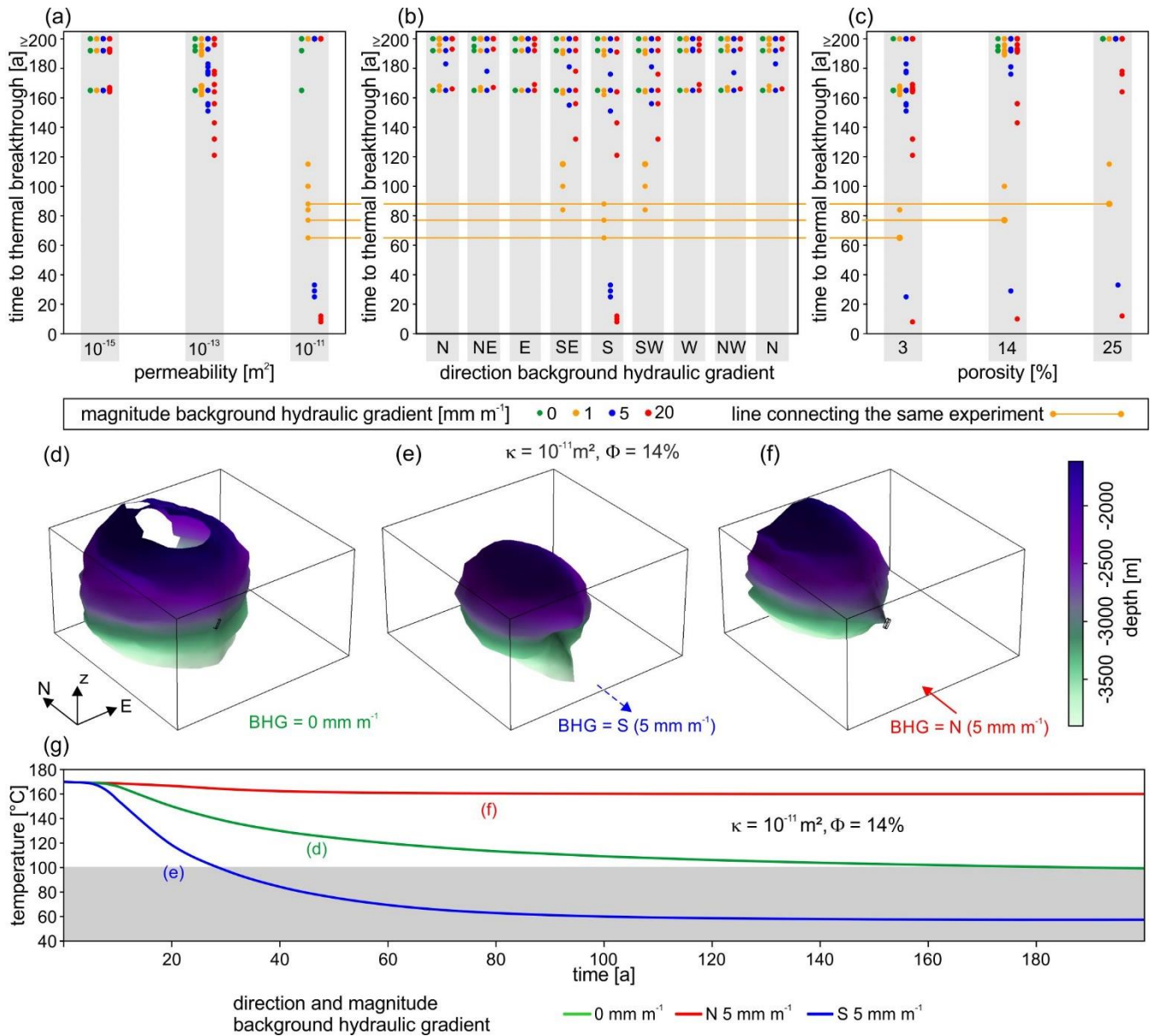
785 Fig. 2: Parameter values against time to thermal breakthrough for model experiments with homogenous and isotropic structure (Scenario 1). Plots (a), (b), and (c) each contain the same results of 225 simulations, but are arranged according different x-axes. The results show that with increasing permeability, the BHG becomes the prime factor that determines time to thermal breakthrough, while the effect of porosity is minor. Plots (d), (e), and (f) show the shape of the HDI after 100 years for a model with a permeability of 10 -11 m 2 and porosity of 14%, with no BHG (d), with a BHG of 5 mm m -1 to the S (e), and with a BHG of 5 mm m -1 to the N (f). At high permeabilities and magnitudes of the BHG, the shape of the HDI becomes ellipsoidal. Panel (g) shows the development of the production temperature over time for the models presented in (d-f). 790
