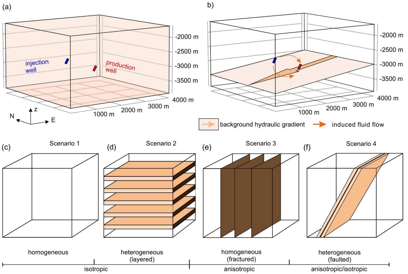
775 Fig. 1. Model setup used in our study. (a) the rectangular cuboid model lies at a depth between 1600 and 3900 m and has side lengths of 4000 m. Injection- and production wells are 1500 m apart. (b) shows one example of an westward directed BHG. (c–f) show sketches of the different scenarios investigated, comprising of reservoirs that are (c) homogenous, (d) horizontally layered, (e) include vertical fracture anisotropy, and (f) a 60° west-dipping fault zone that consists of a damage zone, with and without a fault core, and with and without fracture anisotropy in the damage zone. Modified after Bauer (2018). 780
