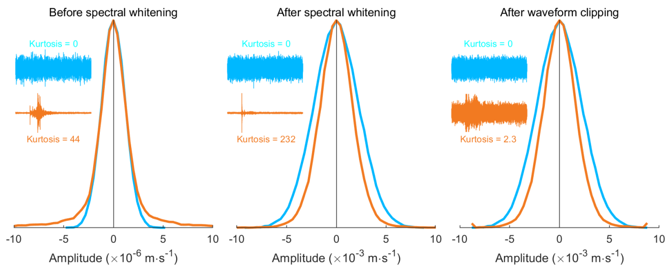
Figure 3: Kurtosis-based selection filter to determine if a segment contains large-amplitude transients. The two segments used here are the same as in Fig. 2. For display, waveforms are plotted in varying scales. The amplitude histograms are normalized by their own maximums. Histogram tails outside the horizontal axis limits are cropped.
