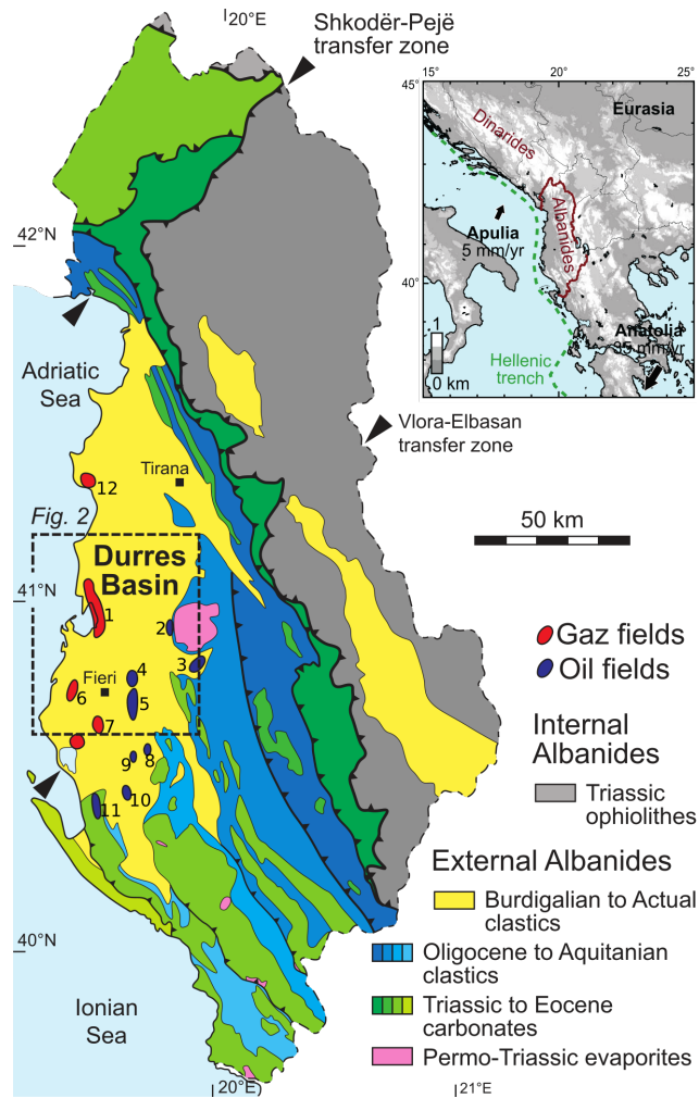
Figure 1. Simplified geological map of Albania. Oil and gas main fields are indicated in blue and red, respectively and numbered : 1-Ballaj-Divjaka, 2-Pekishti, 3-Kucova, 4-Bubullima, 5- Patos-Marinza, 6-Seman-Poveica, 7-Frakula, 8-Balshi, 9-Cakrani, 10-Gorishti-Koculi, 11-Drashovice, 12-Durrresi. Dashed rectangle is the study area as plotted in Fig. 2. Upper right inset shows the geographical location of Albania and regional kinematics with respect to stable Eurasia (Métois et al., 2015).
