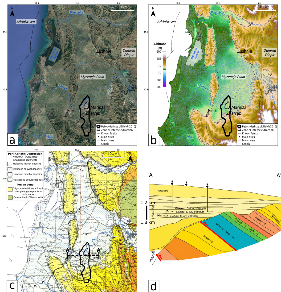
Figure 2. Anthropogenic, hydrological and geological context of the study area. The Patos-Marinzë active oil-field (black bold line) is contoured based on BCP, 2015. It encompasses the zone where wells are the densest and extraction activity concentrates (thin black line). Faults (black dashed lines) are from Aliaj et al. (2000). a-Optical satellite image of the southern part of the Durres Basin in the Fieri prefecture (satellite images from the Google Earth data base). b-Hydrology of the Myzeqeja plain. The network of man-made canals (in blue) is from TPGINC and is superimposed to the topography of the area (Farr and Kobrick, 2000). c-Extract of the Geological Map of Albania (simplified from Xhomo et al., 2002). The dotted bold line is the approximate position of the simplified geological transect presented in the panel d. d-West-East interpreted geological cross-section modified from Silo et al. (2013). The average depth of the Messinian sandstones oil-bearing formations drilled in the northern part of the Patos-Marinzë oil field is indicated together with the associated depositional environments. Faults in the underlying sedimentary series are plotted in red.
