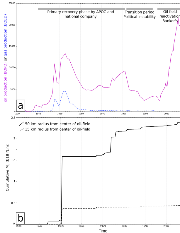
Figure 3. a- History of production of oil (plain line in Barrel Oil per Day) and gas (dashed line, in Barrel Oil Equivalent per Day) in the Patos-Marinza field (BCP, 2015; IHS, 2019). b- Cumulative seismic moment released since 1939 based on a combined USGS-EMSC catalog (USGS; CSEM-EMSC, before and after 2004, respectively) over a 50 km radius area (plain line) and a 15 km radius area around the oil field (dashed line). The contours of these zones are plotted in figure 5.
