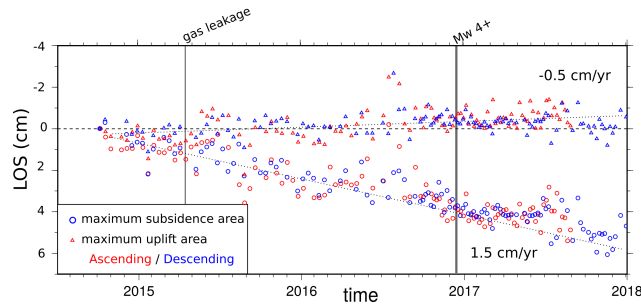
Figure 7. Displacement time-series for the most subsiding and uplifting areas (3x3 pixels) on both tracks (ascending is red, descending is blue) in the Patos-Marinza oil field, relative to a stable area. The average trend is indicated (dashed line), together with two particular events (grey vertical bars) related to the field exploitation and seismic activity.
