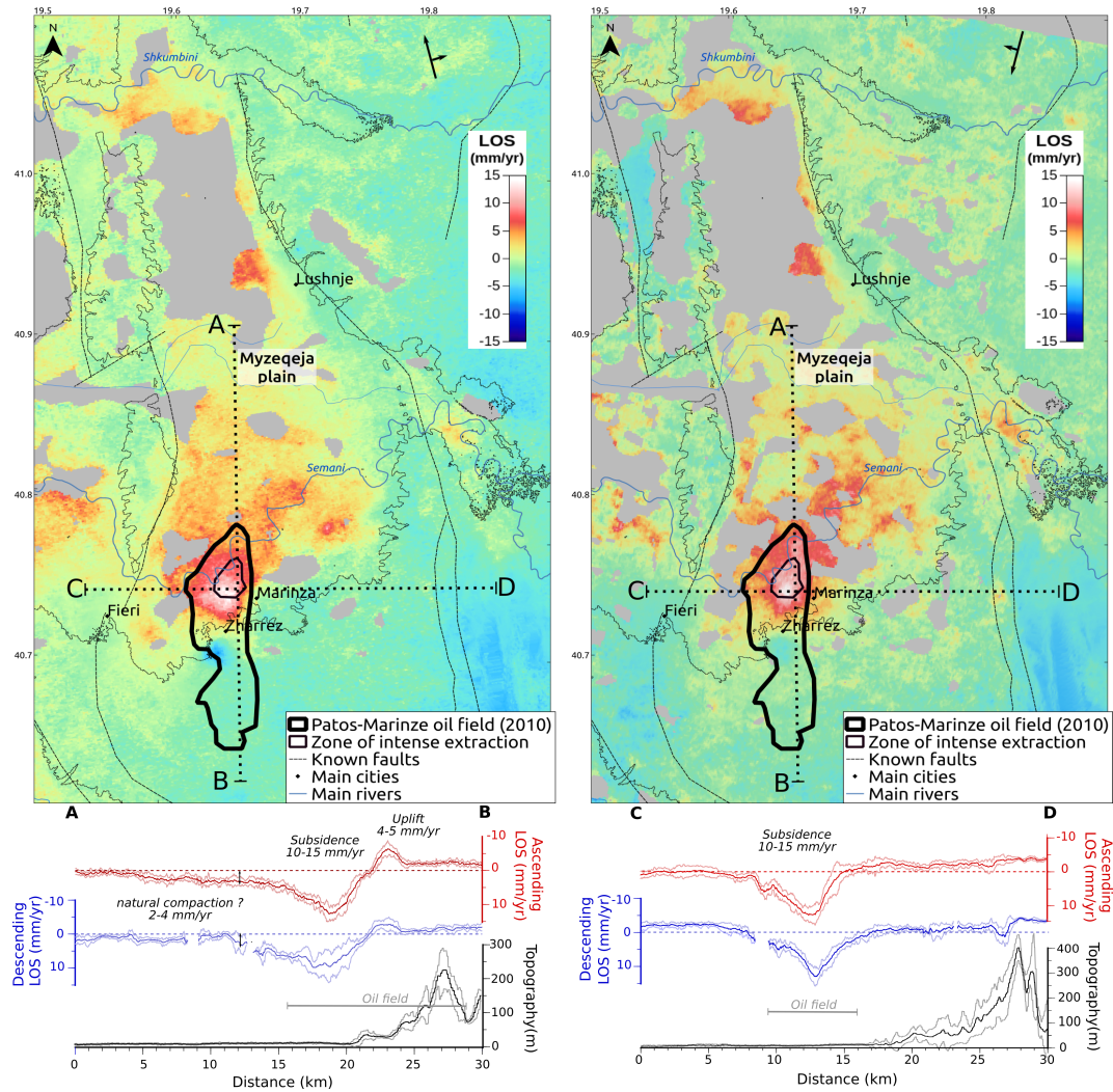
Figure 6. Top: Zoom on the LOS average velocity map for the ascending (left) and descending (right) tracks over the Patos-Marinza oil field. Color code and sign convention are the same as in Figure 5. Dotted lines indicate the location of the profiles at bottom. Bottom: north-south (left) and west-east (right) velocity profiles across the oil field's most intense deformation zone together with topography profiles (bottom). Average values over a 2 km width across the profile lines is plotted darker, while lighter lines limit the 2\sigma standard deviation envelop.
