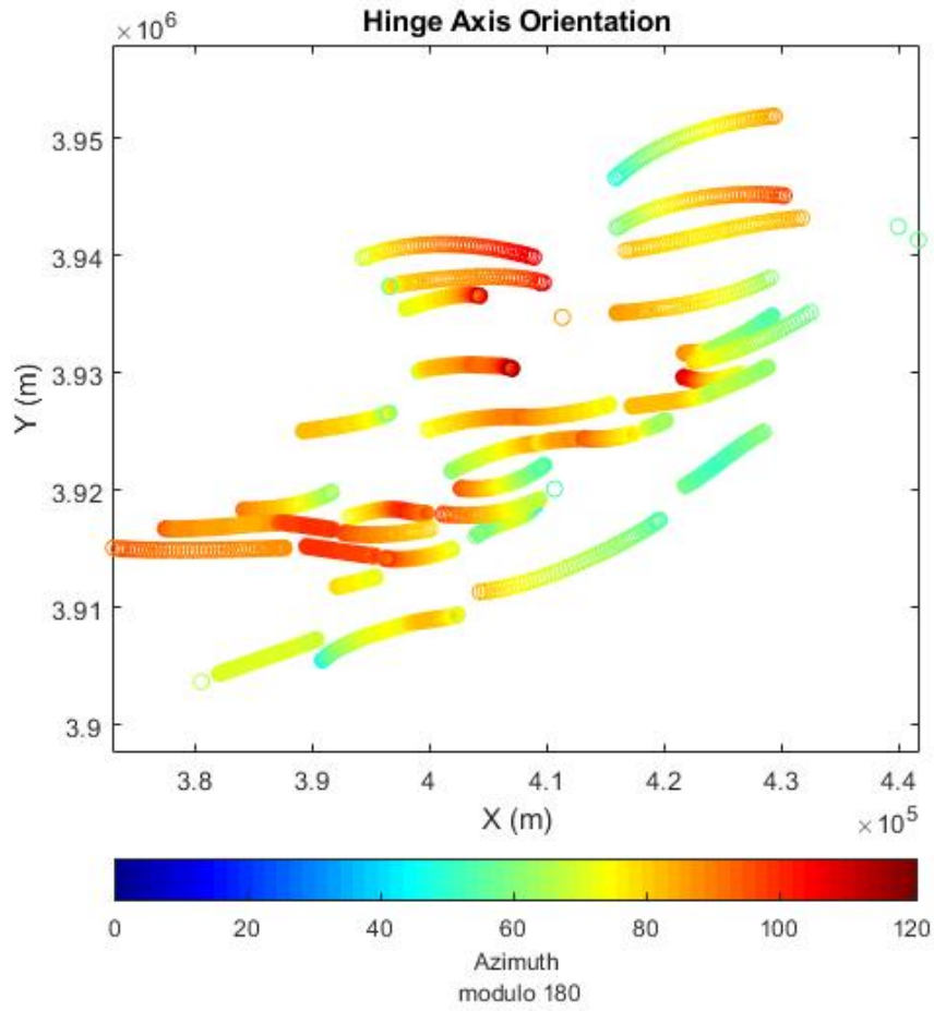
Figure 1: Azimuths of the hinge axis of the folds along the SAR area. Azimuths tend toward the E-W direction at the center of the folds and toward a N065 direction toward the tips of the folds, therefore demonstrating the left lateral deflection. Computations of the strike of the folds hinge axis are done using MatLab.
