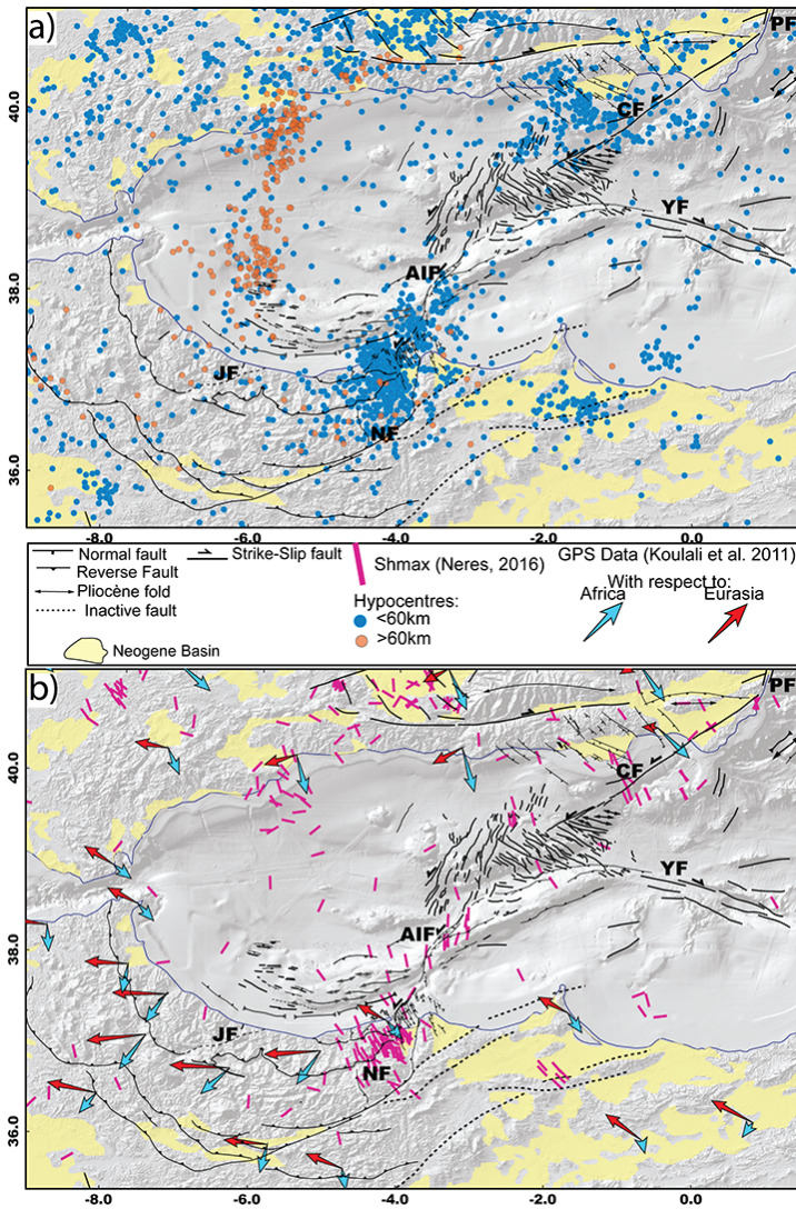
765 Figure 2. Maps showing the distribution of the seismicity along the Neogene tectonic structures in the Alboran Sea. a) Neotectonic map of the Alboran region modified from d'Acremont et al., (2014), Alvarez-Marrón and others, (1999), Chalouan et al., (1997), Estrada et al., (2014), Gràcia et al., (2006), (2012); Lafosse et al., (2016), Martínez-García et al., (2011), Muñoz et al., (2008), Perea et al., (2014); Vázquez et al., (2014) and from this study. Seismicity from IGN catalogue 1970-2017 ( http://www.ign.es/ ), only earthquakes with M_w \geq 3 and depth \geq 2 km are figured. b) GPS data from Koulali et al., (2011) and Sh_{max} from Neres et al., (2016). See figure 1 for scale. CF, Carboneras fault; PF, Palomares fault; YF, Yusuf fault; NF, Nekor fault; AIF, Al-Idrissi fault zone.
