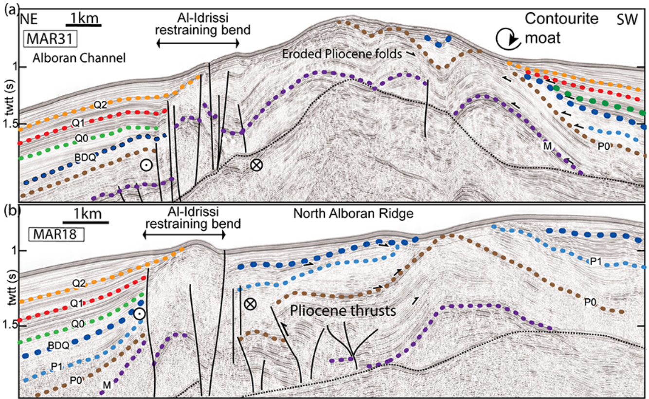
835 Figure 13: Multichannel seismic lines across the left-lateral restraining bend of the Al-Idrissi fault zone showing lateral evolution of the tectonic structures in North Alboran Ridge and in the left-lateral restraining bend. a) The Al-Idrissi fault zone is a positive flower structure following the front of the Alboran Ridge. b) The Al-Idrissi fault zone is a positive flower structure distinct from the Pliocene thrusts and folds.
