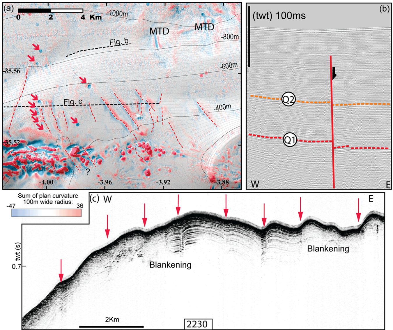
Figure 14: Active structures affecting the northern flank of Francesc Pagès and Ramon Margalef highs. a) plan curvature map overlying the shaded bathymetry; red arrows pockmarks on the seafloor; dashed black lines, seismic lines in the figures (b) and (c); dashed red lines, positions of the fault tracks. b) SPARKER seismic reflection line showing the northward continuity of N145° fault (red line). c) TOPAS seismic line showing the subsurface of the seafloor. Red arrows, positions of the faults drawn in a).
