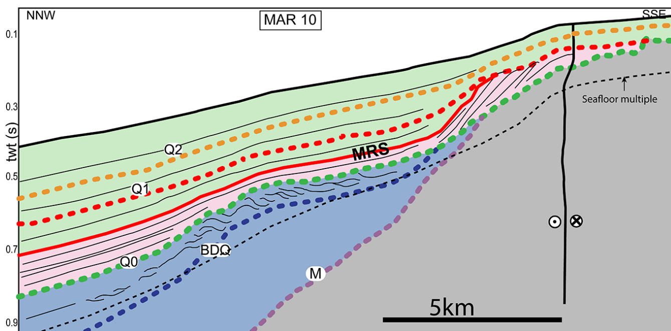
830 Figure 12: SPARKER seismic line showing the transgression of marine sediment (in green) over the prograding shelf of the Nekor Basin (in pink). Oldest depositional units (Pliocene) are colored in blue and the acoustic basement in grey. The Maximum Regressive Surface (MRS) is in red.
