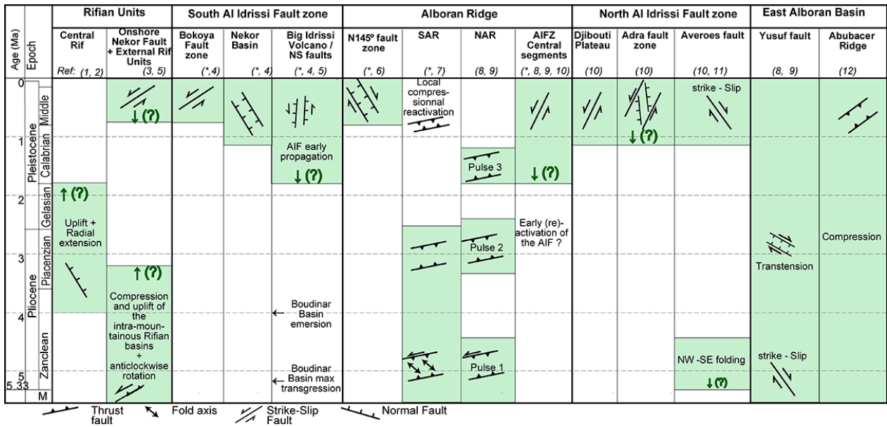
Figure 15: Synthesis of the tectonic events in the Alboran Basin, and the Rif from the literature and the present study. *, this study; (1), Benmakhlouf et al., (2012) ; (2), Romagny et al., (2014) ; (3) Aït Brahim and Chotin, (1990), (4), Lafosse et al., (2017); (5), Azdimoussa et al., (2006); (6), Galindo-Zaldivar et al., (2018); (7) Juan et al., (2016); (8) Martínez-García et al., (2013) ; (9), Martínez-García et al., (2017); (10), Gràcia et al., (2019); (11), Perea et al., (2018); (12) Giaconia et al., (2015). The main tectonic events are in green. Green arrows and question marks indicate the age uncertainties of the main tectonic events.
