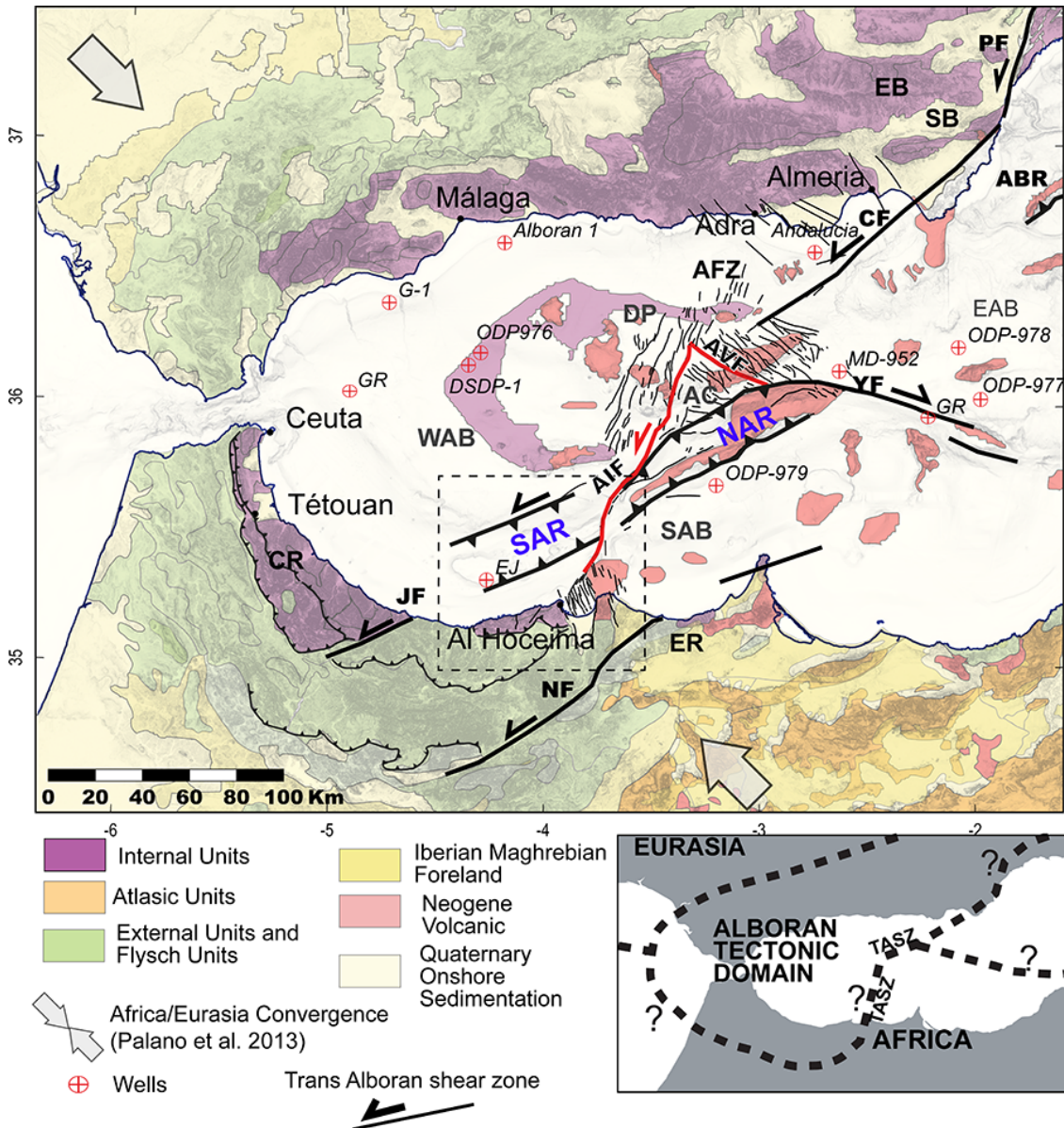
755 Figure 1. Topographic map and principal structural units of the Alboran region. Structural units in the studied area modified from Chalouan et al., (2008); Comas et al., (1999); Leblanc and Olivier, (1984); Romagny et al., (2014). The Trans Alboran Shear Zone (TASZ) indicates the motion inferred for the Late-Miocene – Pliocene period. The red faults are the present-day active Al-Idrissi 760 fault and its conjugated Averroes Fault. AC, Alboran Channel; AFZ, Adra Fault Zone; AVR, Averroes Fault; ABR, Abubacer Ridge; CF, Carboneras Fault; CR, Central Rif; DJ Djibouti Plateau; EB, Eastern Betic; EAB; East Alboran Basin; AIF, Al-Idrissi Fault; ER, Eastern Rif; JF, Jebha fault; NF, Nekor Fault; SAB, South Alboran Basin; SAR, South Alboran Ridge; SB, Sorbas Basin; NAR, North Alboran Ridge; YF, Yusuf Fault; WAB, West Alboran Basin. Inset: Hypotheses of plate boundaries between an Alboran tectonic domain and the African plate from Nocquet, (2012).
