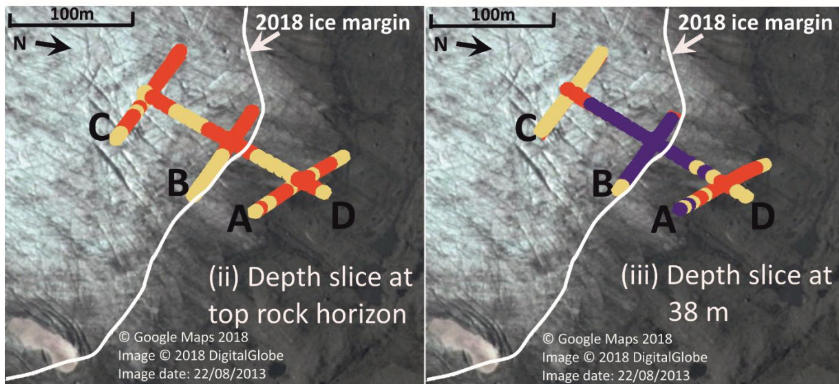
Figure 10. i) 3-D cross-section of lines A-D, showing the subglacial material estimated from applying Vs and resistivity conditions stated in table 3. ii) Depth slice through 3-D cross at the top rock horizon. iii) Depth slice through 3-D cross-section at 38 m.
