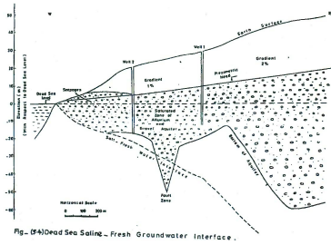
Fig. (D4) Dead Sea Saline - Fresh Groundwater Interface.
