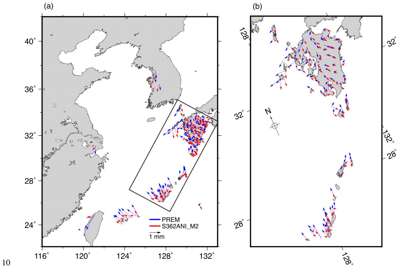
10 Figure 5 Phasor differences between our GPS-observed M_2 vertical OTL displacements and the predictions computed using the NAO99Jb regional ocean tide model (augmented elsewhere globally with FES2014b) and the elastic PREM (blue phasors) and S362ANI_M2 (red phasors) Green's functions. (a) shows the whole ECS region, while (b) is an enlargement of Kyushu and part of the Ryukyu Islands, for the boxed region in (a).
