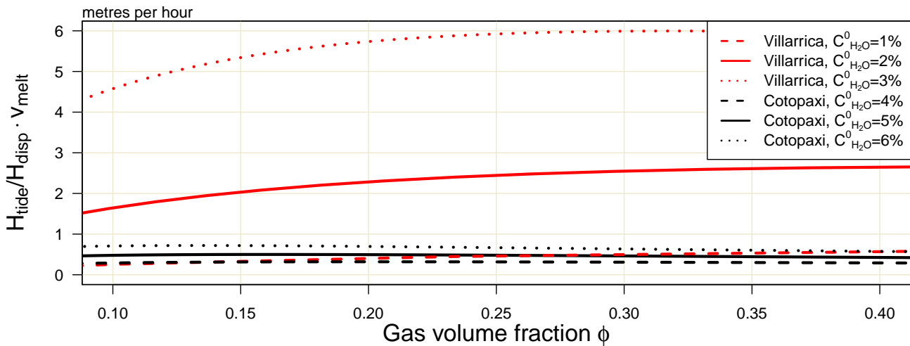
Figure 3. Relative contribution of the tidal mechanism (magnitude given by H_{tide} ) on the bubble coalescence rate for a purely disperse bubble flow (magnitude given by H_{disp} ) in dependency of the gas volume fraction and the initial water weight fraction of the magmatic melt. The corresponding values for \phi are calculated with equation (5) assuming an ideal gas and magma temperatures of 1200°C for Villarrica and 1000°C for Cotopaxi. The relative tidal contribution is displayed as the equivalent to an enhancement of the magma ascent rate which would have the same effect on the bubble coalescence rate. The model increasingly loses validity above the percolation threshold of \phi_{perc} \approx 0.3 .
