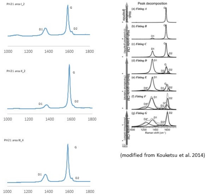
Fig. 1. Representative Graphite Raman spectra of BFZ045 host rock
