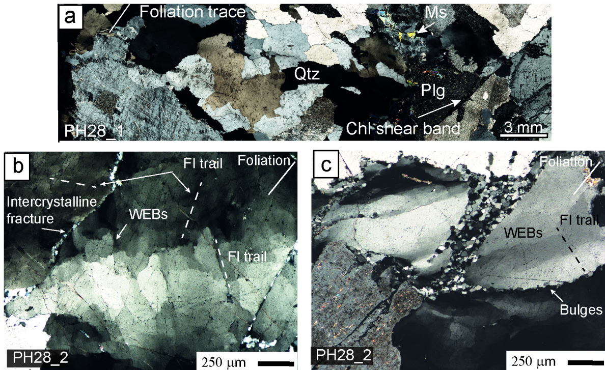
1040 Figure 3. Polarized light microscope images of characteristic lithologies for the damage zone damaged host rock (a), and fault core representative quartz microstructures (b-c). Stitched microphotographs in cross Cross polarized light and plane polarized light. (a) Damage zone shows Host rock showing the original magmatic textures and mineral assemblage of the host rock. White arrow shows a chlorite-rich shear band oriented at a low angle to the mylonitic foliation of the fault core. (b) Mylonite in the fault core. Foliation is defined by the alternation of quartz-rich and mica-rich domains. Porphyroclasts of feldspars are preferentially located in mica-rich domains. (c) Fault core cataclasite BFZ045. (b with characteristic pseudotachylite injection veins (arrow). The cataclasite matrix is enriched in chlorite and Ti oxides. (d) Scanning electron microscope (SEM) image of the pseudotachylite injection vein. Rounded quartz clast (dark grey) and Ti oxides (white) are surrounded by a chlorite and mica-rich ultrafine-grained matrix. Quartz microstructures in the damage zone. Cross polarized light. (a) Quartz with wide extinction bands (WEBS) and undulatory extinction. WEBS are bounded by sets of fluid inclusions trails (FI trail, dashed lines). Intercrystalline deformation bands and well-developed FI trails developed sub-parallel to the mylonitic foliation. (b,c) Polygonal recrystallized quartz grains, with small grain size (~20 μm), forming bands oriented sub-parallel to the mylonitic foliation. The white arrow shows sutured grain boundaries between magmatic quartz grains, indicative of bulging. Foliation trace is projected as a white line on to the images from the adjacent foliated host rock. 1045 1050
