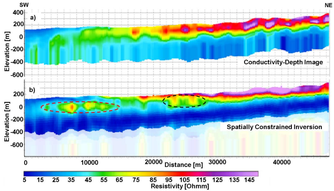
Figure 4: (a) The original Conductivity-Depth Image (CDI) along-in a portion of NE-SW line 2 (Fig. 11a); (b) the associated result obtained with the new data processing and inversion approach (smooth Spatially Constrained Inversion).
