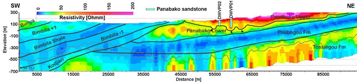
Figure R2.1: Cross-section along SW-NE line 2 across the study area (see Fig. 1a for the location) with the conceptual geological interpretations showing the U-shaped valleys (from about 53 km to 63 km). In addition, also two of the geologic logs (DWVP02 and DWVP01 – Fig. 1a) used for demarcation of lithostratigraphic boundaries and the interpretation/verification of the geophysical model are shown. The two solid grey lines at the bottom represents the DOIs. The three arrows indicate the location of the paleovalleys.
