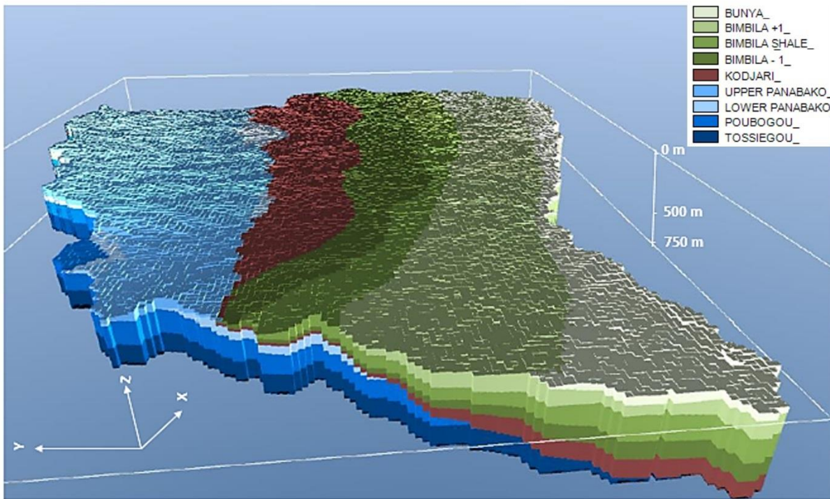
Figure R2.3: 3D geological model of the Nasia sub-basin resulting from the combined interpretation of the B-field airborne data, the prior geological knowledge of the area, and the available wells. With respect to the previous version of this figure, not only, now, the color scale is in agreement with the one of Fig. R2.2, but, in both of them, the legends follow the chronostratigraphic order (with the oldest located at the bottom).
