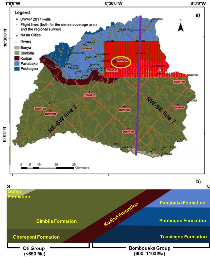
Figure R2.2: (a) Geologic Map of the Nasia sub-basin after Carney et al. (2010) 1 ; the location of some of the available boreholes are indicated (e.g. DWVP01); the red solid lines represents the flight lines of the regional survey (20 km x 20 km grid) and of the dense coverage acquisition (200 m line spacing – in the NE of the Nasia basin – see, also, Fig. 9 in the revised manuscript). (b) Conceptual Model of the geology along a cross sectional N-S line within the study area - solid violet line in the panel (a).
