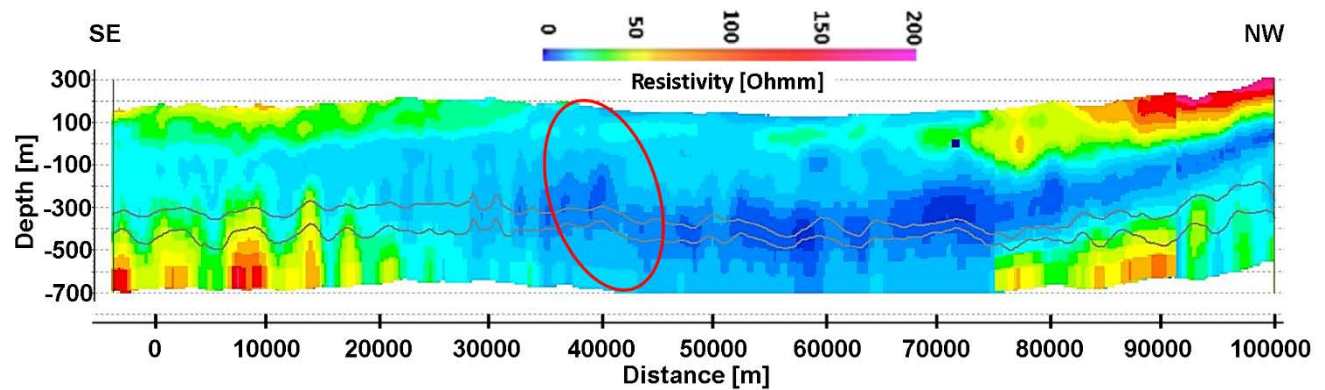
Figure R1.5: Cross-section along NW-SE line 7 (Fig. 1a) showing faulting (within the red circle) in the Bimbila. The DOIs are shown as solid grey lines.
