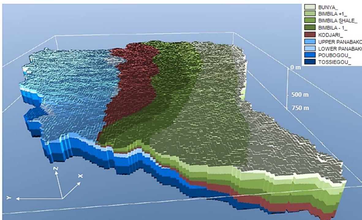
Figure R1.3: 3D geomodel of the Nasia sub-basin. With respect to the original version, the legend in this new figure is presented in stratigraphic order and with the intent of making more evident the group subdivisions.
