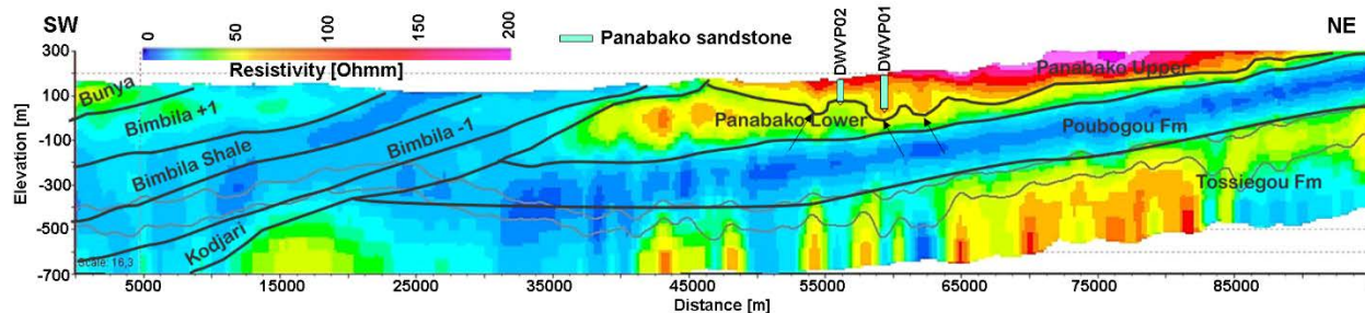
Figure R1.4: Cross-section along SW-NE line 2 across the study area (see Fig. 1a for the location) with the revised conceptual geological interpretations showing the U-shaped valleys (around ~60 km). In addition, also two of the geological logs (DWVP02 and DWVP01 – Fig. 1a) used for demarcation of lithostratigraphic boundaries and the interpretation/verification of the geophysical model are shown. The two solid grey lines at the bottom represents the DOIs. The three arrows indicate the location of the paleovalleys.
