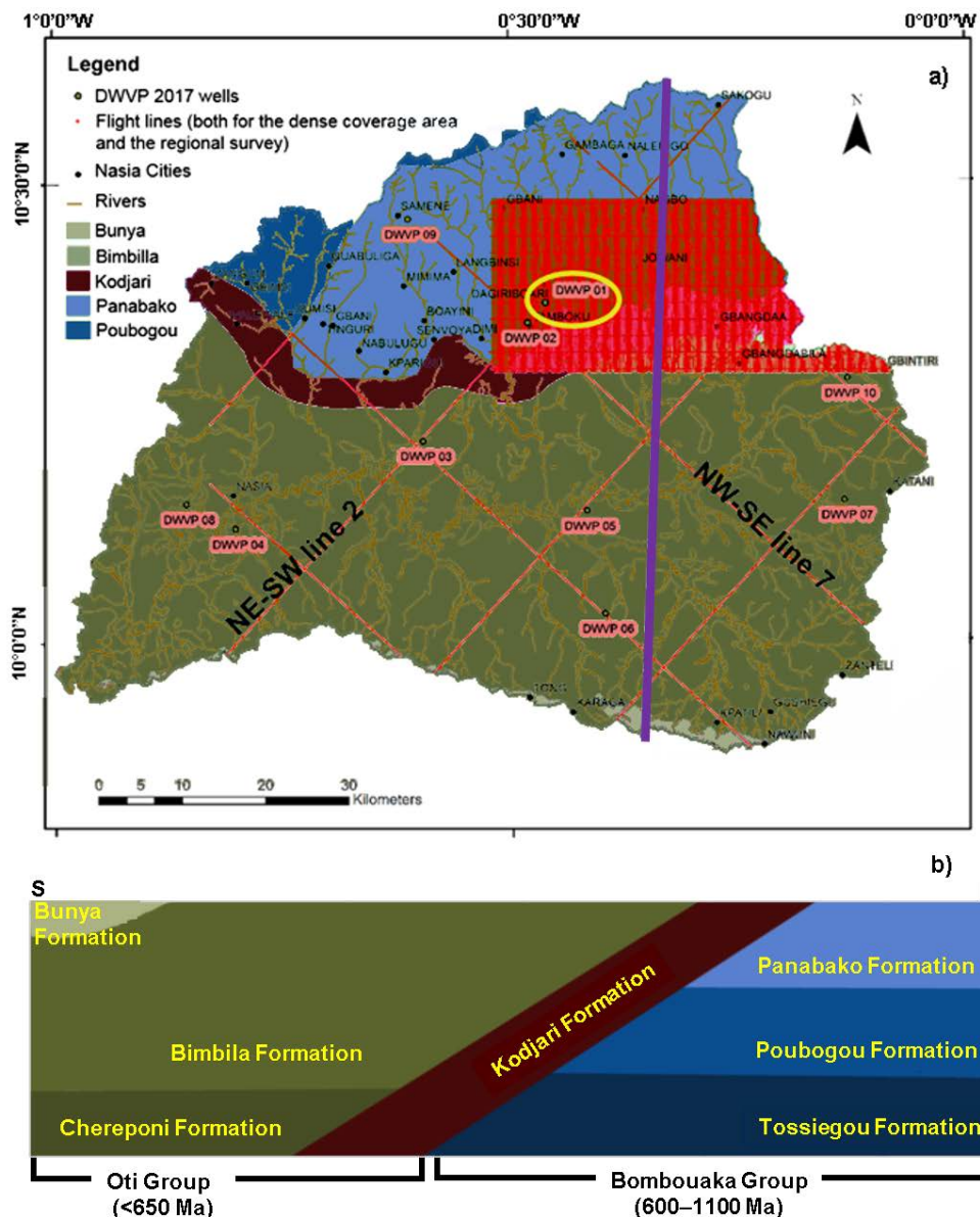
Figure R1.2: (a) Geologic Map of the Nasia sub-basin after Carney et. al (2010) 1 ; the location of some of the available boreholes are indicated (e.g. DWVP01); the red solid lines represents the flight lines of the regional survey (20 km x 20 km grid) and of the dense coverage acquisition (200 m line spacing – in the NE of the Nasia basin – see, also, Fig. 9 in the revised manuscript). (b) Conceptual Model of the geology along a cross sectional N-S line within the study area - solid violet line in the panel (a).
