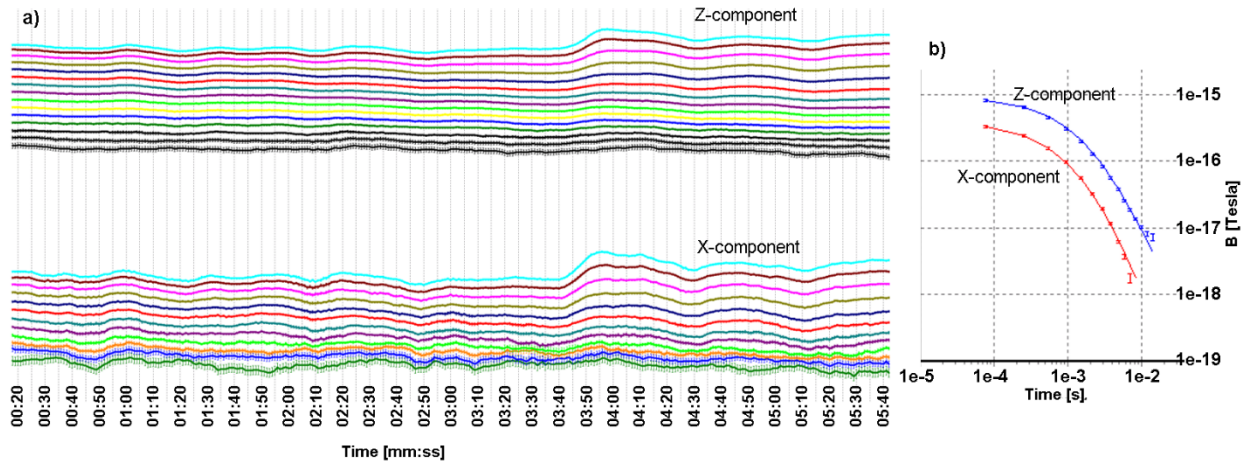
Figure R1.4 (a) An example of the Z and X components of the B-field data (with their uncertainty shown as vertical bars) obtained after the application of the moving window stacking with width varying with the time-gates. (b) Example of a typical sounding (Z and X components): the vertical bars represent the stacked data with the associated uncertainty; the solid lines are the calculated data corresponding to the inversion model (not shown).
