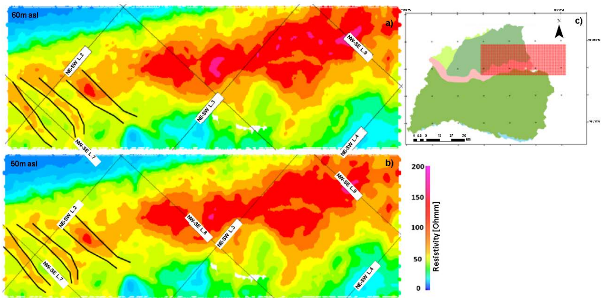
Figure R1.1: Horizontal resistivity slices at 60 m (a) and 50 m (b) depth of the portion of the study area - in red in the panel (c) - characterized by a geophysical sampling much denser (200 m line-spacing) than the regional survey - for comparison, the flight lines from “NE-SW L.2” to “NW-SE L.9” in both panels are characterized by a 20 km x 20 km spacing (e.g., “NE-SW L.2” corresponds to a portion of NE-SW line 2 in Fig. 1a).
