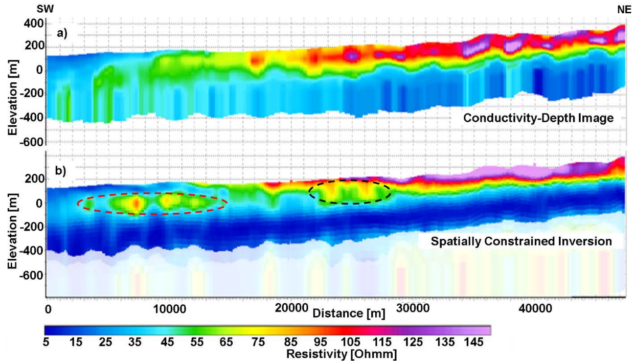
Figure R1.5 (a) The original Conductivity-Depth Image (CDI) along NE-SW line 2 (Fig. 1a); (b) the associated result obtained with the new data processing and inversion approach (smooth Spatially Constrained Inversion).
