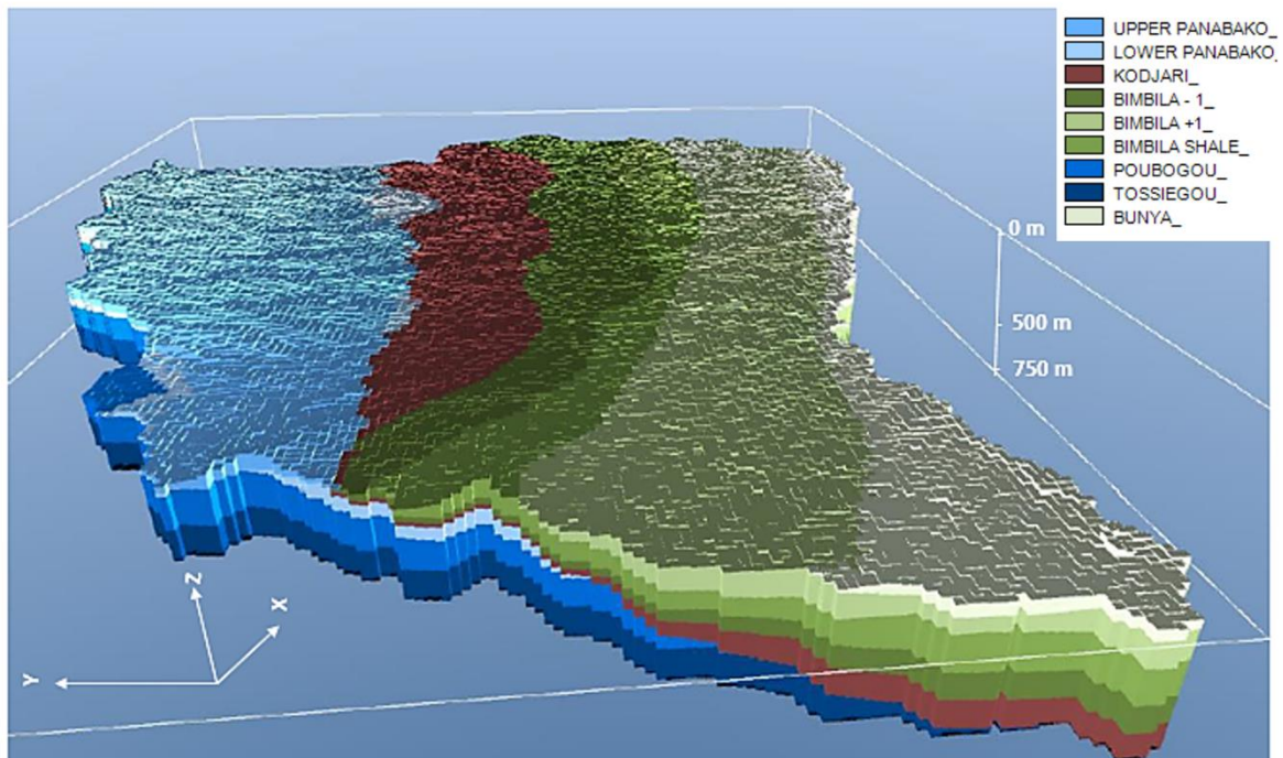
565 Figure 5. 3D geological model of the Nasia sub-basin resulting from the combined interpretation of the B-field airborne data, the prior geological knowledge of the area, and the available wells.
