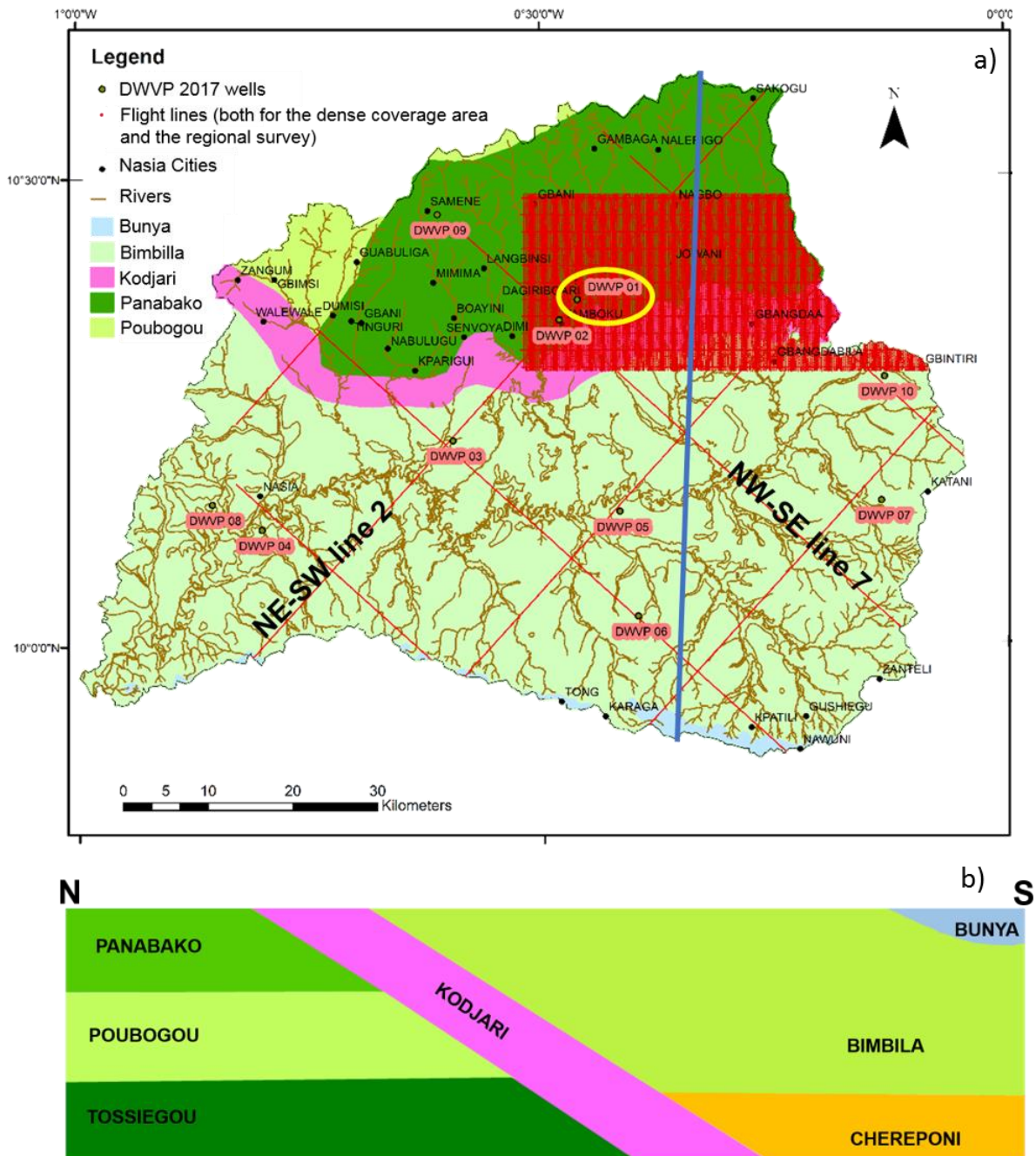
550 Figure 1: (a) Geologic Map of Nasia sub-basin after Carney et. al (2010); (b) Conceptual Model of the geology along a cross sectional N-S line within the study area (solid blue line in the panel a).
