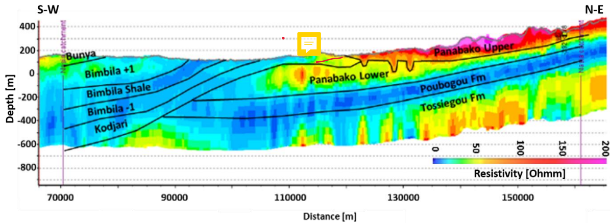
Figure 7. Cross-section from the North along NE-SW line 2 of the study area (see Fig.1a for the location) with conceptual geological interpretations showing U-shaped valleys (between 120 and 130 km).
