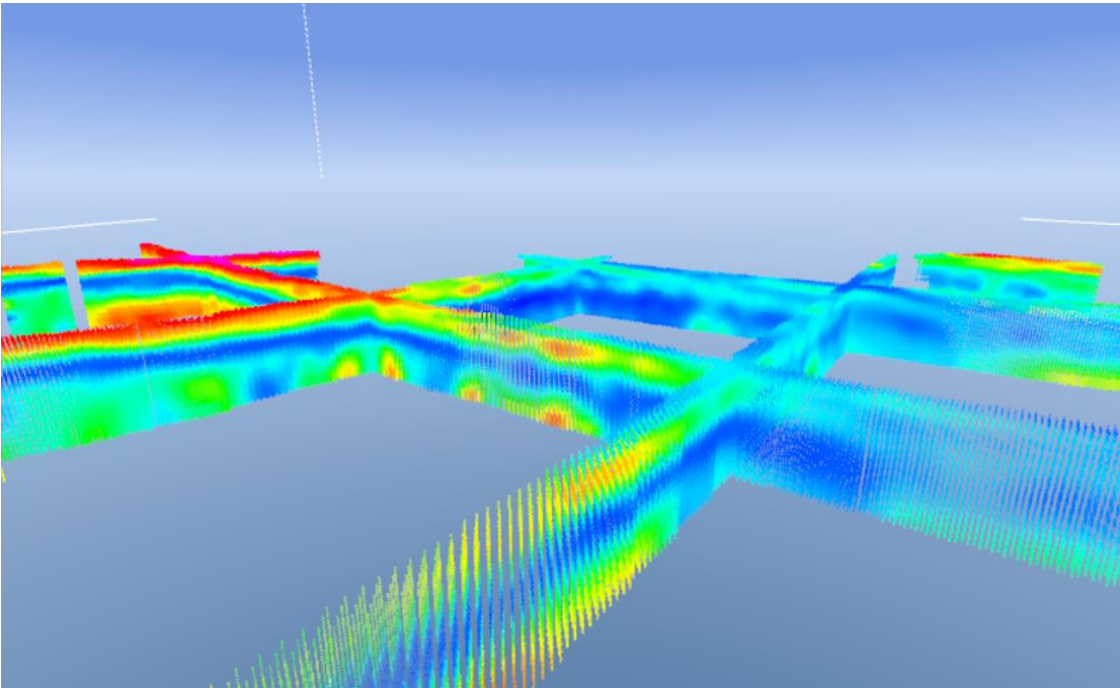
Figure 3. A 3D view of the B-field SCI results along the 20km x 20km grid lines in the study area. These soundings were used as basis for geologic interpretation and modelling.
