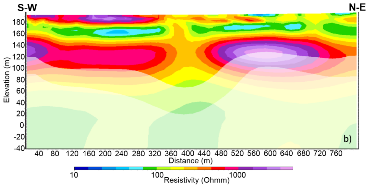
560 Figure 4. Results of the ERT performed preliminarily to the drilling of the DWVP 01 well (the location of the midpoint of the line is shown in Fig.1a, highlighted by a yellow circle). The sensitivity of the data with respect to the model parameter values reduces significantly below the depth of investigation (DOI – Asch et al., 2015) that is indicated by the white overlay.
