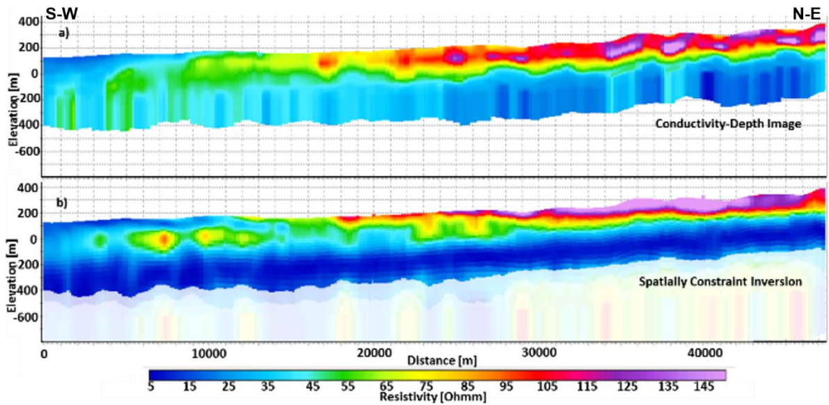
Figure 2. (a) The original Conductivity-Depth Image (CDI) along NE-SW line 2 (Fig. 1a); (b) the associated result obtained with the new data processing and inversion approach (smooth Spatially Constrained Inversion).
