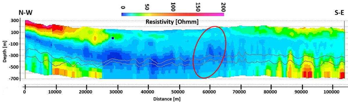
Figure 8. Cross-section along NW-SE line 7 (Fig. 1a) showing faulting (within the red circle) in the Bimbila. The DOI is showed as a solid grey line (there are two of them accordingly to their definition – more details on this distinction can be found in Christiansen and Auken, 2012).
