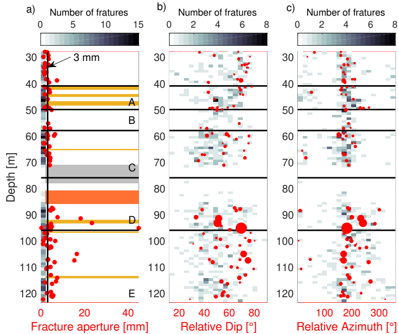
Figure 5. Summary of the brittle deformation based on the OTV data Egli et al. (2018) a) fracture aperture, b) relative dip and c) relative azimuth. All identified fractures are displayed in histogrammic form along the borehole. Fractures with measurable aperture (greater than 0.8 mm) are displayed as red dots. In a) additionally cataclastic zones, the cementation zone and main fault core are plotted.
