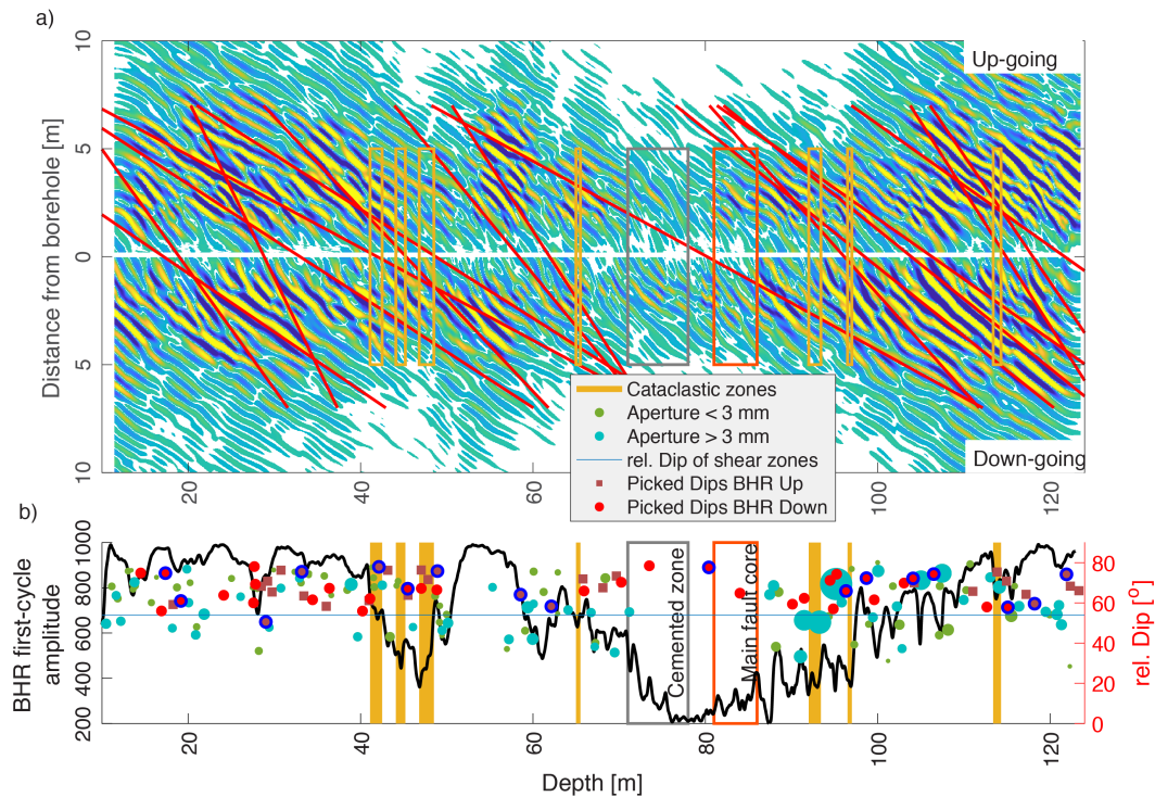
Figure 3. a) Migrated BHR image consisting of the up- and down going reflection data plotted in positive distance from the borehole trajectory. Red lines denote selected reflection events used for estimating the dips and locations of the associated fractures. b) Maximum first-cycle amplitude of BHR first arrivals (black line), relative dip of fractures from OTV data (turquoise dots) and relative dips picked from the depth-converted BHR reflection image (red dots and squares). For the OTV data, the size of the dots is a relative measure of fracture aperture. The dips of events denoted by red lines in a) are identified by red dots encircled in blue.
