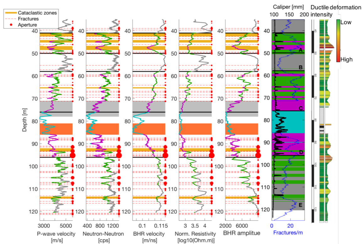
Figure 7. Borehole log data used for cluster analysis color-coded according to the four cluster groups identified in Fig. 6 and overlain by brittle deformation inferred from the OTV data. The right-hand column shows the sequence of clusters along the borehole together with the fracture density inferred from the OTV data, the ductile deformation intensity log (Egli et al., 2018), the caliper data as well as the zonation A through E inferred from the Stonely wave analysis (Fig. 4).
