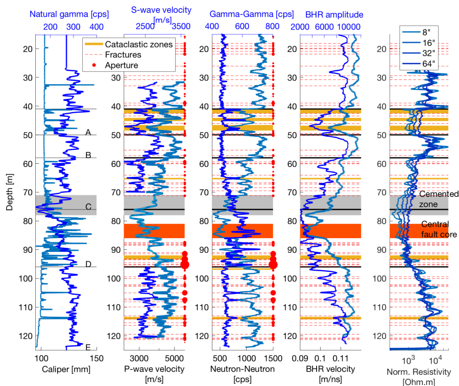
Figure 5. Representative selection of borehole log data comprising from left to right caliper, natural gamma, sonic velocity, Neutron-Neutron and Gamma-Gamma, BHR direct-wave velocity and amplitude as well as normal resistivity logs. The brittle deformation features interpreted from the OTV data (Egli et al., 2018) are superimposed on the log data. The sizes of the circles are indicative of the relative fracture apertures. Zones A through E refer to zonation shown in Fig. 4.
