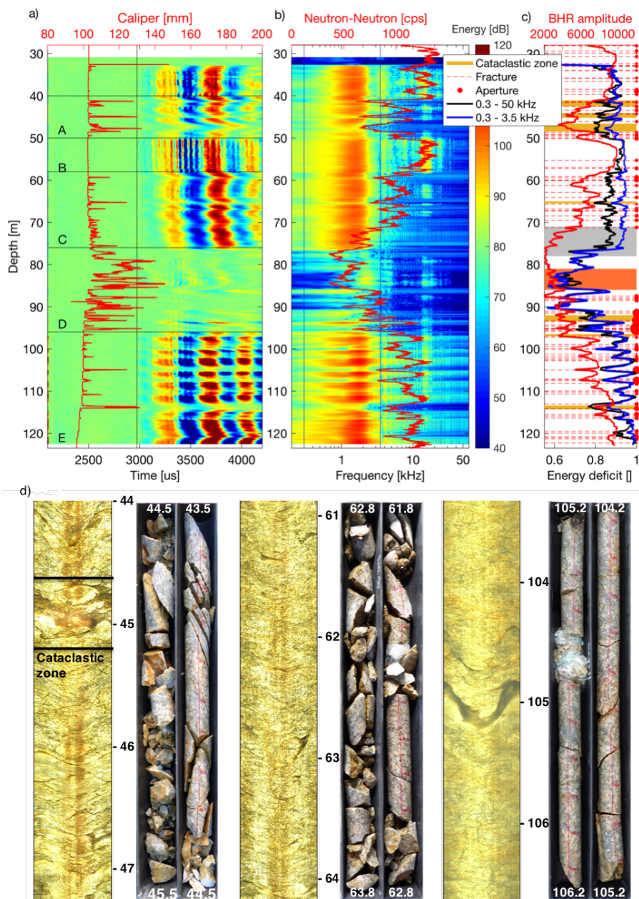
Figure 4. a) Low-gain FWS data acquired with a nominal central frequency of 2 kHz overlain by the caliper log; b) corresponding power spectrum overlain by the Neutron-Neutron log; c) relative energy deficit for two different frequency bands, one capturing the Stoneley wave and the other the complete spectrum, in conjunction with the first-cycle amplitude of the BHR direct wave and the brittle deformation data from the OTV; d) examples of brittle deformation based on a comparison of OTV data and corresponding drill core sequences.
