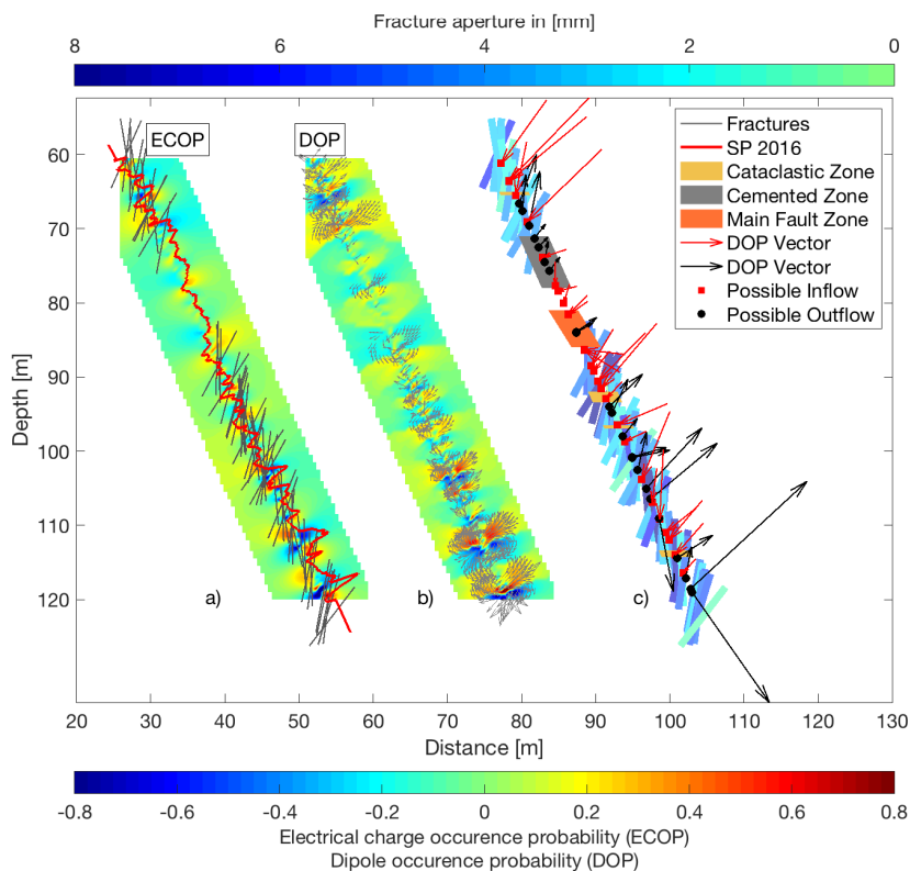
Figure 11. a) Electric charge occurrence probability (ECOP) and b) dipole occurrence probability (DOP) maps along the borehole track overlain by the SP log and fractures from OTV data, and DOP vectors with an absolute probability larger than 0.15, respectively. c) Most probable DOP vectors in each 1.2 m interval mapped onto the borehole track together with a projection of fracture planes and their color-coded apertures.
