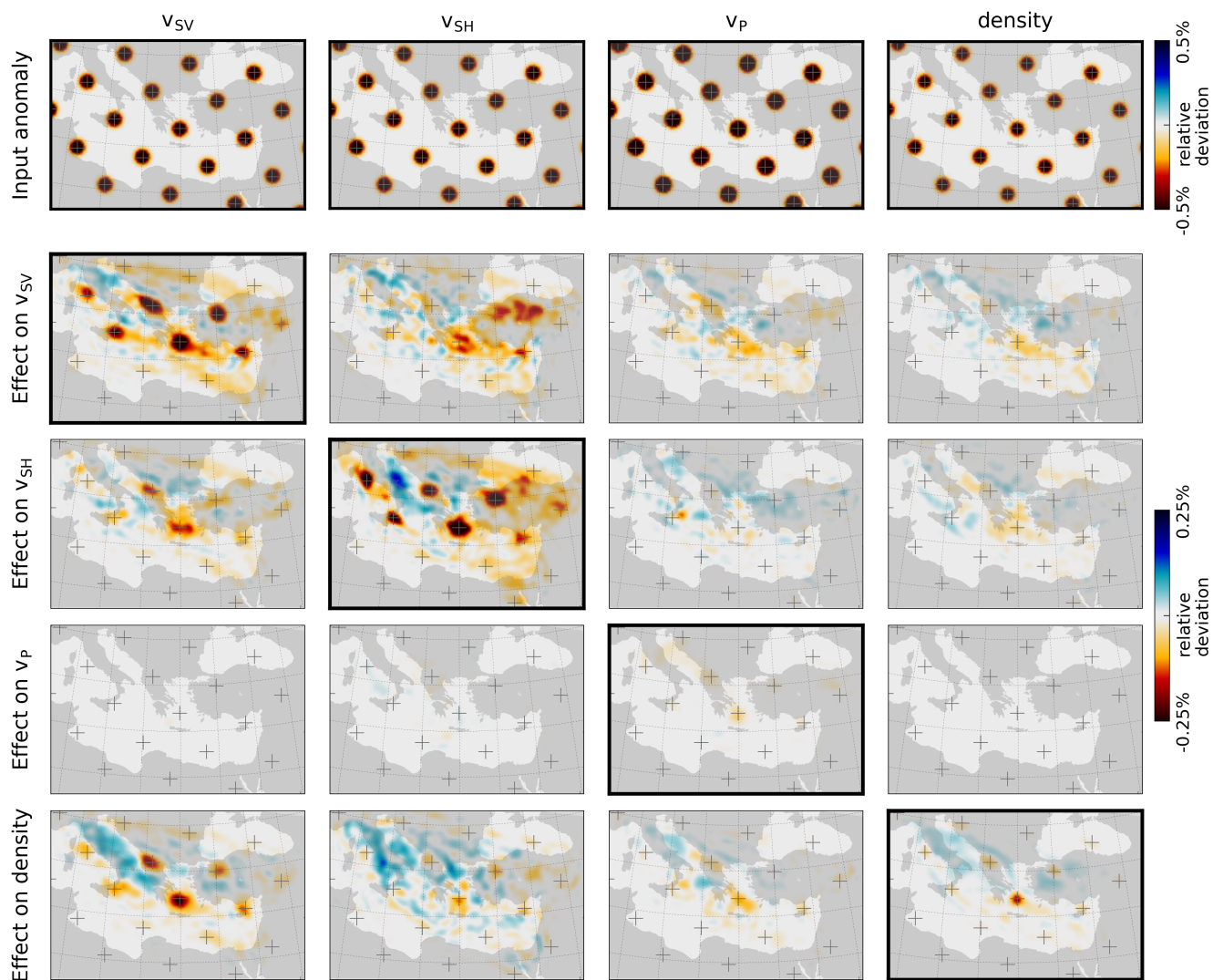
Figure 15. Spike tests conducted for model 91 in the period band 28–150 s, designed in the spirit of Rawlinson and Spakman (2016). Each of the columns represents a separate test with a checkerboarded grid of spikes in one of the parameters. We denote the original model as \mathbf{m}_{91} , the model with spikes as \mathbf{m}_s and the model produced after 5 iterations as \mathbf{m}_{s+5} . The updated reference model is \mathbf{m}_{96} . The top row represents the input anomaly for that particular parameter, where we show \mathbf{m}_o - \mathbf{m}_s . In the following four rows, we show the cumulative model update after five iterations – i.e. (\mathbf{m}_{s+5} - \mathbf{m}_s) - (\mathbf{m}_{96} - \mathbf{m}_{91}) – for each of the parameters. Results are shown for a depth of 100 km.
