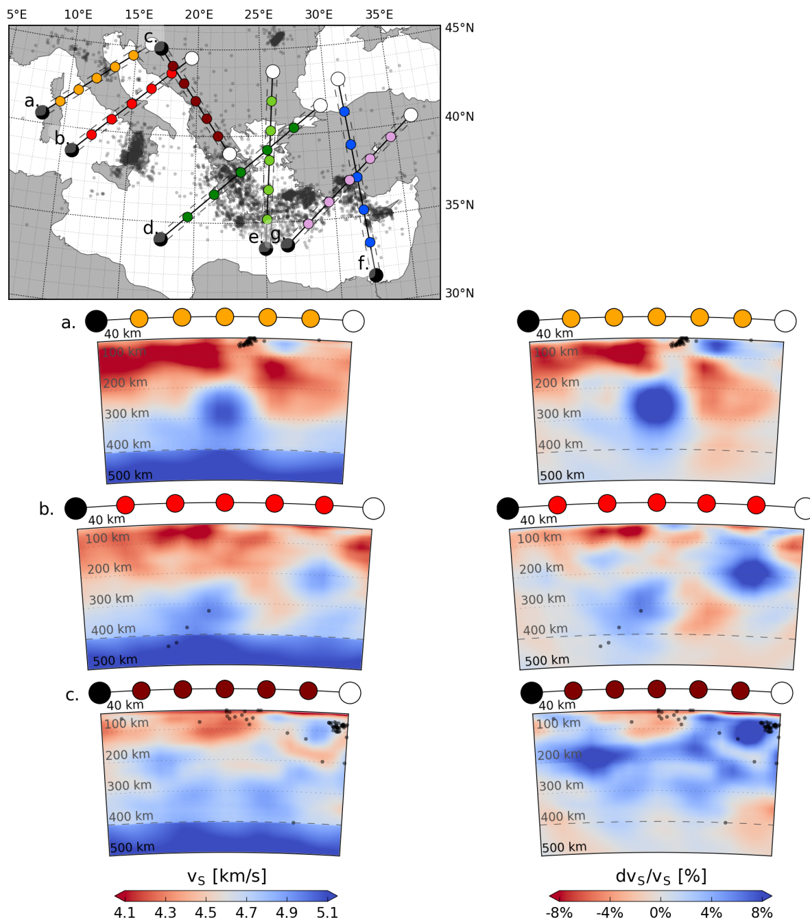
Figure 12. Cross-sections through the S velocity model and a map showing their locations. Left column: isotropic S velocity v_s , right column: relative deviations in v_s from the depth-averaged starting model. Black dots indicate seismicity in the region, as obtained from the EMSC-CSEM catalogue (2004–August 2019, depths greater than 40 km and M > 2 ; Godey et al., 2013). Seismicity on the cross-sections is plotted if it is within 50 km from the cross-section slice. (top) Map showing the locations of the cross-sections. (a) Cross-section across Northern Italy (anomaly A) (b) Cross-section across Italy and the Dinarides (anomalies A & B) (c) Cross-section parallel to the Dinaric anomaly (anomaly B)
