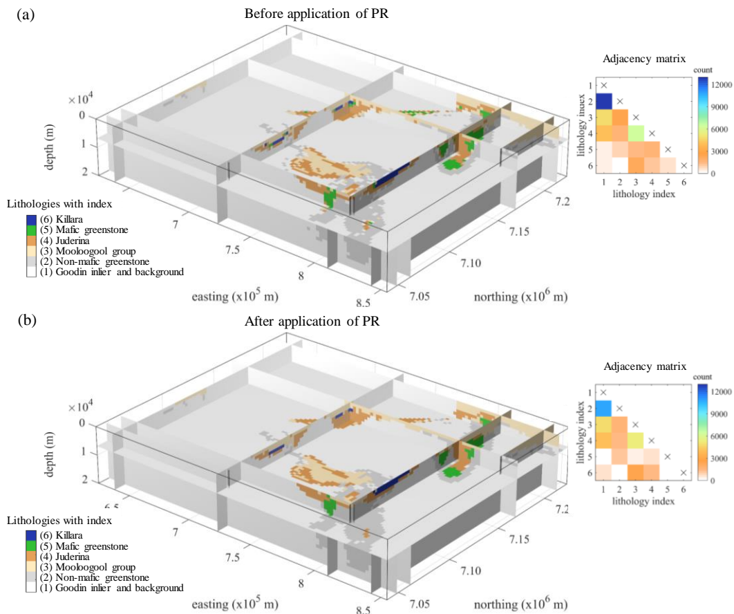
10 Figure 9. Recovered lithologies before post-regularisation (a) and after (b) next to the corresponding adjacency matrix (right hand side). The indices used to designate lithologies are indicated in the legend of the volume (left hand side).
