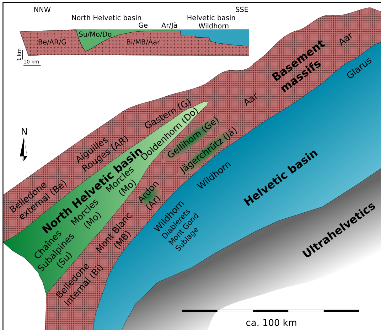
Figure 2. Simplified paleogeographic map of the lower cretaceous Cretaceous showing the assumed distribution of the basement massifs and sedimentary units forming the discussed tectonic nappes of the Helvetic nappe system (modified after Epard, 1990 and Pfiffner, 2015). The cross section on the top left represents shows a representative section through across the Helvetic nappe system in the SW region across of the Helvetic -nappe system (modified after Jaquet et al., 2018).
