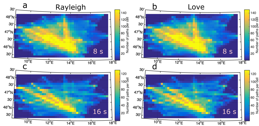
Figure 6. Path density map for the tomography inversion: a, c) for Rayleigh waves at 8 and 16 s respectively, and b, d) for Love waves at 8 and 16 s. The path coverage is generally good for the entire region. Most of the cells have path density more than 20 rays per cell. path density map at larger periods are also shown in Supplementary Figure S3.
