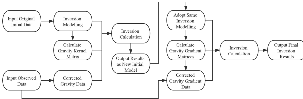
Figure 4 The flowchart for the whole PCG inversion algorithm procedure.
