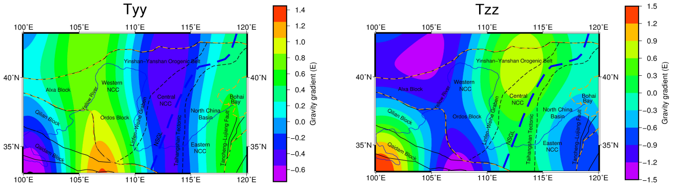
480 Figure 12 The gravity gradient effect ( T_{xx} , T_{xz} , T_{yy} , T_{zz} ) caused by the lithosphere under 180 km.
