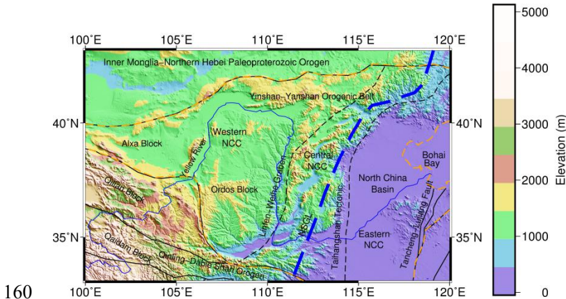
Figure 1 Topography and main tectonics of the study area. NCC - North China Craton.
