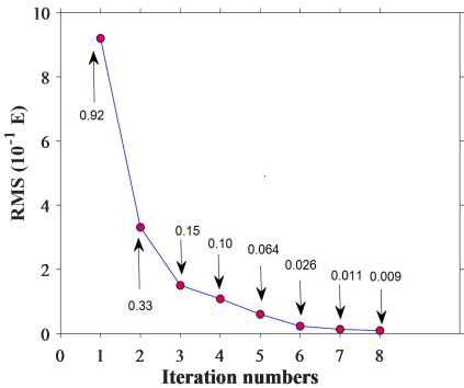
545 Figure 14 For the iterative calculation, the residual mean square between the forward calculated theoretical gravity gradient and the gravity gradient measurements versus the iteration number in the PCG inversion algorithm.
