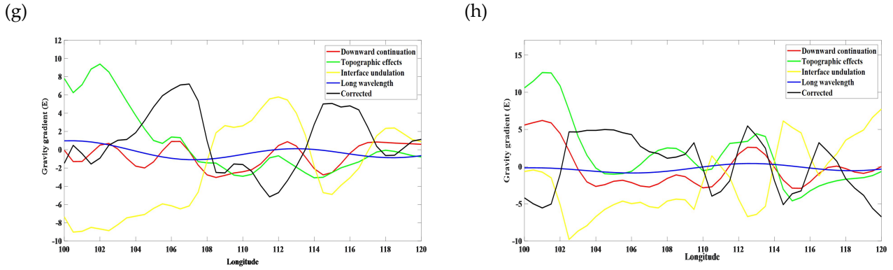
Figure 13 The corrected gravity gradient components (a) T_{xx} , (b) T_{xz} , (c) T_{yy} , and (d) T_{zz} . Gravity gradient effects with extended area (e) Topographic effects T_{zz} . (f) Interface undulation T_{zz} (Sedimentary and Moho) effects. Several corrections T_{zz} at different cross sections: (g) Latitude 35° and (h) Latitude 37.5°.
