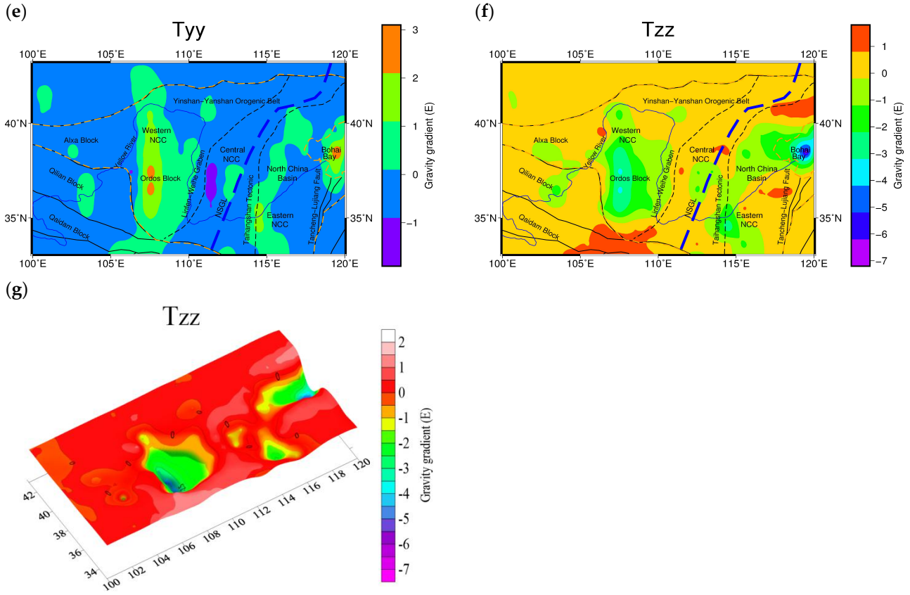
405 Figure 10 (a) Sedimentary layer interface of the NCC. (b) Sedimentary layer interface undulation of the NCC. The anomalous gravity gradient component caused by the relief at the sedimentary layer interface undulation, (c) T_{xx} , (d) T_{xz} , (e) T_{yy} , and (f) T_{zz} . (g) The 3D gravity gradient effect T_{zz} of the sedimentary layer interface undulation.
