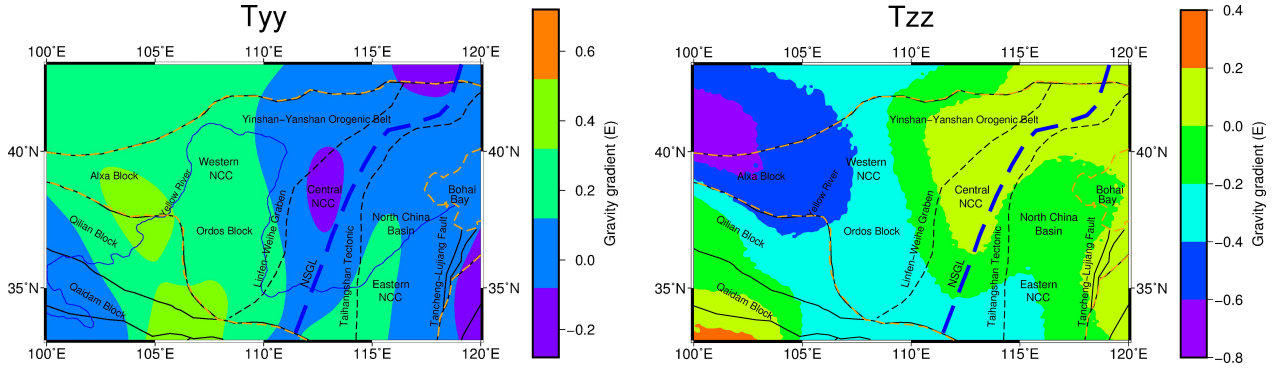
Figure 7 Gravity gradient anomaly ( T_{xx} , T_{xz} , T_{yy} , T_{zz} ) after average orbital correction to an altitude of 250 km.3.3 Downward continuation
