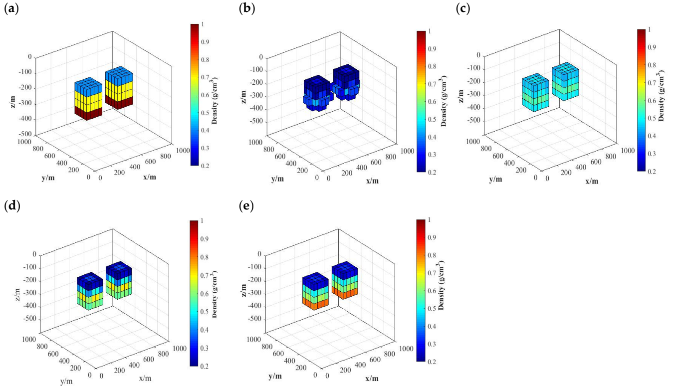
270 Figure 2 Initial density model experiments. (a) True model. Inversion results for (b) Test 1, (c) Test 2, (d) Test 3, and (e) Test 4.
