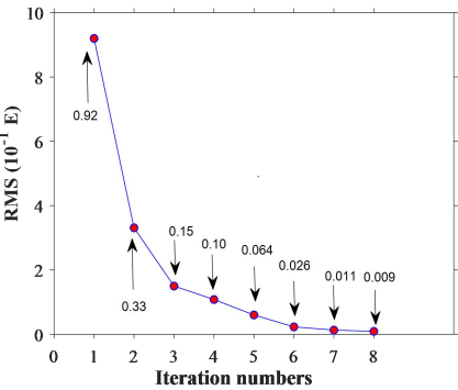
Figure 14 For the iterative calculation, the residual mean square between the forward calculated theoretical gravity gradient and the gravity gradient measurements versus the iteration number in the PCG inversion algorithm.
