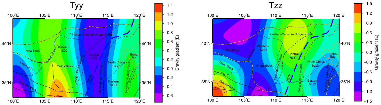
430 Figure 12 The gravity gradient effect ( T_{xx} , T_{xz} , T_{yy} , T_{zz} ) caused by the lithosphere under 180 km.
