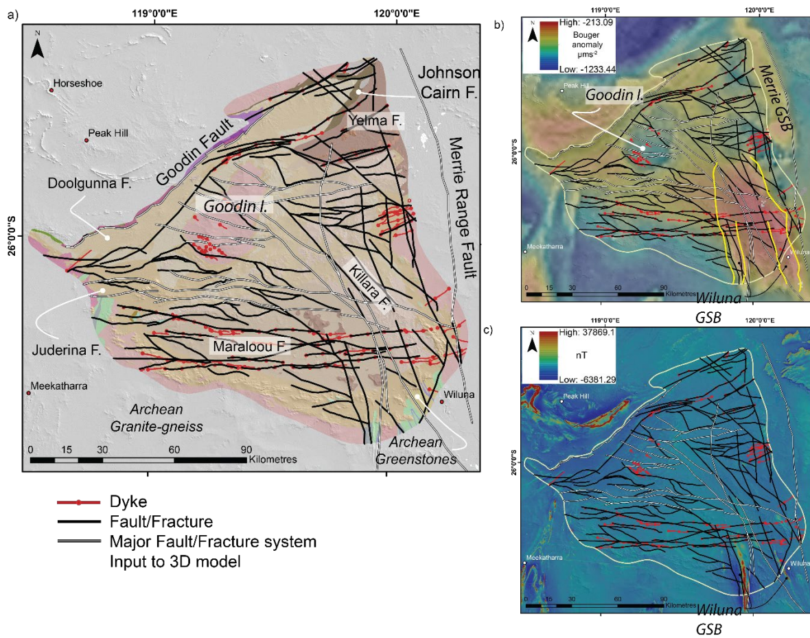
780 Figure 6. Simplified structural geophysical interpretation of the southern Yerrida Basin. (a) Integrated interpretation of structure and rock units with the highlighted major fault systems input to the 3D model (refer section 4.6 3D Model). (b) Interpreted structure shown with gravity data (blended image: Bouguer anomaly shown in colour with 1VD of the Bouguer anomaly in greyscale). (c) Interpreted structure shown with blended magnetic data (blended image: RTP shown in colour with 1VD of the RTP shown in greyscale). GSB = greenstone belt.
