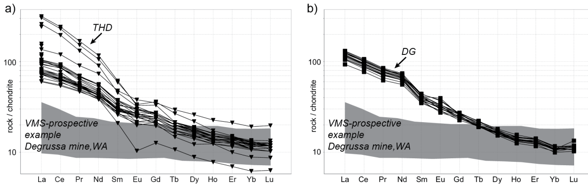
830 Figure 16. REE spider diagrams for mafic rocks sampled from a) THD001 and b) DGDD347. Note the inclined profiles for each indicated a non-prospective environment for VMS mineralisation. The shaded portion indicates a VMS-prospective example taken from basaltic and micro-gabbroic rocks sampled from the Degrussa mine (Hawke, 2016).
