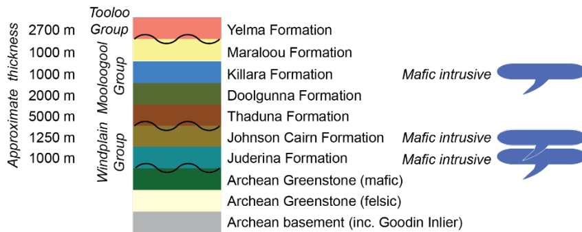
770 Figure 2. Stratigraphy and input for the Yerrida Basin 3D model modified from Occhipinti et al. (2017). The position of unconformities is indicated with a wavy line and approximate thicknesses are given. The position of the mafic intrusives is shown to indicate the possible stratigraphic position being tested by geophysical modelling. Unit colours correspond to those used in the 3D model (refer Section 4.6 3D Model and Figure 10).
