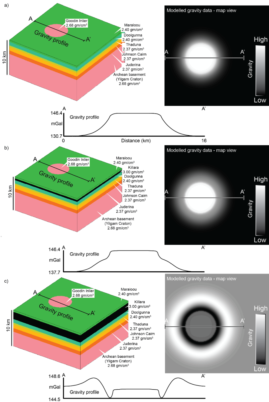
Figure 8. Conceptual forward modelling results obtained from Noddy. (a) No Killara formation; (b) 500 m of Killara Formation and (c) 2000 m of Killara Formation.
