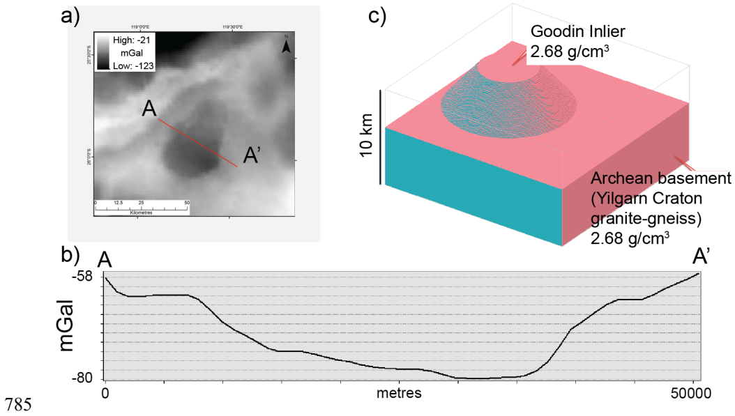
Figure 7. Initial conceptual model using 'Noddy': a) the observed gravity response from a part of the Yerrida Basin, showing the location of the profile in part b); b) curve representing the gravity response of the Goodin Inlier taken from the observed gravity; c) initial conceptual 3D model of the Goodin Inlier. The Yerrida Basin sedimentary rocks are modelled, but are not shown here for better visualisation of basement geometry.
