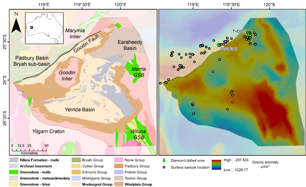
765 Figure 1. a) Location and geology of the Yerrida Basin, Capricorn Orogen. b) Bouguer gravity image of the Yerrida Basin shown with sampling locations for petrophysical and geochemical data. Points represent surface sample locations; diamonds represent location of diamond-drilled core collars with name. Significant regions are labelled, with Archean rocks shown with italic font. GSB = greenstone belt. The legend lists group-level stratigraphic units and those shown in bold are described in Figure 2. The shaded region indicates those outside the study area,
