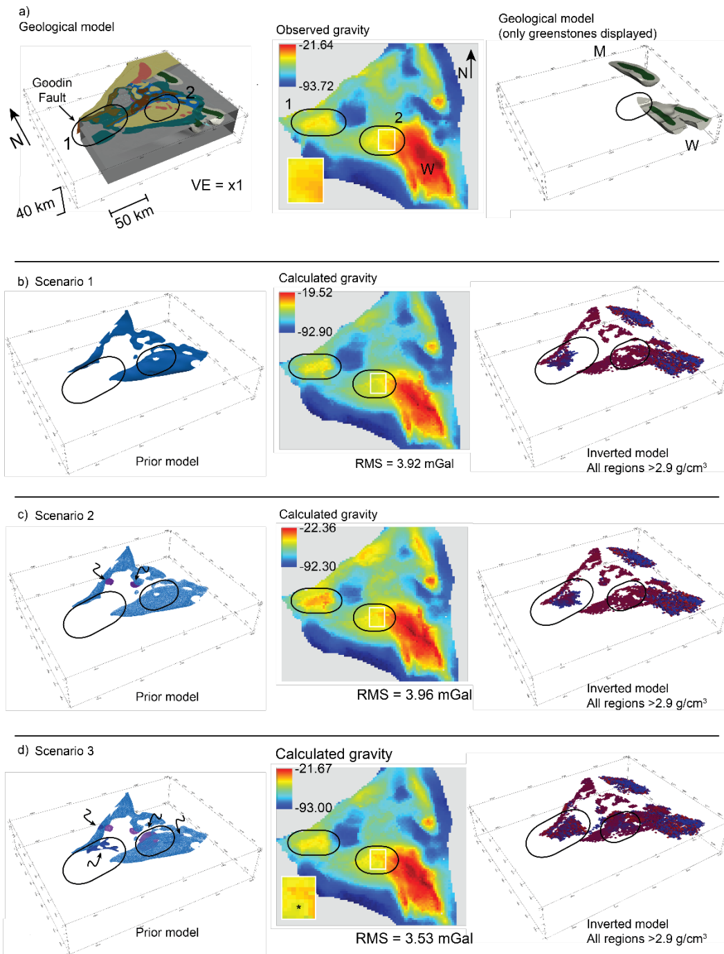
Figure 11. Geological models and mafic intrusive scenarios subjected to inversion modelling. a) Top panel: 3D geological model (left); observed gravity response (centre); location of greenstone belts (right). b-d) Results from scenarios 1-3 respectively: (left) position of mafic intrusions; calculated gravity response from inversion (centre); distribution of locations determined by the inversion to be >2.9 g/cm 3 (right). Scenario 2 and 3 incrementally introduce mafic bodies to the prior model (left-hand panes, c and d), as indicated by the arrows. Colours in the gravity response indicate blue = low; yellow = moderate; red = high.
