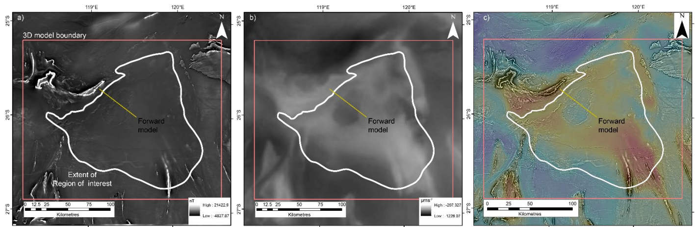
775 Figure 3. Geophysical grids and forward model location trace (as indicated). a) Magnetic anomaly, b) Bouguer gravity anomaly and c) blended image of Bouguer anomaly (colour) and 1VD of the RTP magnetic data (greyscale).
