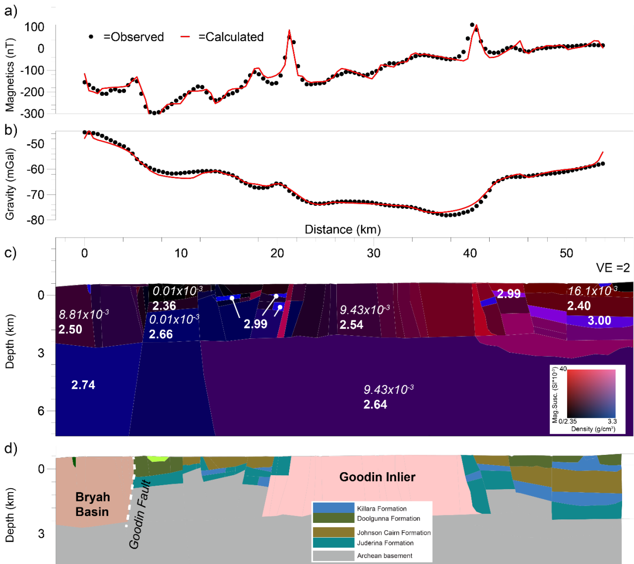
Figure 9. Section-based forward modelling of the Yerrida Basin and Goodin Inlier – location of profile shown in Figure 2. The top two panels show the degree of fit between the observed (points) and calculated (line) geophysical response for magnetic (a) and gravity (b) data. The middle panel (c) shows the petrophysical model that was used to model the calculated geophysical response. Indicative petrophysical values are shown (bold: density – g/cm 3 ; italics – susceptibility Six10-3) to help guide visualisation of the colour scale shown at right. The bottom panel (d) shows the geological interpretation made from the petrophysical model. Boundaries shown at the surface of the model are sourced from field observation and interpretation (refer section Table A 1).
