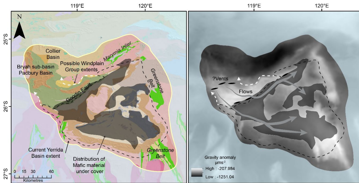
835 Figure 17. Proposed source of magmatism for the mafic component of the Yerrida Basin. The lack of an Archean signature in the mafic rocks suggests that conduits for magmatism do not include the Yilgarn Craton rocks that underlie the Yerrida Basin, but likely sourced from the northwest or along the current position of the Goodin Fault. a) Major components of the southern Capricorn region are shown, with Archean regions listed in italics. Shaded regions show the position of mafic material determined via geophysical inversion. b) Vent locations and flow or sill intrusion paths are proposed and shown over the Bouguer gravity anomaly.
