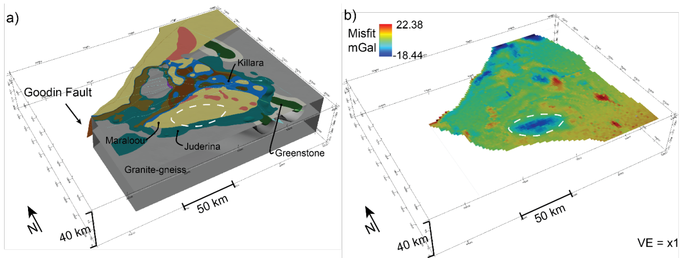
810 Figure 12. Assessing the plausibility of the Yerrida Basin model with geological knowledge and geophysical inversion. a) The 3D 815 model representing scenario 3 and b) the remaining misfit between the inverted geological model and geophysical data. Misfit values after regional trend effects were removed using a linear solver. Red = density exceeds that required by observed gravity, blue = density lower than that required by observed gravity. Note the large region of misfit outlined by the white dashed line that indicates the position of where a portion of high-density material needs to be added to reduce misfit. The cause of this misfit is considered to be in response to the modelled sedimentary basin rocks being too thick and not hosting the required volume of mafic material.
