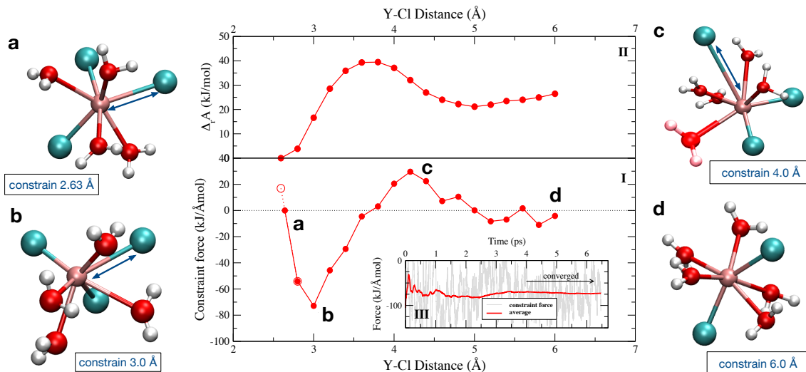
Figure 2. (I) potential of mean force of the dissociation reaction of \text{YCl}_3 to \text{YCl}_2^+ at 1.3 GPa and 800 °C over a distance between 2.63 Å and 6.0 Å. The evolution of the Helmholtz free energy is shown in (II). (a-d) indicate the different stages of the dissociation of the initial complex (see text for details). (III) shows exemplary the progress of the constraint force with simulation time for stage b for a Y-Cl distance of 3.0 Å.
