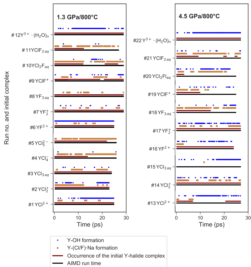
Figure 5. Presence of selected ion pairs or complexes during the different AIMD simulations. This includes the formation of \text{OH}^- within the first hydration shell of yttrium, the association of sodium with the coordinating halogens and the stability of the initial Y-halide complexes over AIMD time.
