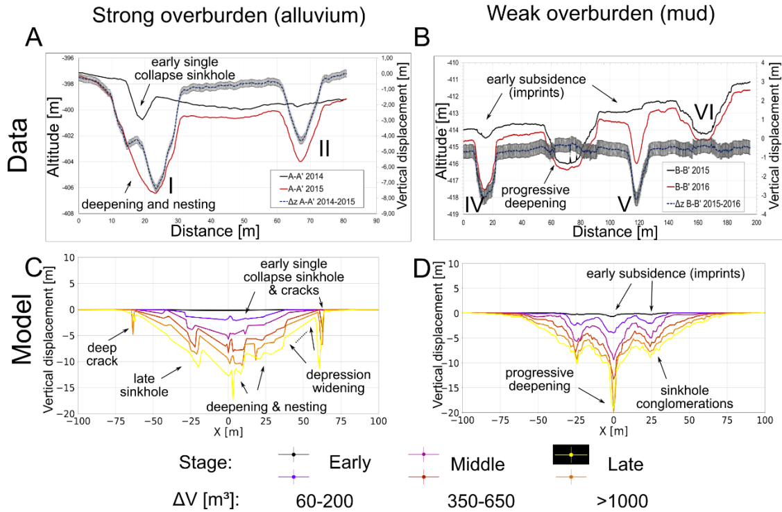
Figure 11: Topographic profiles data as indicated in Figure 10 and corresponding models. Top row: Topography and vertical displacement. Figure 10 of (A) cross-section A-A' from SW-NE in the alluvium and (B) cross-section B-B' from W-E in the mud-flat. Bottom row: Representative topographic profiles across final models for (C) high strength alluvium on mud and (D) low-strength lacustrine mud.
