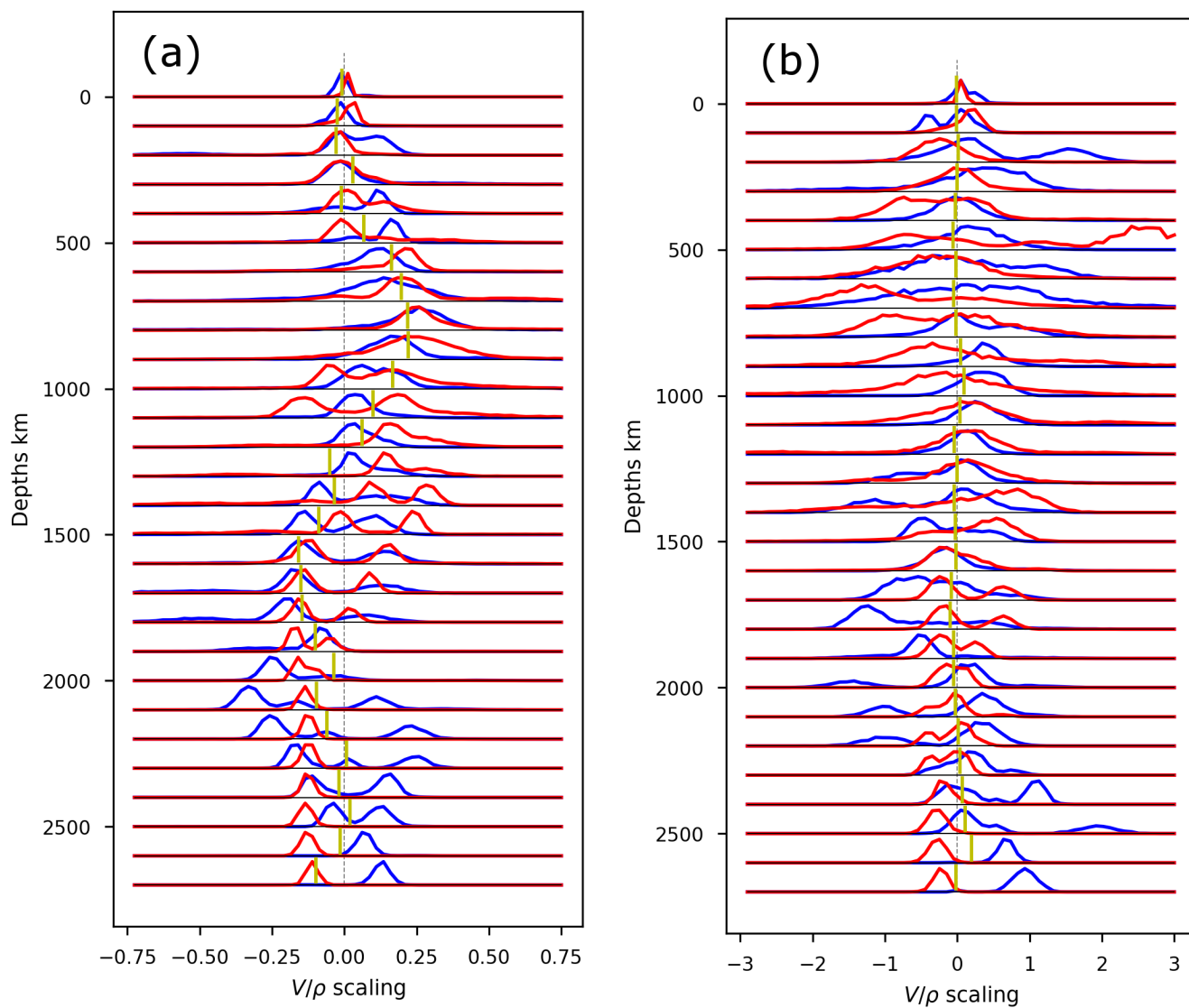
Figure 9. Distribution of density-velocity ratios as a function of depth. The blue is the distribution for fast velocity anomalies and the red is for slow velocity anomalies. The yellow line gives the median of the ratio distribution. Note that the median sometimes appears to lie outside the distribution, which is due to heavy tails that are not visible on this scale. Furthermore, the histograms for slow and fast anomalies are scaled to have the same maximum height for easier visual comparison. a) Scaling for results with isostatic residual. b) Scaling for results with crustal residuals.
