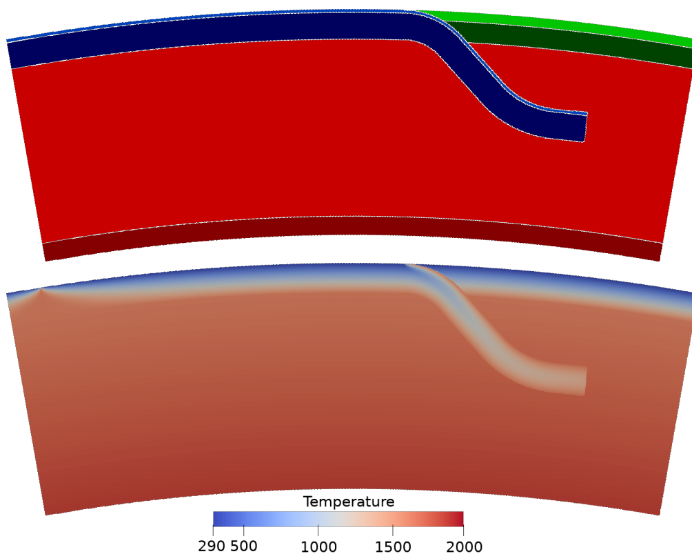
Figure 2. The same as setup as in figure 1, but now in spherical geometry. The top figure shows the composition, the bottom figure shows the temperature.
