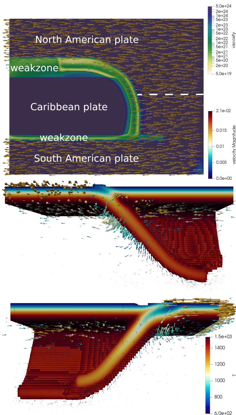
Figure 8. The 3D ASPECT Caribbean example after 2.5 million years of evolution. The top image is a top view of the model, where the top 50 km is removed, and where the viscosity field is shown with the velocity field indicated by the arrows. The bottom two figures are cut outs of the temperature field between 600 K and 1535 K, showing in colour the temperature (T) and with arrows the velocity fields, highlighting the velocity field in the slab and lithosphere.
