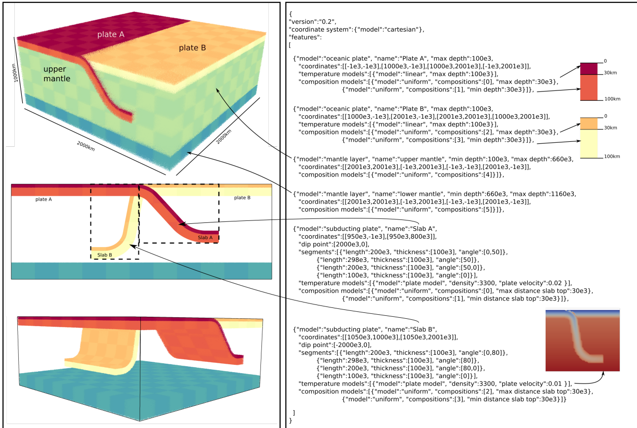
Figure E1. Connection between the GWB input file (right panel) and the resulting marker fields (left panel). Small upper inserts in the right panel show each plate layering while the bottom insert shows the temperature field zoomed in on slab B.
