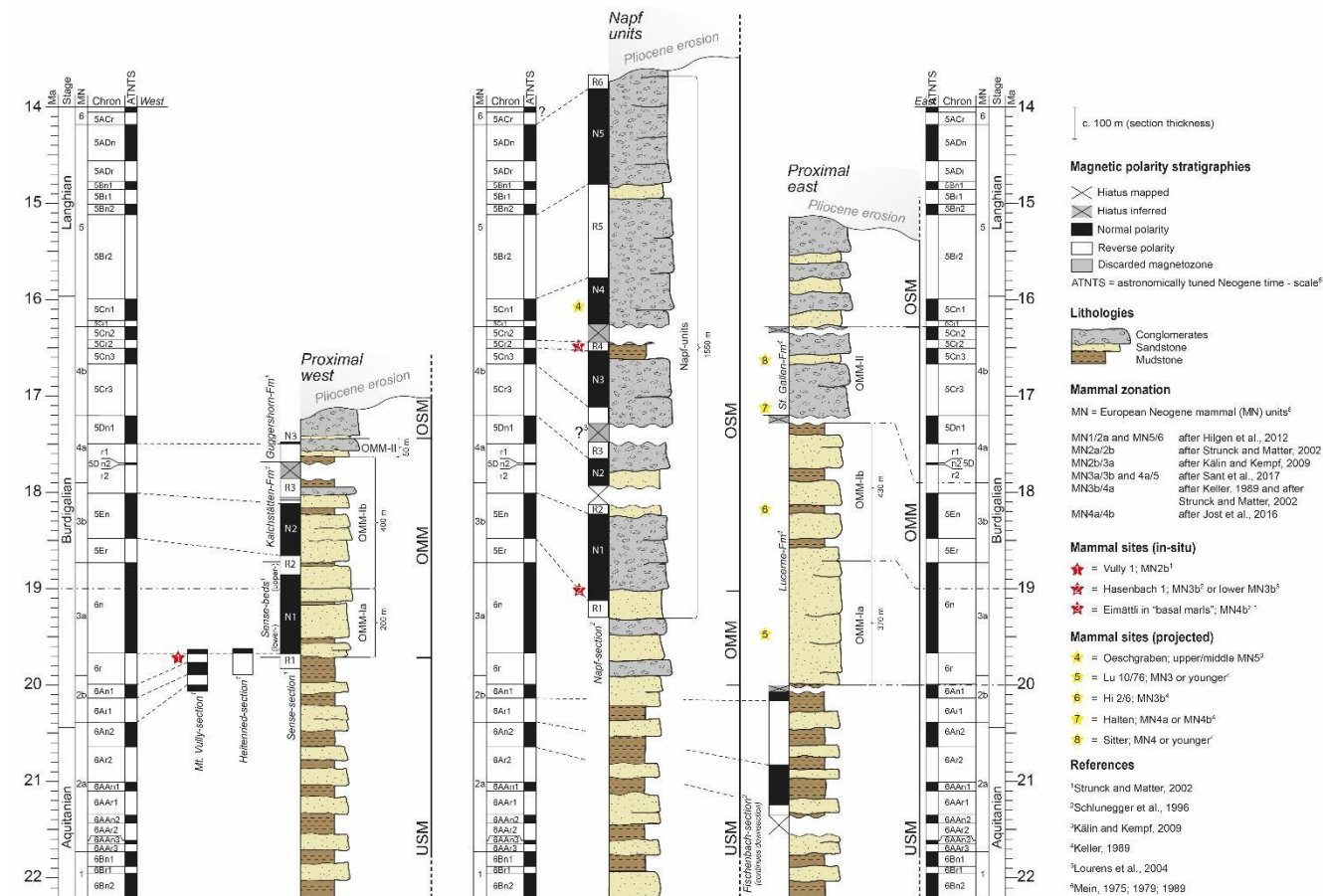
Figure 3: Composite stratigraphic columns illustrating the sedimentary architecture at the proximal basin border in the western Molasse basin (proximal west) in the central part of the Molasse basin (Napf units) and in the eastern basin (proximal east). A composite section for the proximal west has been drawn based on data from the Mt. Vully- and Heitenried-sections, drillings, and from surface information from the Sense-section (Sense beds and Kalchstätten-Fm) (Strunck and Matter, 2002). The composite section representative for the sequence at the Napf is mainly based on the sedimentary log by Schlunegger et al. (1996; see their Schwändigraben- and Fontannen-sections) complemented with information from the geological map of the region (Schlunegger et al., 2016). Please note that Kälin and Kempf (2009) proposed the occurrence of a very short hiatus recorded by magnetozone R3 within the Napf-units which we do not discuss in detail for simplicity purposes. The composite section illustrating the situation at the proximal basin border east of the Napf represents the sedimentary architecture as far east as of Lake Zurich (Fig. 2). It is based on data from Keller (1989, see his Rümli-, Ränggloch- and Lucerne-sections) and data from Schlunegger et al., (1996, see their Fischenbach-section) and geological maps of the region (Wolhusen; Isler and Murer, 2019). Please note that the Entlen-section is situated immediately east of the Napf (Fig. 4a) where the basal part (Lucerne-Fm) can be characterized by the composite section of the proximal east, while the topmost part is made up of the conglomerates of the Napf-units. Detailed sedimentological data of the Sense-beds and the Lucerne-Fm can be found in Fig. 5. Note, that the Molasse units written in capitals (i.e. USM, OMM and OSM) are based on the lithological architecture and thus on the facies associations identified in the field.
