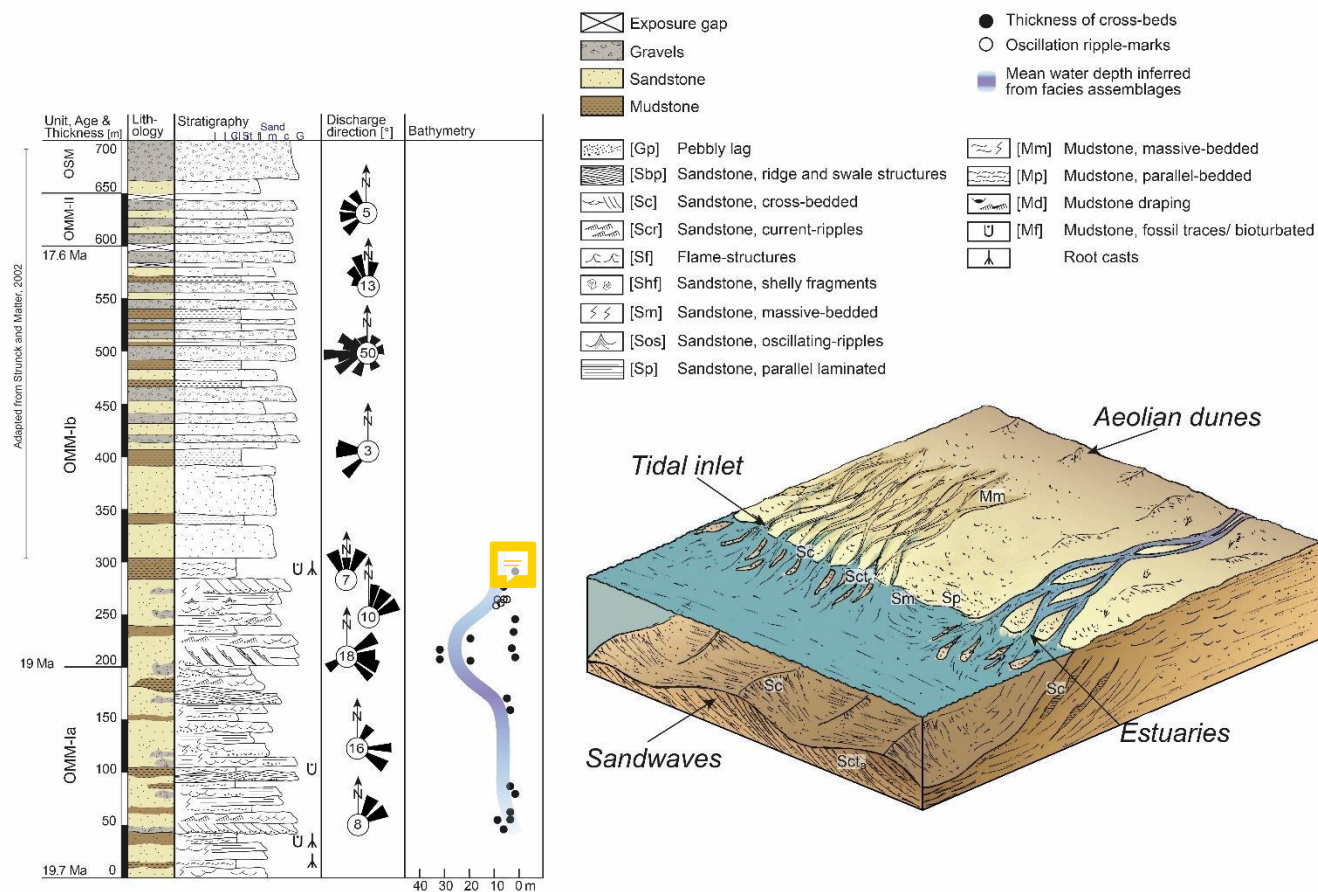
Figure 5 (a) and (b): Sedimentological log of the a) Entlen- and b) Sense-section. See Fig. 2 for location of sections, Fig. 4 for 5 chronological framework of the deposits and Table S1 (supplement) for further sedimentological details and abbreviations of the lithofacies. The block-diagrams illustrate the palaeo-geographical conditions from a conceptual point of view. Please note that the palaeo-bathymetry values are minimum estimates, and that the mean water depths have been inferred from the assignments of the lithofacies to the depositional environment. This might explain why the numerical values for water-depths based on cross-bed thicknesses and our inferred mean water-depth estimates deviate, in particular between c. 200 m and 250 m of the Sense-section.
