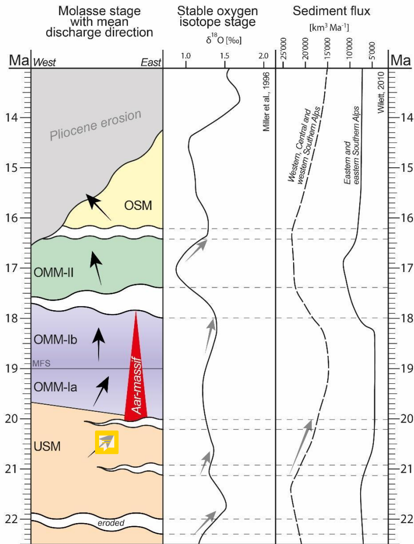
Figure 7: Molasse stages with mean discharge directions with hiatus plotted against stable oxygen isotope stages (Miller et al., 1996) and sediment flux (Willett, 2010). Red triangle marks the onset of delamination and fast exhumation of the Aar-massif (Herwegh et al., 2017). Grey arrows mark drops in sea level and sediment flux possibly contributing to the related hiatus.
