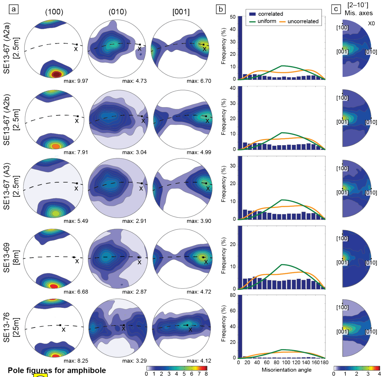
5 Figure 7. Pole figures illustrating amphibole CPO of the samples from the HTa unit in Sumeini massif. Samples are sorted using the distance from the peridotite, with increasing distance downwards. The dashed line represents the foliation and X points to the lineation. Contours are multiples of a uniform distribution. All plots are lower hemisphere projections. Numbers in square brackets refer to the distance to the peridotite; (b) Distribution of misorientation angles between correlated (adjacent) pixels (blue histogram) and between uncorrelated pixels (orange curve) of amphibole. The uniform (green) curve corresponds to the theoretical misorientation distribution for a perfectly randomly oriented crystals; (c) Amphibole inverse pole figures showing the distribution of correlated misorientation axes (between 2° and 10°). Contours are multiples of uniform distribution.
