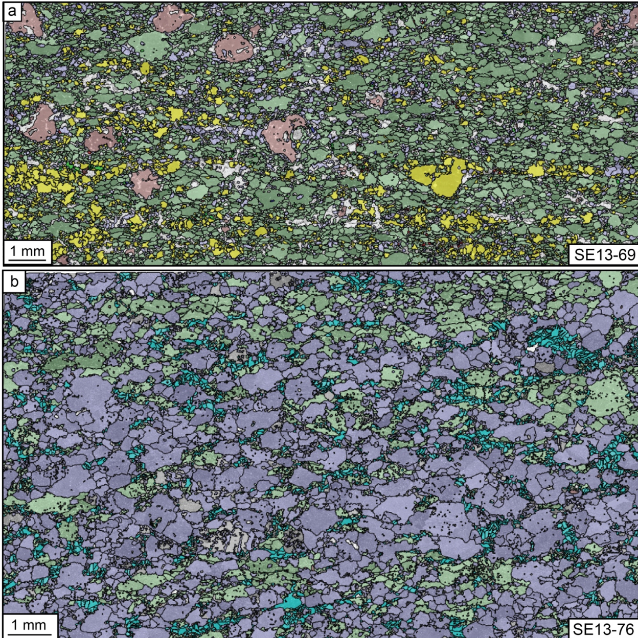
Figure 4: EBSD phase maps (a) from a slightly retrogressed at amphibolite facies garnet-clinopyroxene-bearing amphibolite at the top of HTa unit (sample SE13-69; Sumeini area) (b) from a highly retrogressed garnet-clinopyroxene-free amphibolite at the base of HTa unit (sample SE13-76; Sumeini area).
