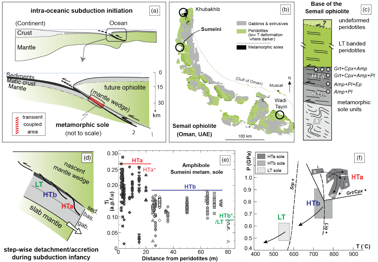
Figure 1: (a) Geodynamic setting of metamorphic sole formation during intra-oceanic subduction infancy; (b) Simplified geological map of the Semail ophiolite, highlighting the outcrops of metamorphic sole beneath the ophiolite mantle (modified after Nicolas et al., 2000); (c) schematic log of the base of the Oman ophiolite showing the structural position of the samples from Khubakhib (K), Sumeini (S) and Wadi Tayin (WT). See Table 1 for details; (d) Close-up view on the tectonic configuration along the nascent plate interface, during the formation and exhumation of the HTa, HTb and LT soles until reaching the steady state (sketch modified after Agard et al., 2016 and Soret et al., 2017). s: sediment, b: basalt, g: gabbro, m: mantle peridotite (e) Amphibole Ti/Si content in amphibolite samples from Sumeini (after Soret et al., 2017) outlining the discontinuous decrease of T conditions during the exhumation of the HT metamorphic sole; (f) Compilations of P-T estimates and associated P-T paths (after Soret et al., 2017), from the Grt-Cpx amphibolite (HTa), to the Pl-rich amphibolite (HTb) and greenschist facies (LT) metamorphic sole units.
