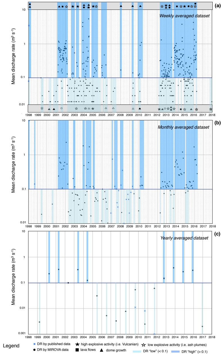
Figure 2. Dataset about the averaged discharge rates of Fuego de Colima during 1998-2018, derived by the MIROVA thermal data (black points) and published data (blue crosses) (Navarro-Ochoa et al. (2002); Zobin et al. (2005); Reubi et al. (2013); Mueller et al. (2013); Varley (2015); Reyes-Dávila et al. (2016); Thiele et al. (2017); GVP (2002, 2017)). Values > 0.1 (m^3 s^{-1}) are considered to be as “high” (dark blue area) and values < 0.1 (m^3 s^{-1}) as “low” discharge rate (light blue area). The 0.01 (m^3 s^{-1}) is the threshold under which the MIROVA system does not provide reliable data (blue line); (a) Weekly average discharge rates. The boxes contain symbols of volcanological observations reported in literature; (b) Monthly average discharge rates; (c) Yearly average discharge rates.
