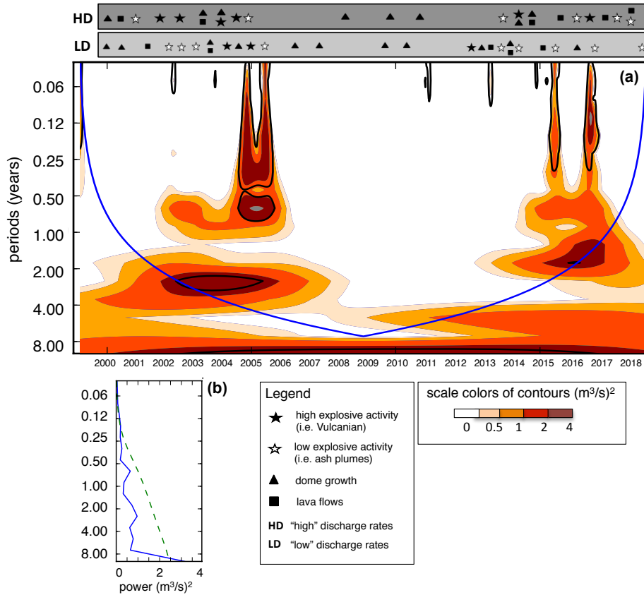
Figure 3. (a) Local wavelet spectrum normalized by 1/(\sigma)^2 ( (\sigma)^2 in (m^3 s^{-1})^2 ). The left axis is the period (in years). The bottom axis is time (in years). The shaded contours are at normalized variances of 0.5, 1, 2, and 4 (m^3 s^{-1})^2 . The black thick contour encloses regions of greater than 95% confidence for a red-noise process with a lag-1 coefficient of 0.72. It shows three orders of periodicities of: long-term (ca. 1.5-2.5 years), intermediate-term (ca. 5-10 months) during 2002-2006 and 2013-2016, and short-term (ca. 2.5-5 weeks) during 2001-2006 and 2011-2016. Blue line indicates the “cone of influence” where edge effects become important outside it; (b) Global wavelet power spectrum. The green dotted line represents the best-fitting red noise spectrum at 95% confidence level.
