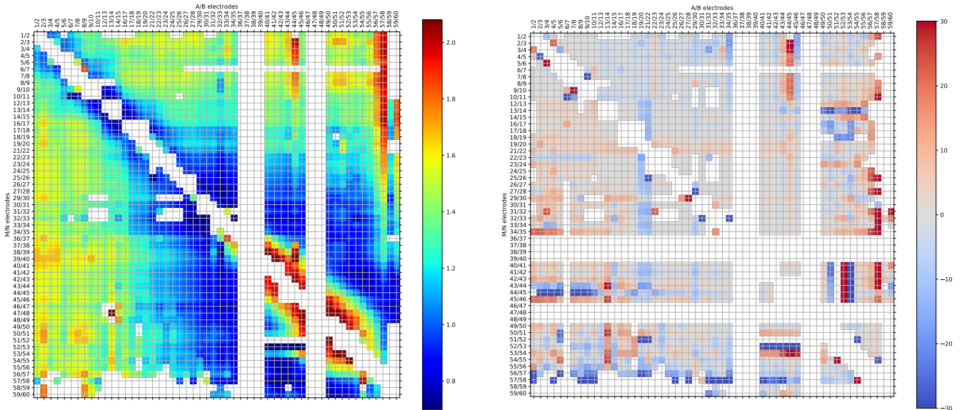
Figure 4. Raw data (all retrieved AB-MN pairs) as a function of current AB and potential MN dipoles. Left: Apparent resistivity ( \log \rho_a [ \Omega\text{m} ]), Right: Relative reciprocal error between forward (starting with current dipole 1/2) and reverse measurements (%).
