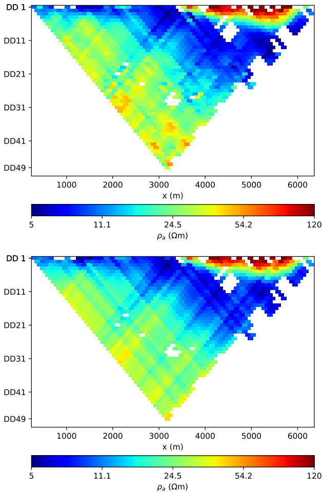
Figure 5. Unified data set as apparent resistivity pseudo-section: measured data (top) and model forward response (bottom).
