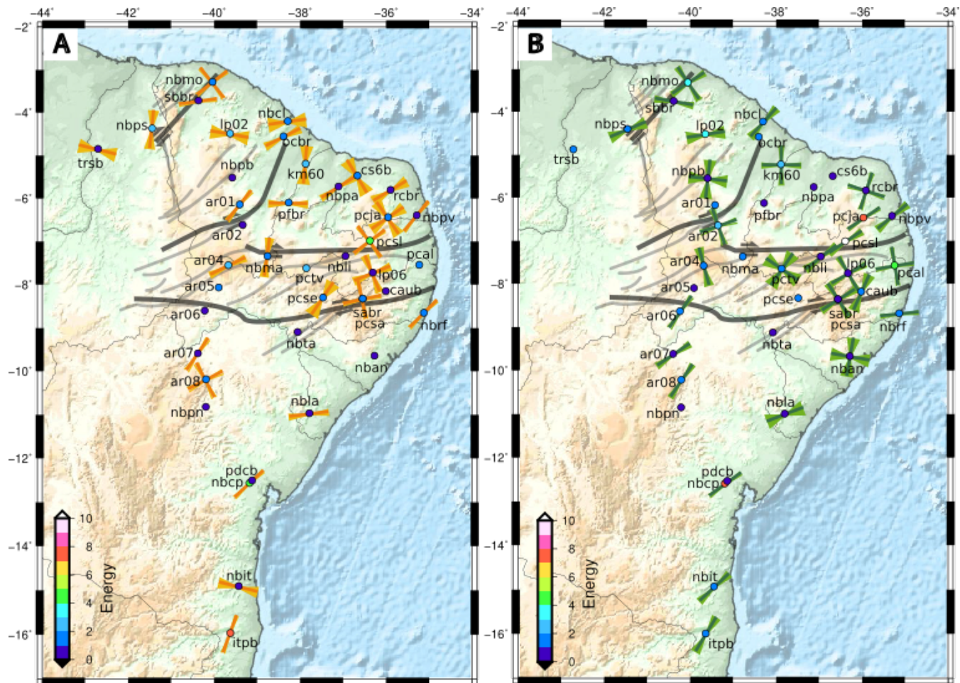
Figure 6. A) Map of symmetry directions (dark lines) obtained for the crust (0-32 km). When one line is plotted at the station, it represents either the trend of the dip in the case of dipping interface or the trend of the fast axis in the case of plunging anisotropy. When two lines are plotted, they refer to the fast axis and to its perpendicular direction in the case of horizontal anisotropy. Light colors represent 2\sigma uncertainties estimated from the bootstrap (after re-sampling 200 times). B) Same for the lithospheric mantle (32-100 km). Station symbols have been color-coded according to the energy level of the dominant harmonic degree.
