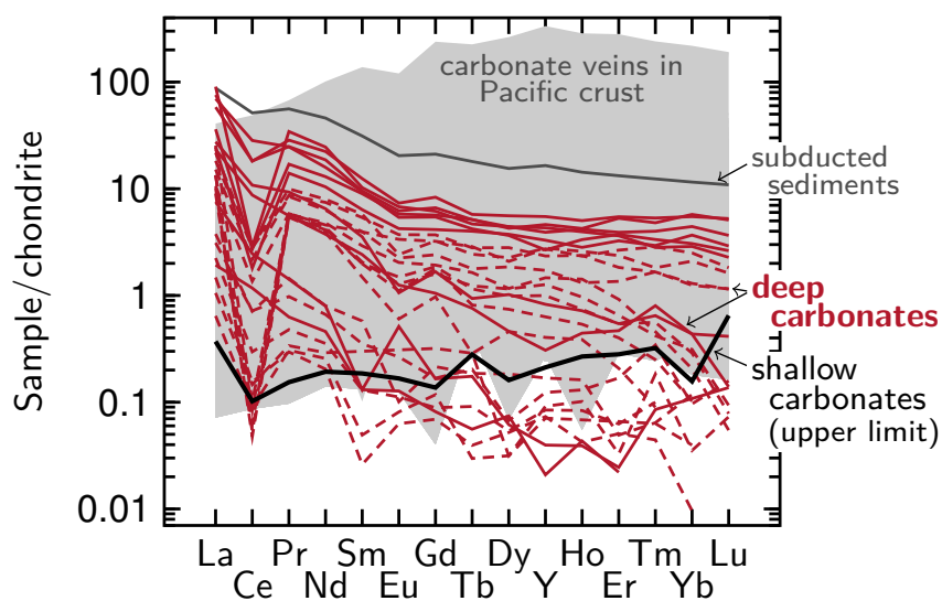
Figure 4: REE+Y compositions of vein carbonates normalized for chondrite (McDonough and Sun, 1995). Carbonates formed from deep fluids (red lines) are enriched in REEs and exhibit negative Ce anomalies. They are hosted by metavolcanic clasts and a quartzite breccia. Samples are from Fantangisña (dashed lines) and Asùt Tesoru (solid lines). Carbonates formed close to the seafloor have low REE contents (the black line marks the upper limit of REE contents across all authigenic carbonates and carbonates within serpentinite clasts) and likely precipitated from mixed venting fluid and seawater. These carbonates are hosted by serpentinite and one metavolcanic clasts, and also include carbonates that grew in the mud matrix. For comparison, REE data of carbonate veins in the basaltic Pacific crust (ODP Sites 801 and 1149; Rausch, 2012) and of subducting sediments (ODP Sites 800 and 801; Plank and Langmuir, 1998) are shown.
