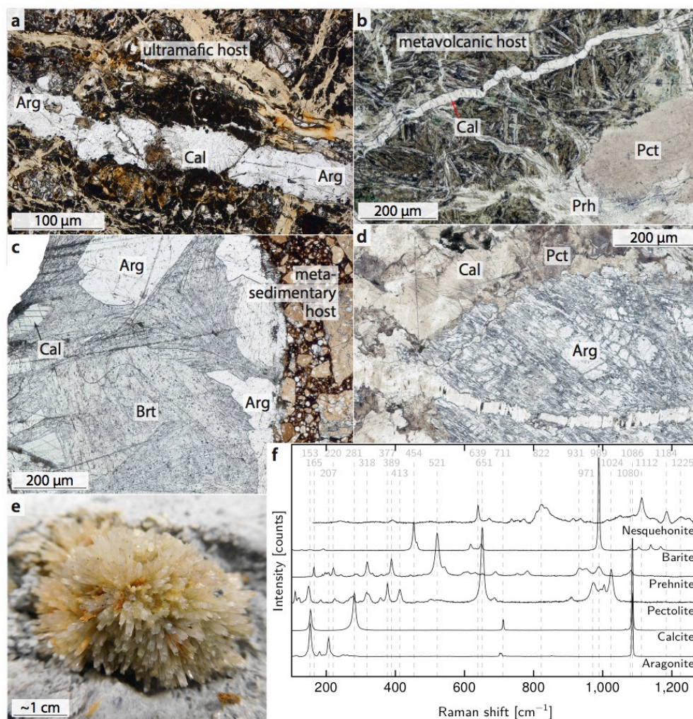
5 Figure 3: Thin section scans and photomicrographs depicting vein assemblages. (a) Late-stage calcite–aragonite vein in partially serpentinized ultramafic clast (sample U1491B-5H-CC, 1–3 cm). (b) Narrow late-stage calcite vein in metavolcanic host rock (sample U1498B-8R-1, 32–34 cm). (c) Wide barite–aragonite–calcite vein in a brecciated quartzite clast (sample U1497A-7X-CC, 29–31 cm). Euhedral crystal shapes imply a strain-free environment and chemical equilibrium during precipitation. (d) Wide vein inside metavolcanic clast with complex intergrowth of pectolite and microcrystalline calcite overgrowing earlier aragonite (sample U1498B-8R-1, 10–15 cm). (e) Authigenic aragonite with acicular growth within serpentinite mudflow (sample U1492B-1H-3, 16–18 cm). (f) Raman spectra of the most common carbonate, silicate, and sulfate vein assemblages. Abbreviations: Arg, aragonite; Brt, barite; Cal, calcite; Pct, pectolite; Prh, prehnite.
