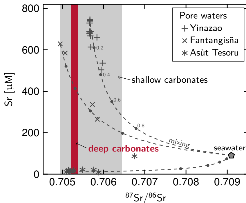
5 Figure 5: Strontium geochemistry of carbonates and serpentinite mud pore waters. Slab-derived fluids are more unradiogenic than seawater. Mixing of slab-derived fluids with seawater is indicated by sample plotting on the mixing lines; it usually occurs towards the core tops ( cf. Table S2). Strontium isotopic values of deep carbonates well resemble those of slab-derived fluids, implying that they precipitated from these fluids at depth. Shallow carbonates exhibit a wider range of Sr isotopic compositions. They likely formed in the mixing zone of upwelling fluids and seawater. Note that even large amounts of seawater admixed into slab-derived fluids do not necessarily alter the Sr isotopic composition strongly (numbers along dashed mixing lines indicate fraction of seawater). Bottom seawater composition from Mottl et al. (2004).
